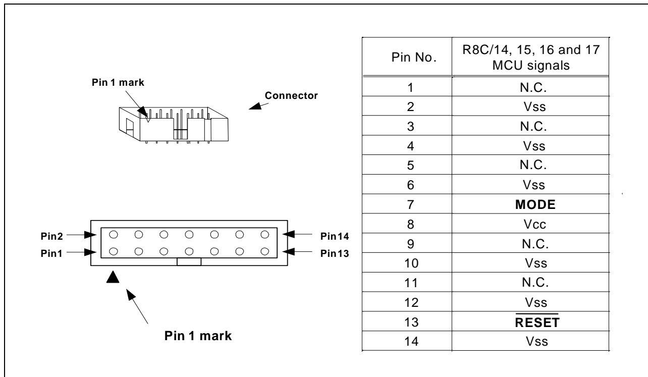
Figure 4.1 E8a Connecting Connector Pin Assignments
