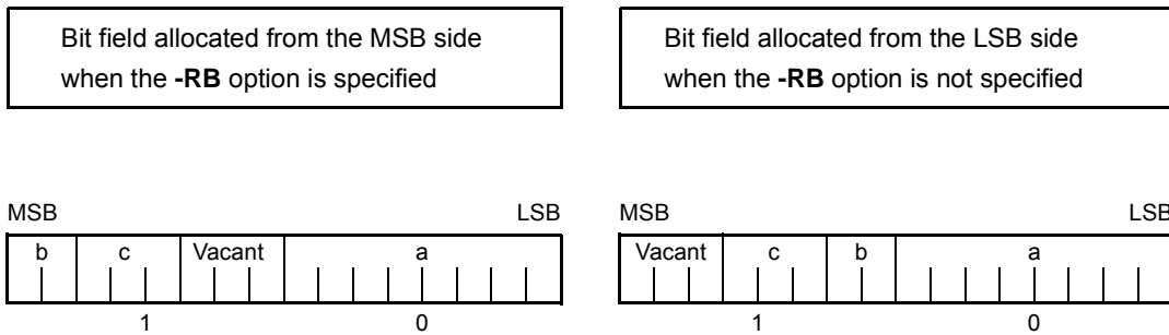
Figure 11-4 Bit Allocation by Bit Field Declaration (Example 2)
