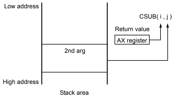
Figure 12-4 Placing Arguments on Stack
