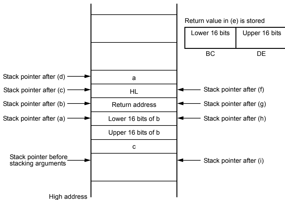
Figure 10-1 Stack Area When Function Is Called (No -ZR Specified)
