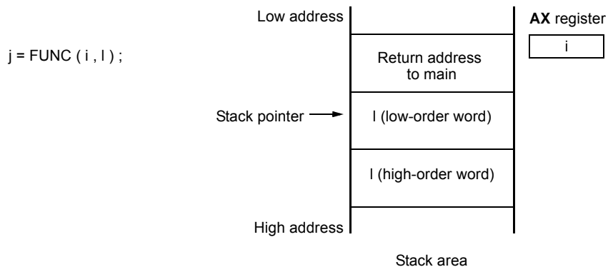
Figure 12-6 Stack Positions of Arguments
