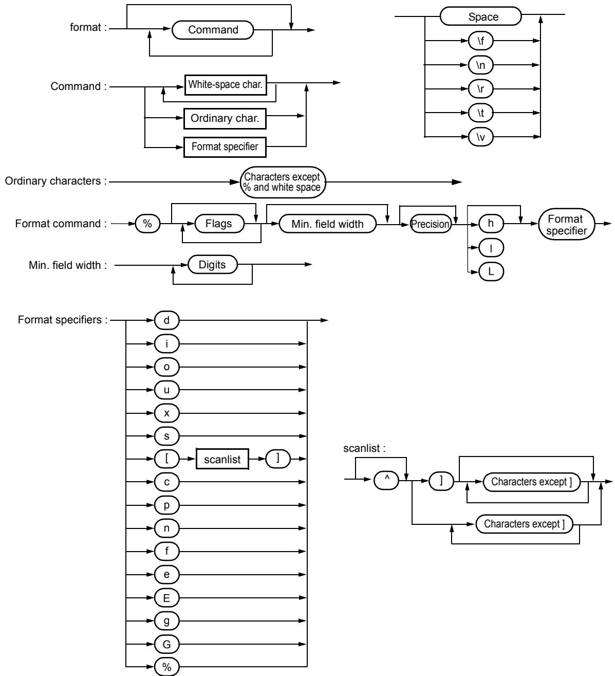
Figure 10-3 Syntax of Input Format Commands
