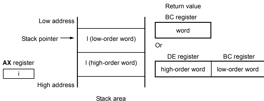
Figure 12-3 Stack Area After Returning
