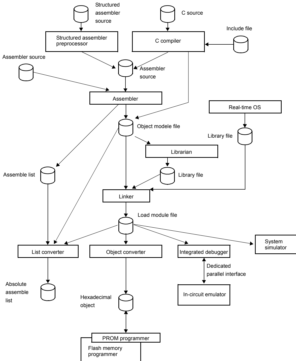
Figure 1-2 Program Development Procedure by This C Compiler
