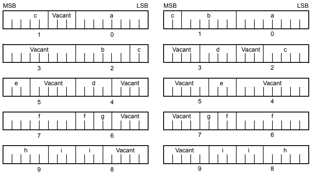
Figure 11-7 Bit Allocation by Bit Field Declaration (Example 3) (with -RC Option Specified)
