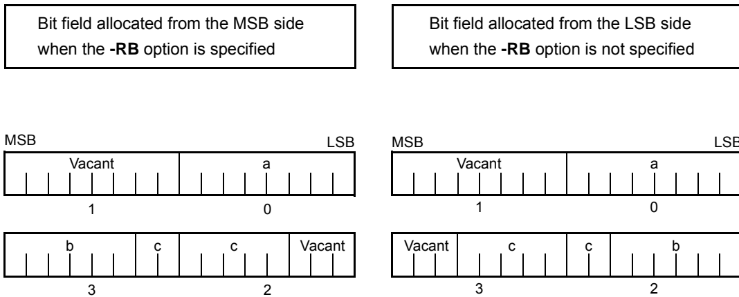
Figure 11-6 Bit Allocation by Bit Field Declaration (Example 3)
