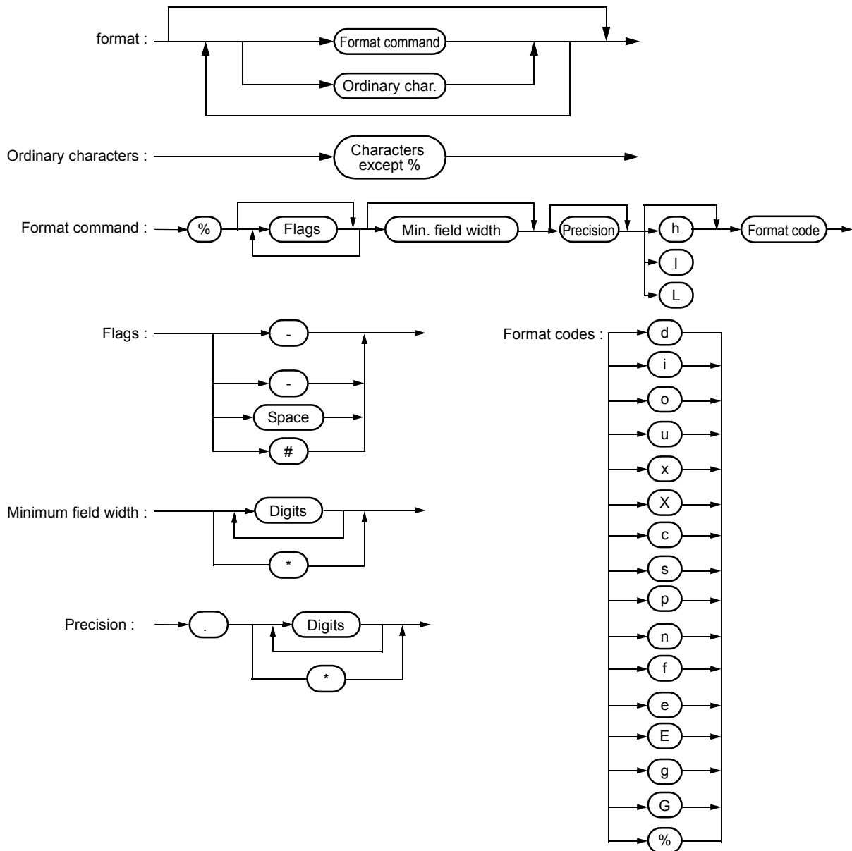
Figure 10-2 Syntax of Format Commands
