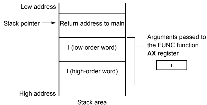
Figure 12-1 Stack Area After a Call
