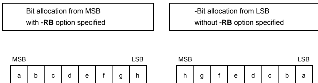
Figure 11-3 Bit Allocation by Bit Field Declaration (Example 1)
