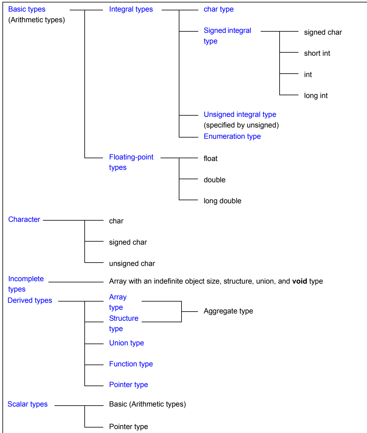
Figure 2-1 Classification of Types
