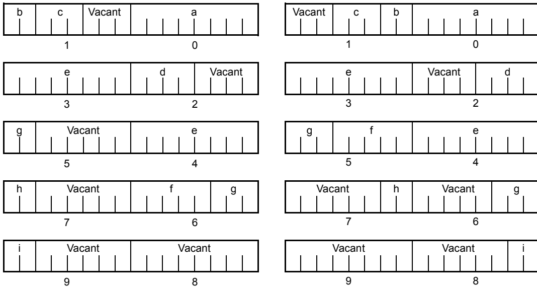
Figure 11-5 Bit Allocation by Bit Field Declaration (Example 2) (with -RC Option Specified)
