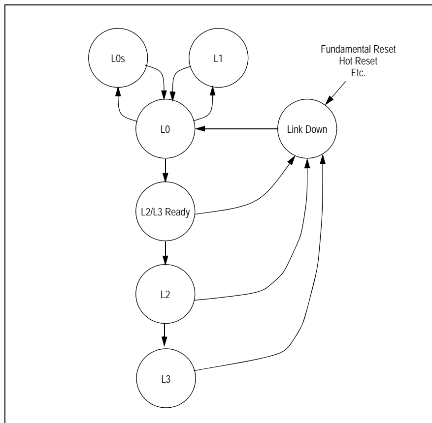
Figure 4.3 PES8T5A ASPM Link State Transitions
