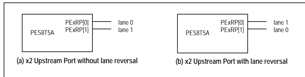
Figure 4.2 Upstream Port (x2 Lane Width) Lane Reversal
