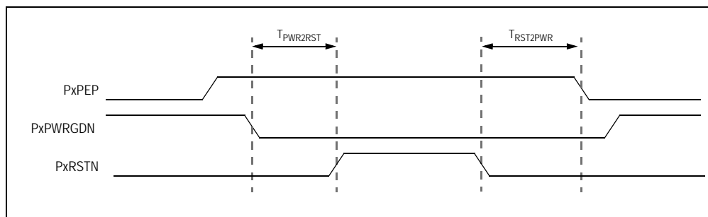
Figure 2.7 Power Good Controlled Reset Output Mode Operation
