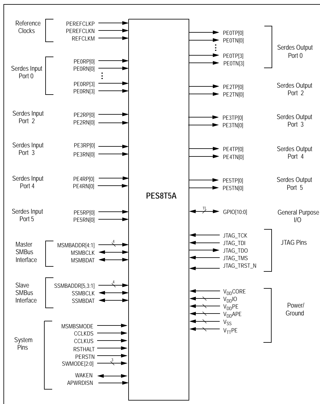
Figure 1.2 PES8T5A Logic Diagram
