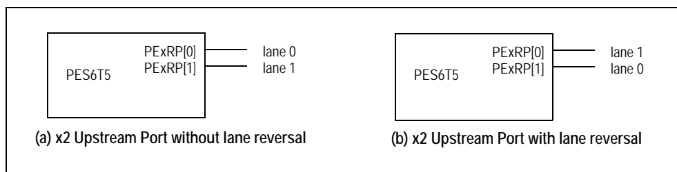
Figure 4.1 Upstream Port (x2 Lane Width) Lane Reversal
