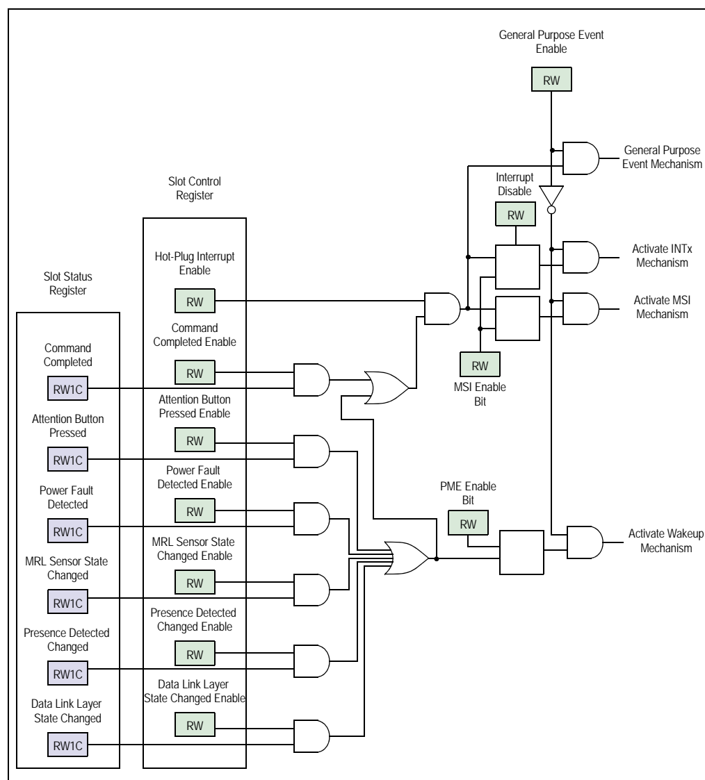
Figure 8.4 PES6T5 Hot-Plug Event Signalling
