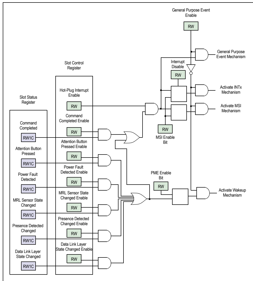
Figure 10.6 PES48H12AG2 Hot-Plug Event Signalling
