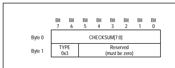
Figure 6.3 Configuration Done Sequence Format
