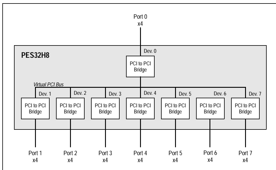
Figure 1.3 All Ports Unmerged Configuration
