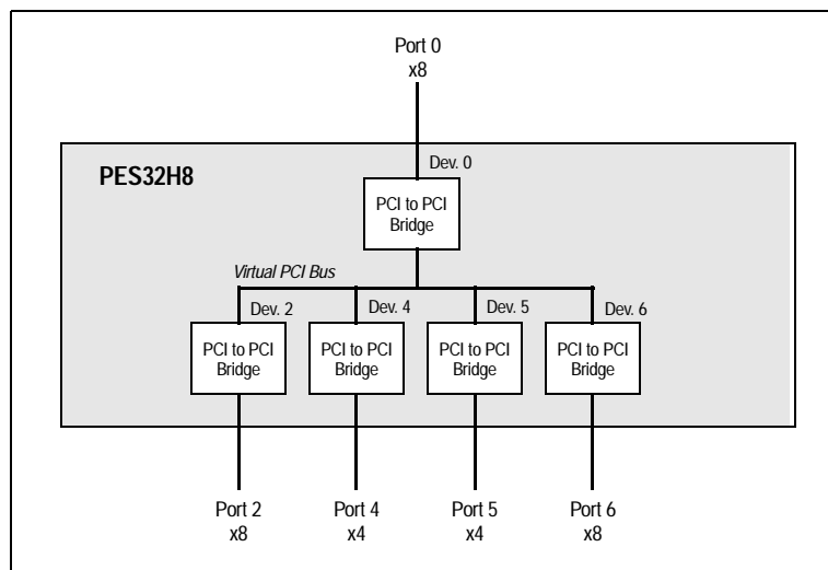
Figure 1.4 Some Ports Merged Configuration
