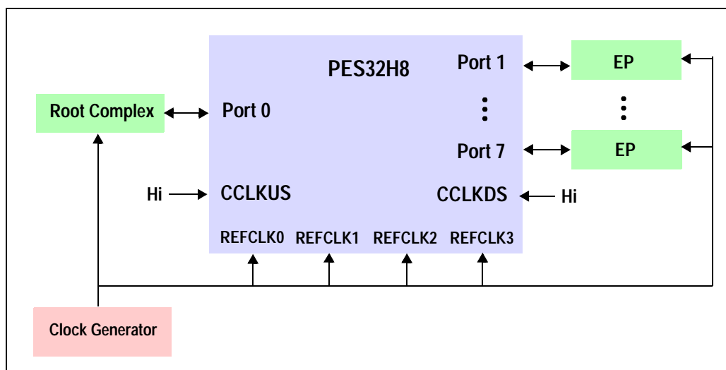
Figure 3.1 Common Clock on Upstream and Downstream (option to enable or disable Spread Spectrum Clock)
