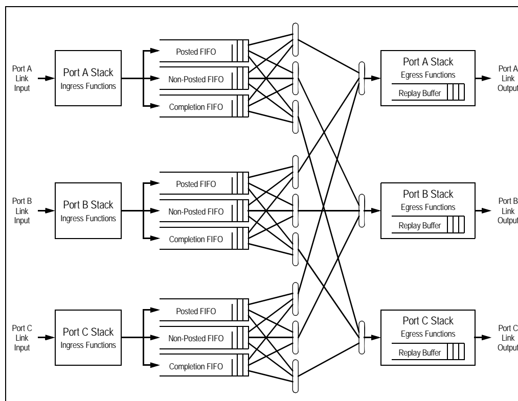
Figure 4.1 PES24N3 Switch Data Flow and Buffering
