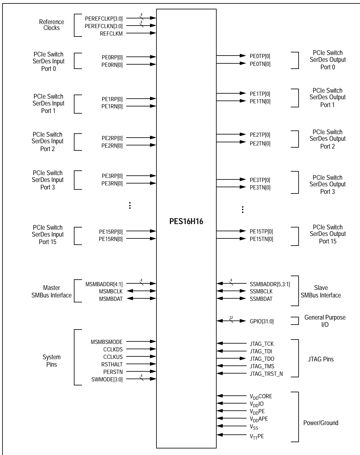
Figure 1.2 PES16H16 Logic Diagram
