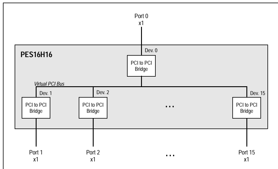
Figure 1.3 Port Configuration
