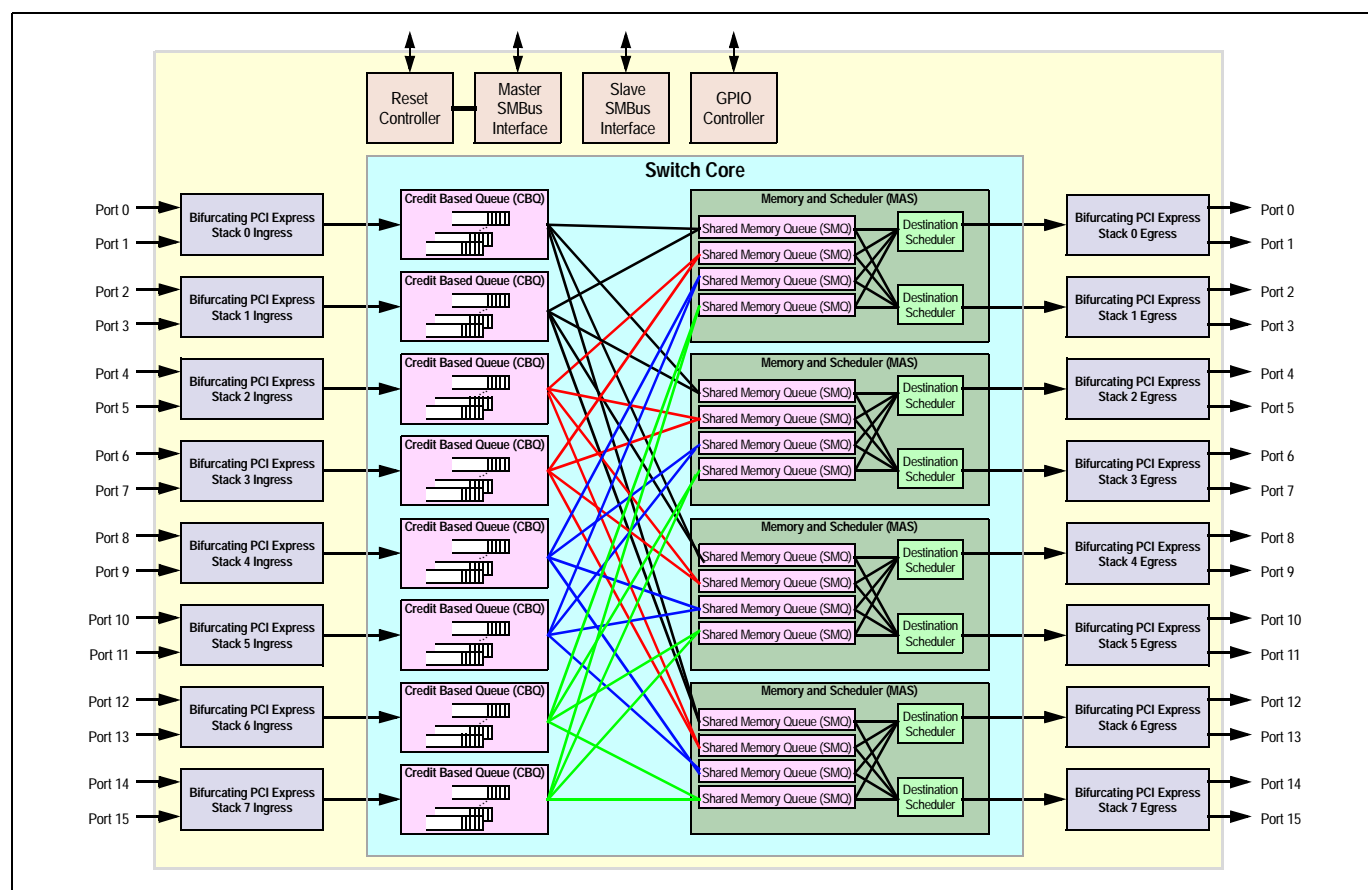
Figure 1.1 PES16H16 Architectural Block Diagram
