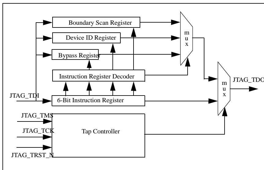
Figure 10.1 Diagram of the JTAG Logic
