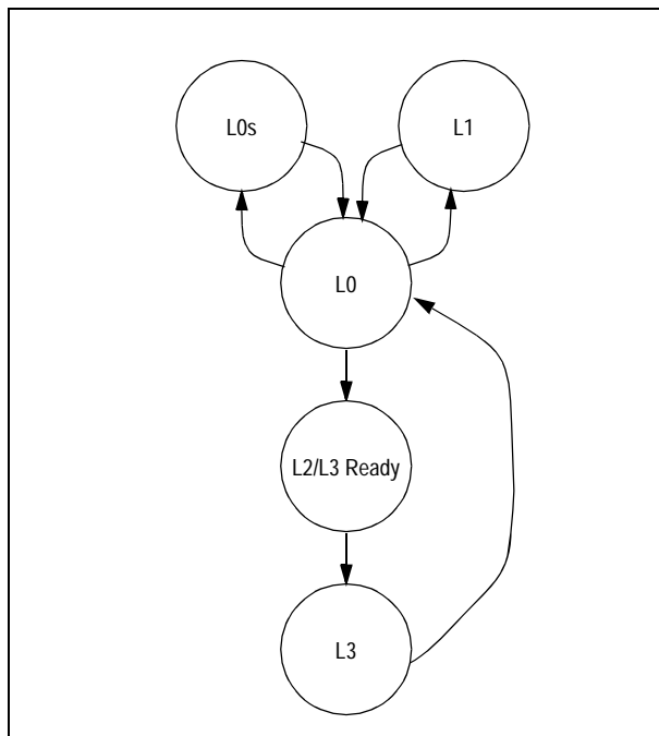
Figure 4.1 PES16H16 ASPM Link State Transitions
