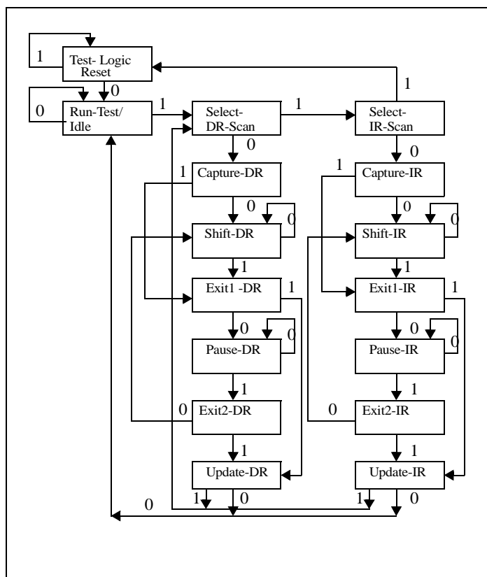
Figure 10.2 State Diagram of PES16H16's TAP Controller
