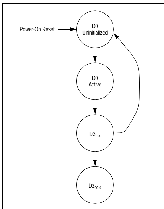
Figure 7.1 PES16H16 Power Management State Transition Diagram
