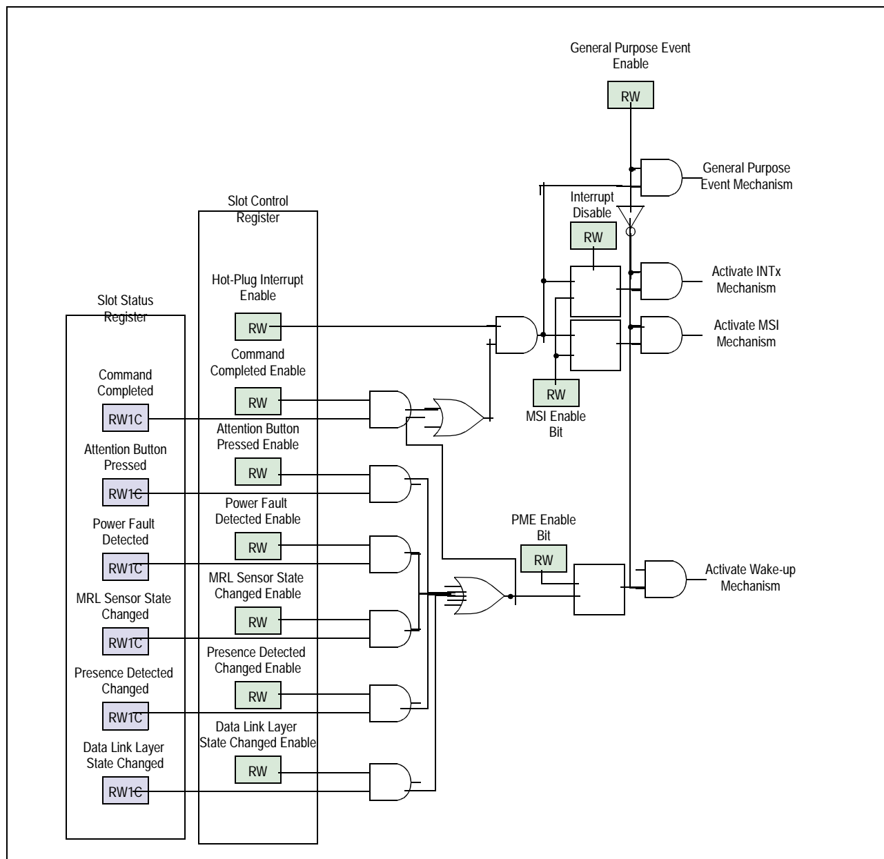
Figure 8.4 PES16H16 Hot-Plug Event Signalling
