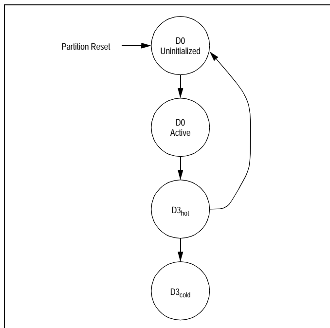
Figure 9.1 PES32NT8xG2 Power Management State Transition Diagram
