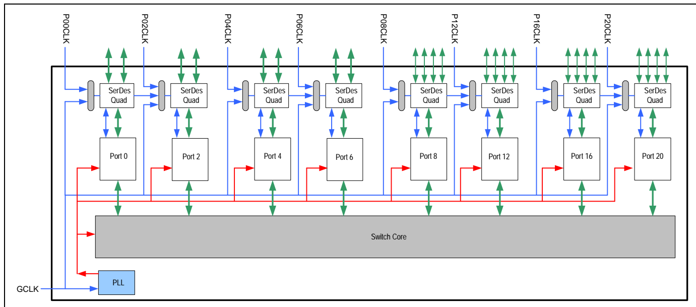
Figure 2.1 Logical Representation of PES32NT8AG2 Clocking Architecture
