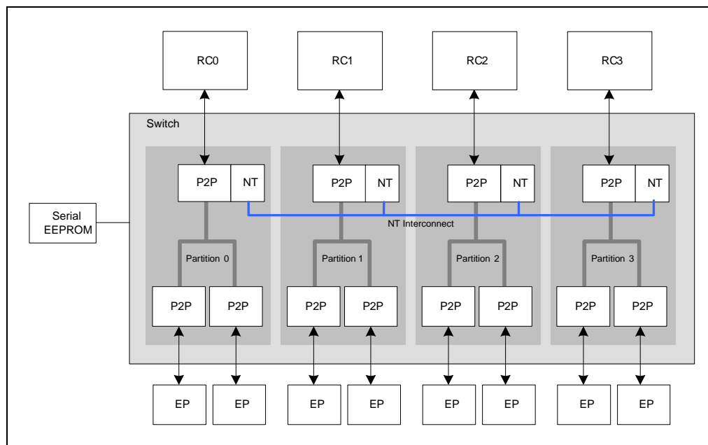
Figure 26.7 Multiprocessor System Interconnection Using the PES32NT8xG2
