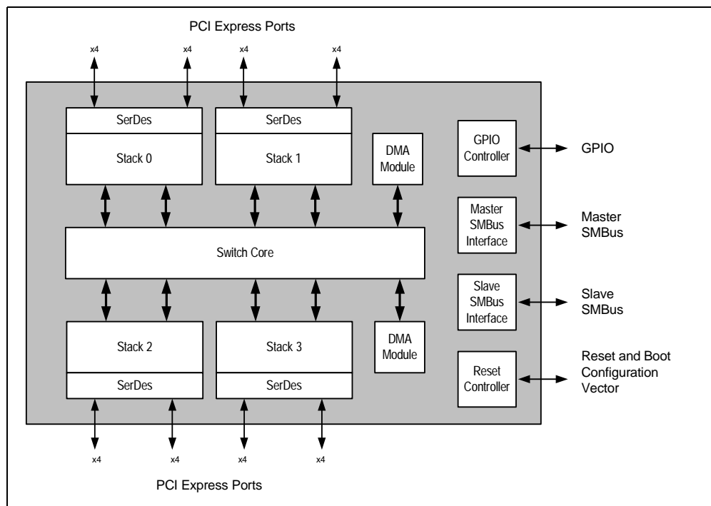
Figure 1.1 PES32NT8xG2 Block Diagram
