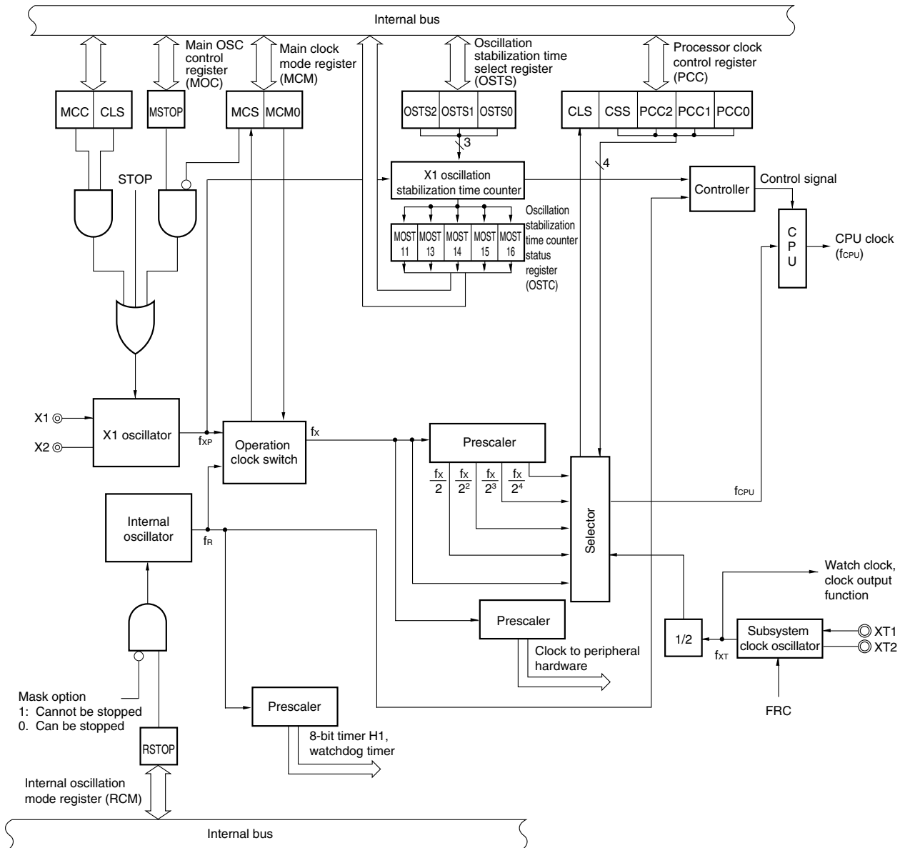
Figure 5-1. Block Diagram of Clock Generator
