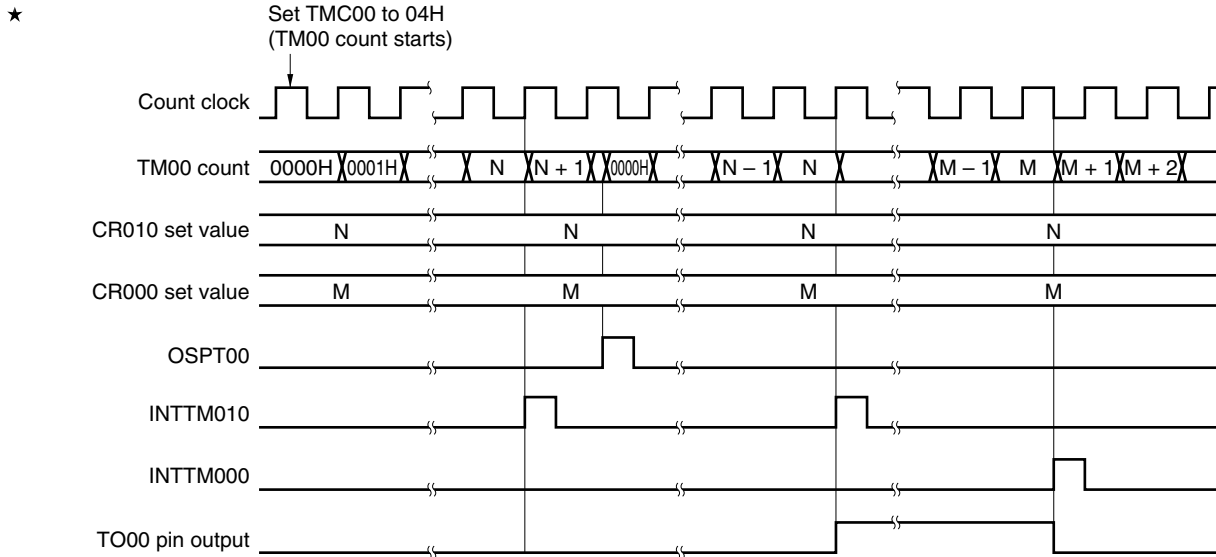
Figure 6-32. Timing of One-Shot Pulse Output Operation with Software Trigger
