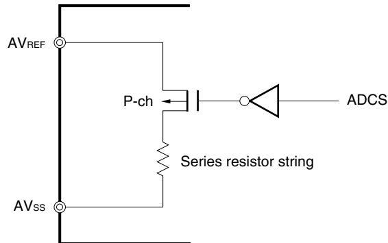
Figure 12-2. Circuit Configuration of Series Resistor String
