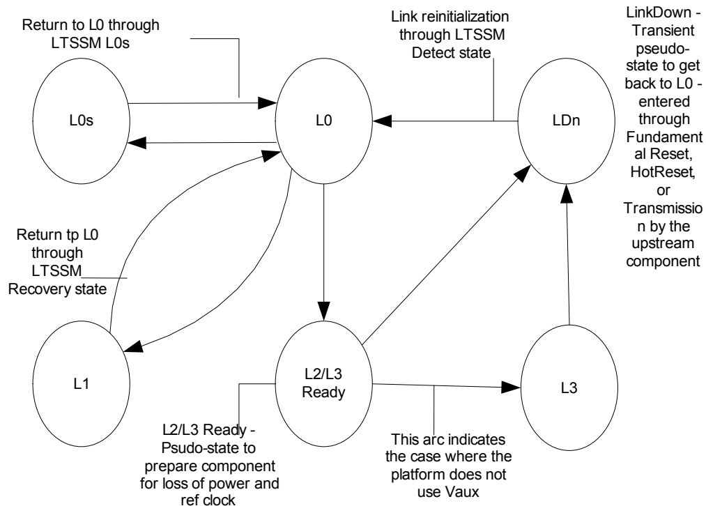
Figure 26: PCIe Link Power Management States
