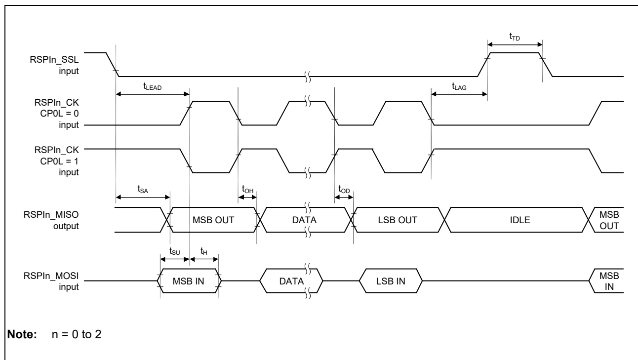
Figure 48.53 Transmission and Reception Timing (Slave, CPHA = 0)
