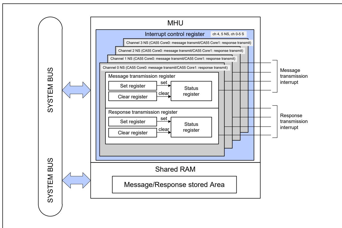
Figure 12.2 Hardware configuration
