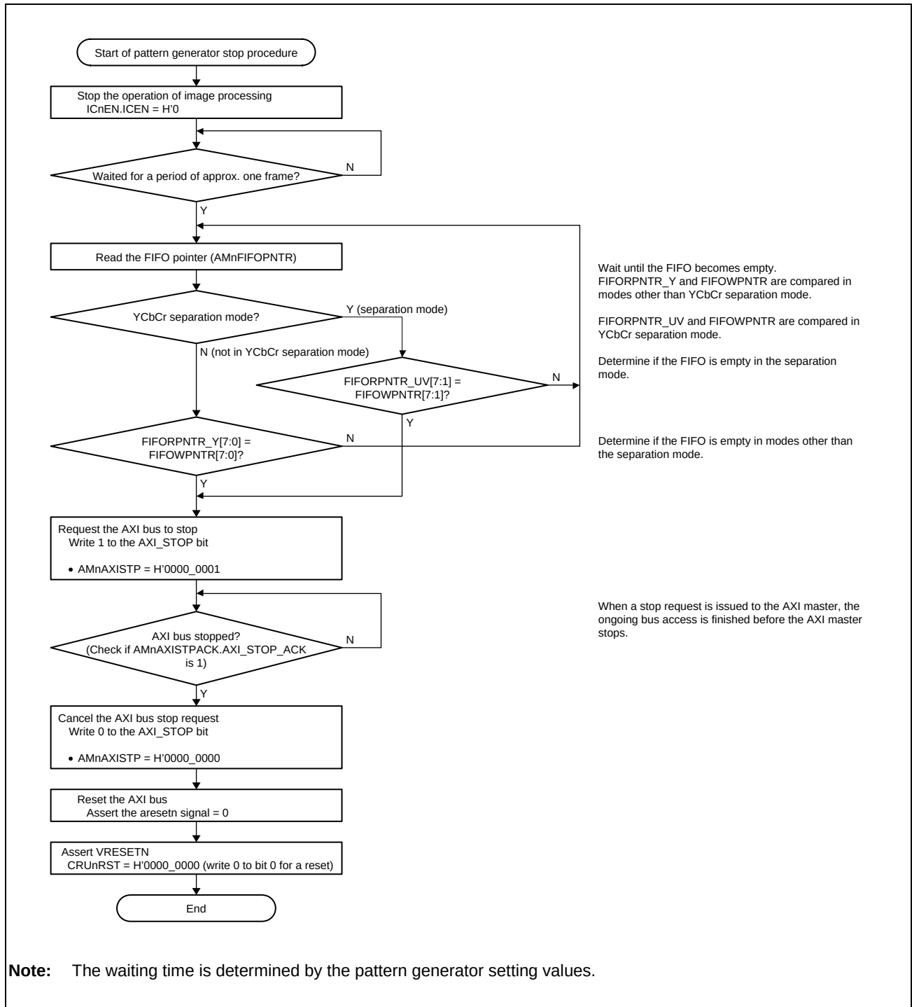
Figure 35.64 Flow for Stopping the Pattern Generator
