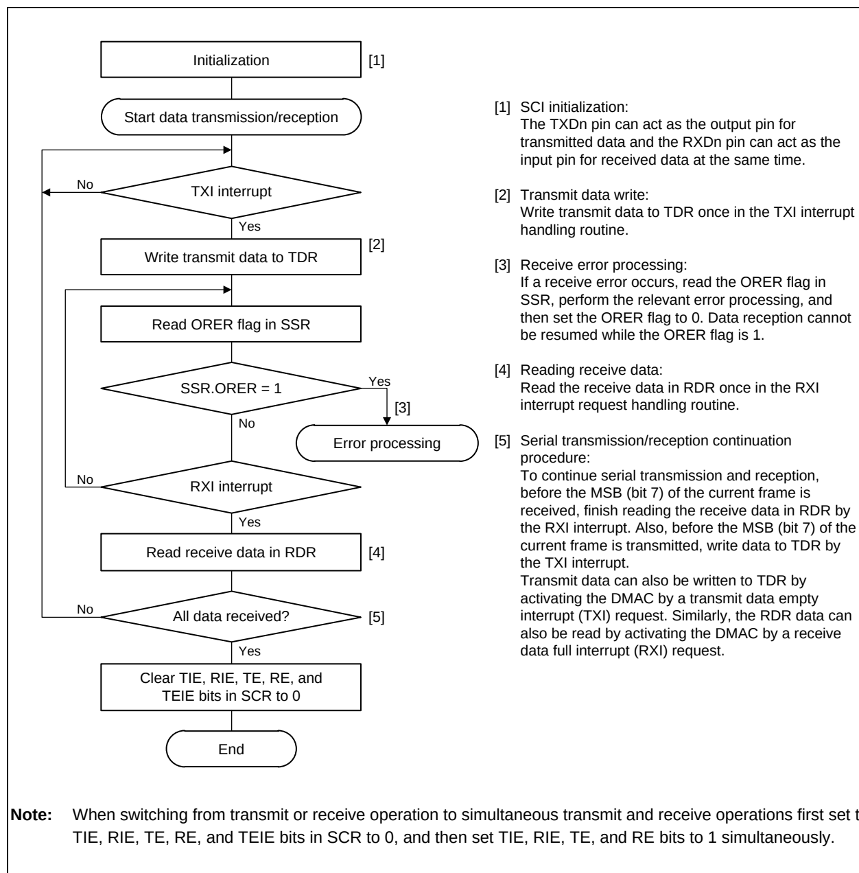
Figure 23.28 Example Flowchart of Simultaneous Serial Transmission and Reception in Clock Synchronous Mode
