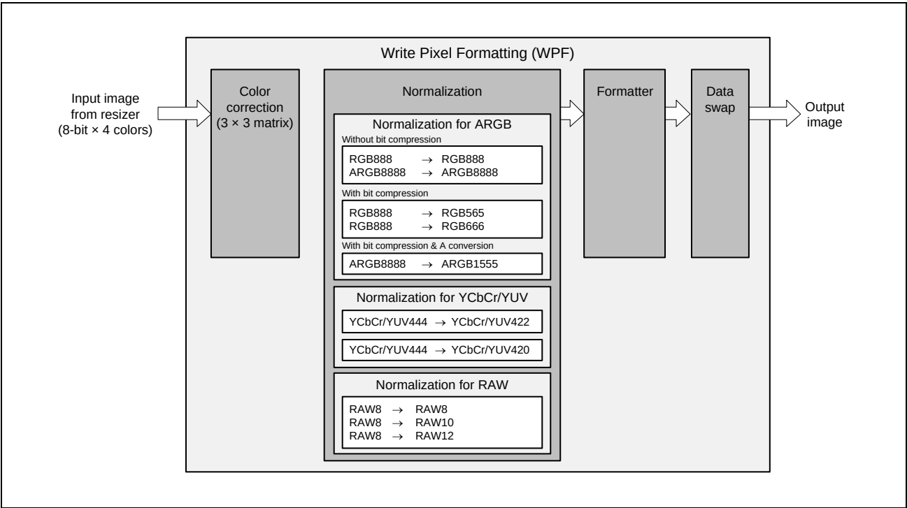
Figure 36.28 WPF Block Diagram
