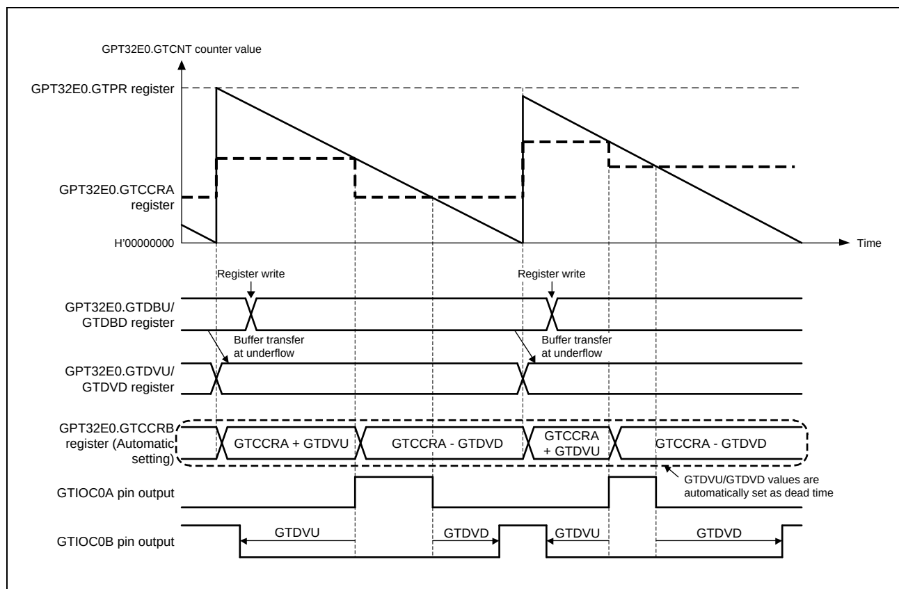
Figure 18.43 Example of automatic dead time setting function operation with saw-wave one-shot pulse mode, down-counting, GTDVU and GTDVD set to buffer operation, and active-high
