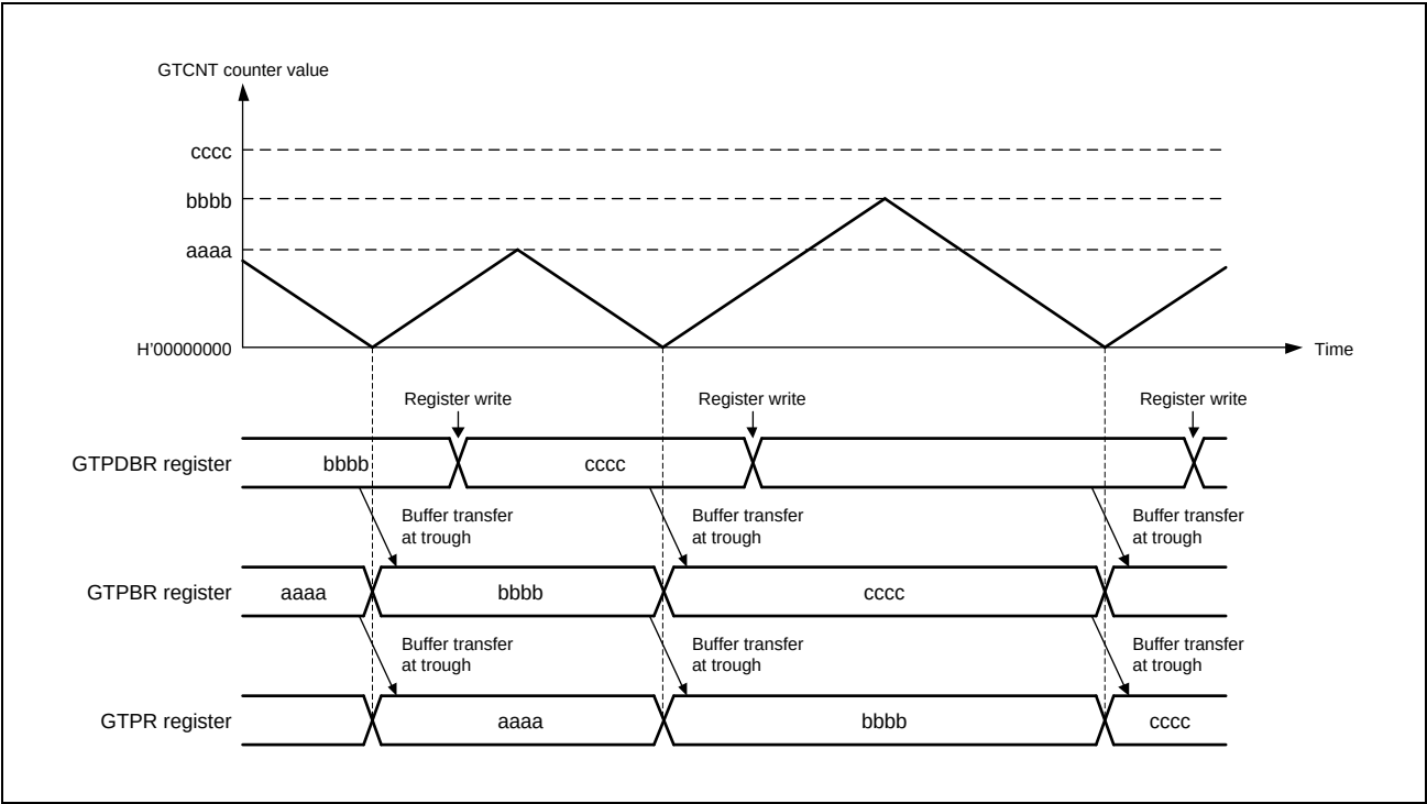
Figure 18.19 Example of GTPR double buffer operation with triangle waves
