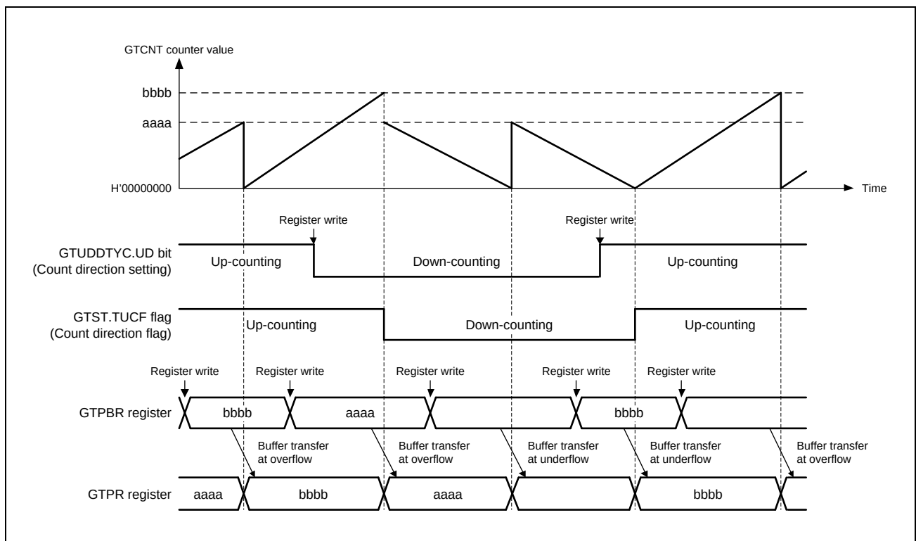
Figure 18.48 Example of count direction changing function operation during buffer operation
