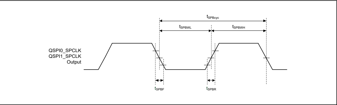
Figure 48.26 Clock Timing
