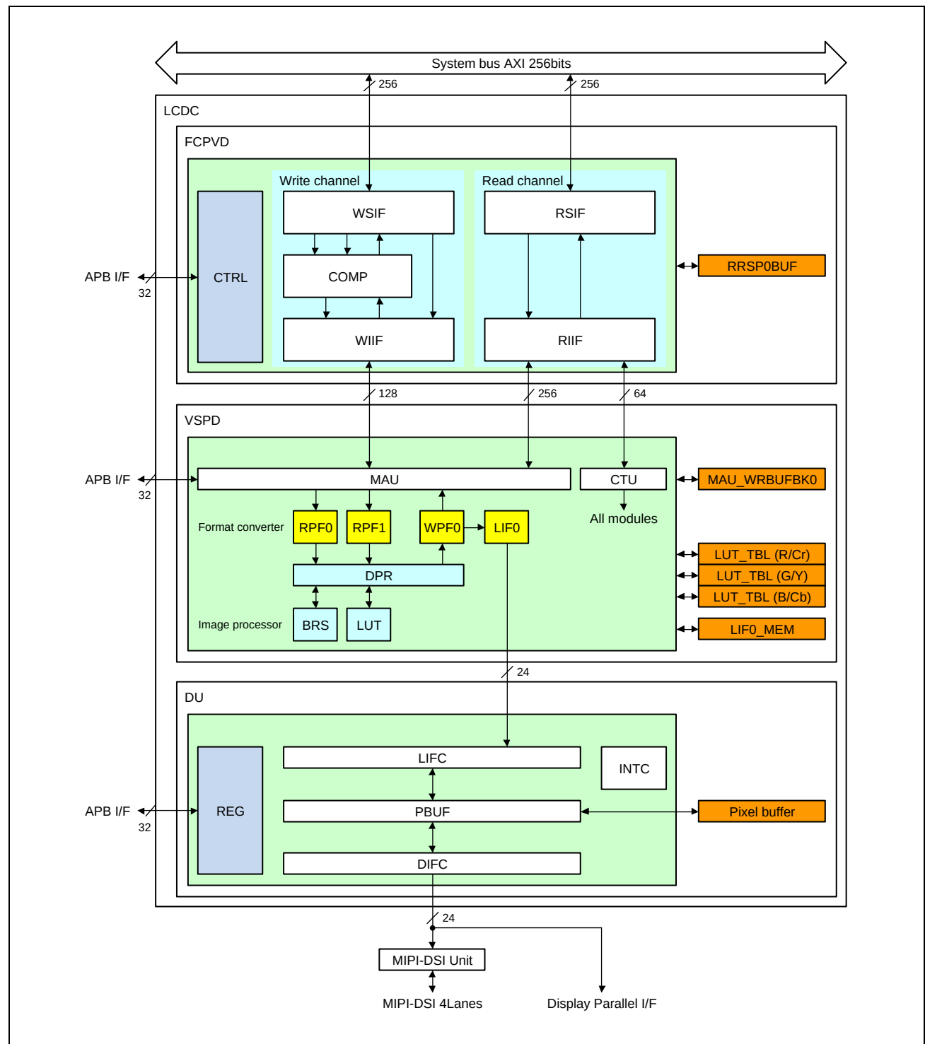
Figure 33.1 Block Diagram
