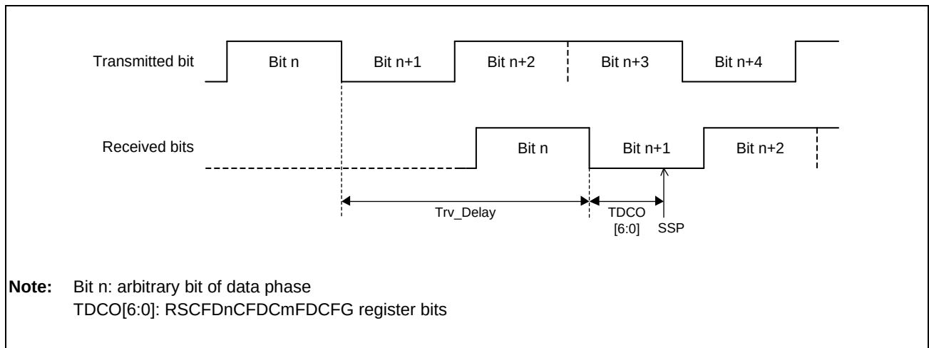
Figure 28.22 SSP Timing
