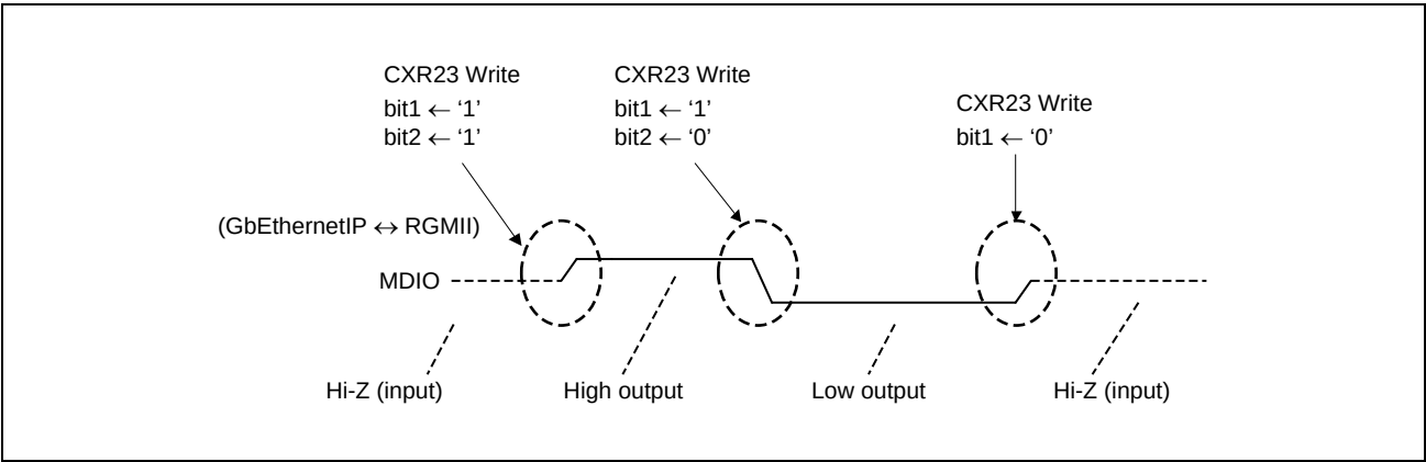
Figure 30.52 Relationship between CXR23 Write and MDIO (output) signal
