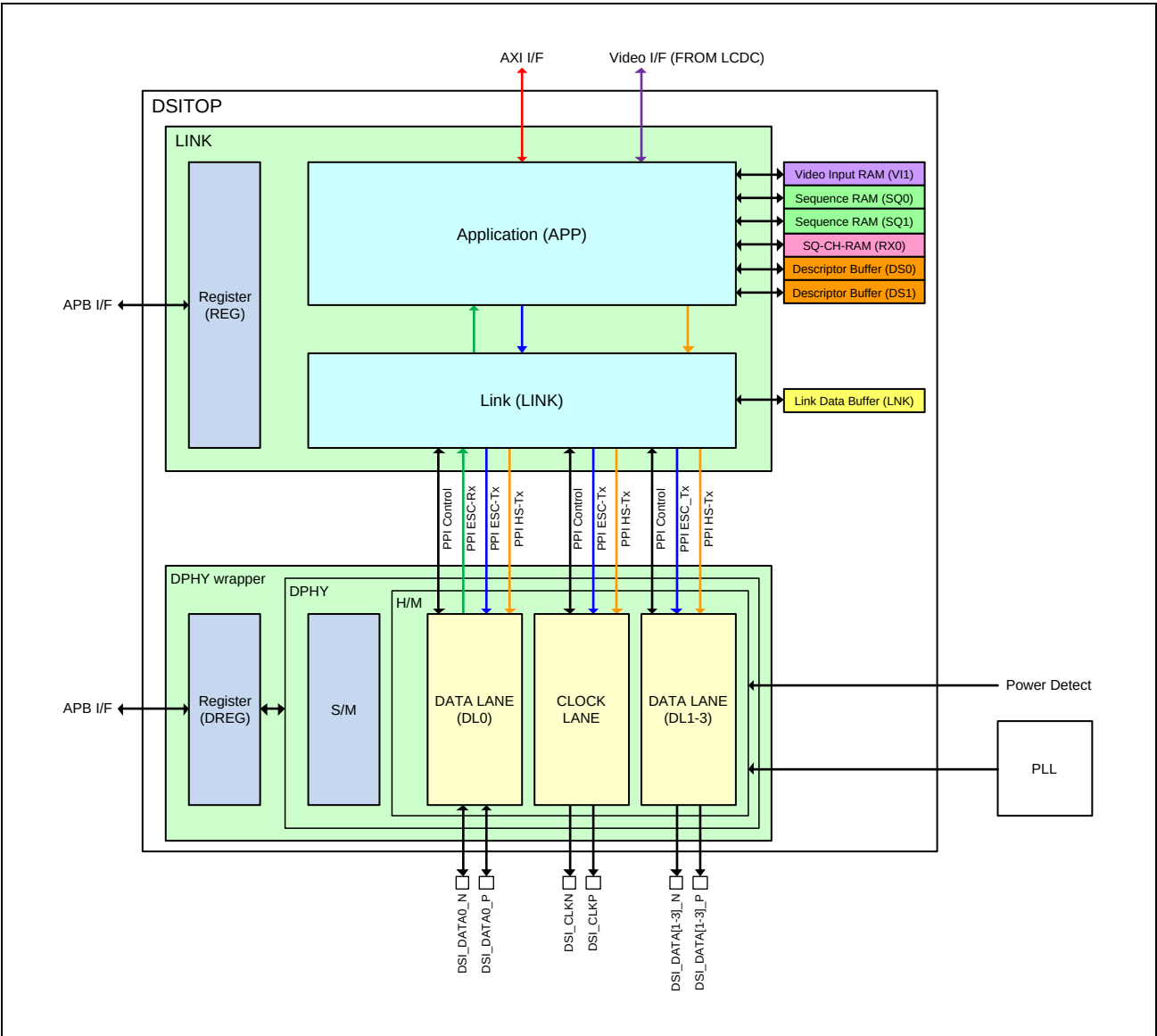
Figure 34.1 Block Diagram
