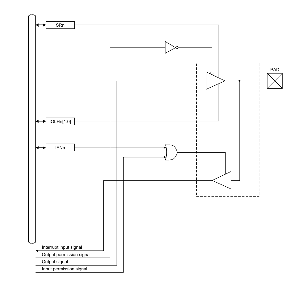
Figure 41.11 TMS/SWDIO
