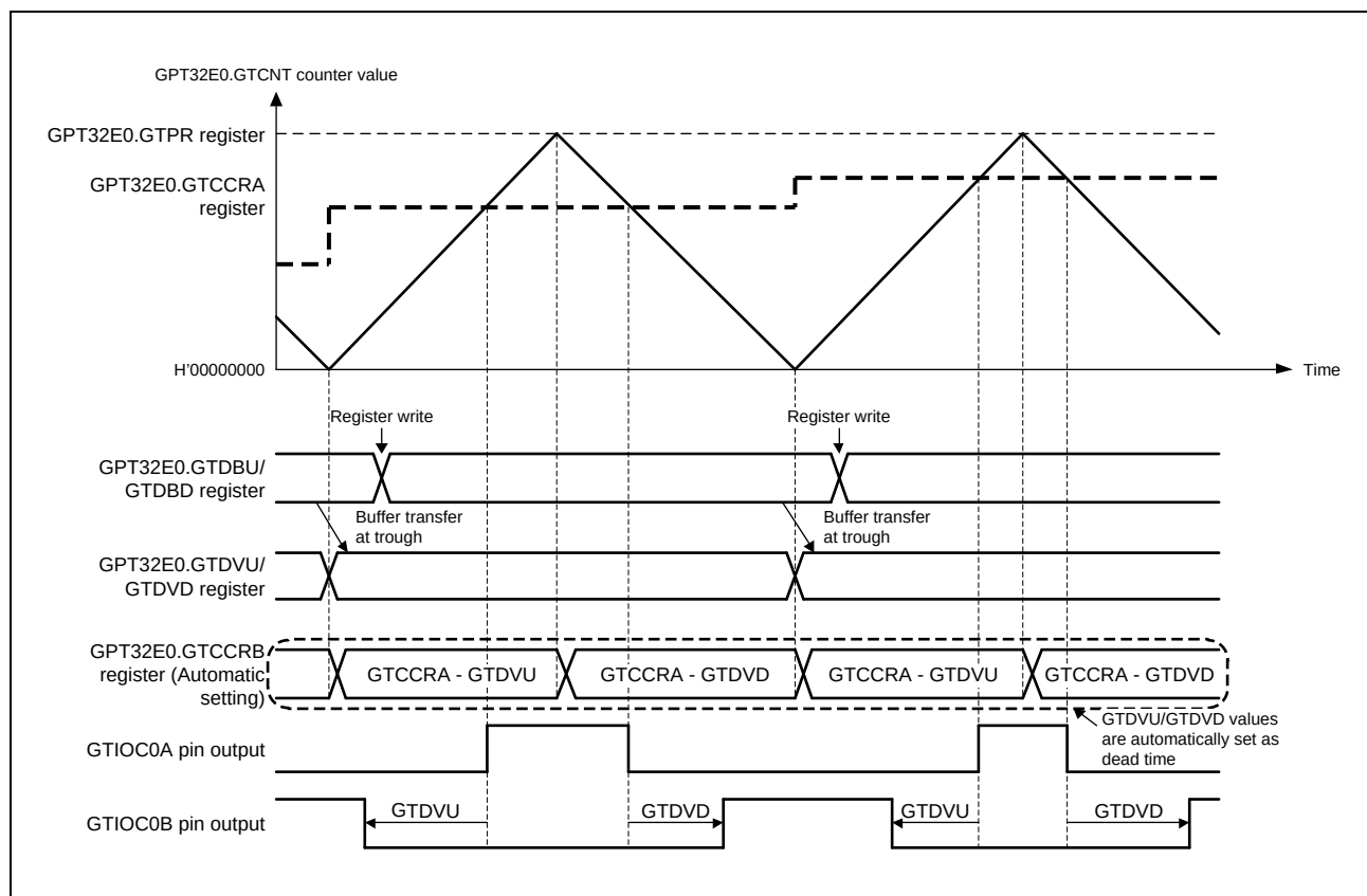
Figure 18.44 Example of automatic compare-match value setting function with dead time with triangle-wave PWM mode 1, GTDVU and GTDVD set to buffer operation, active-high
