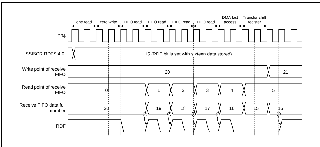
Figure 27.28 Set timing and clear timing of RDF
