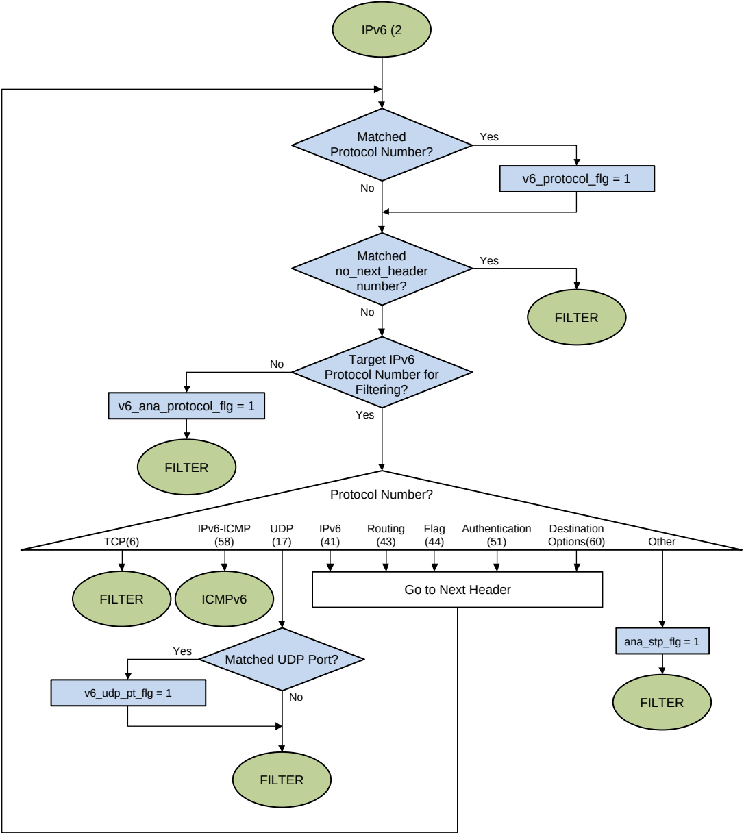
Figure 30.37 Received Frame Filtering Flow (Part4)
