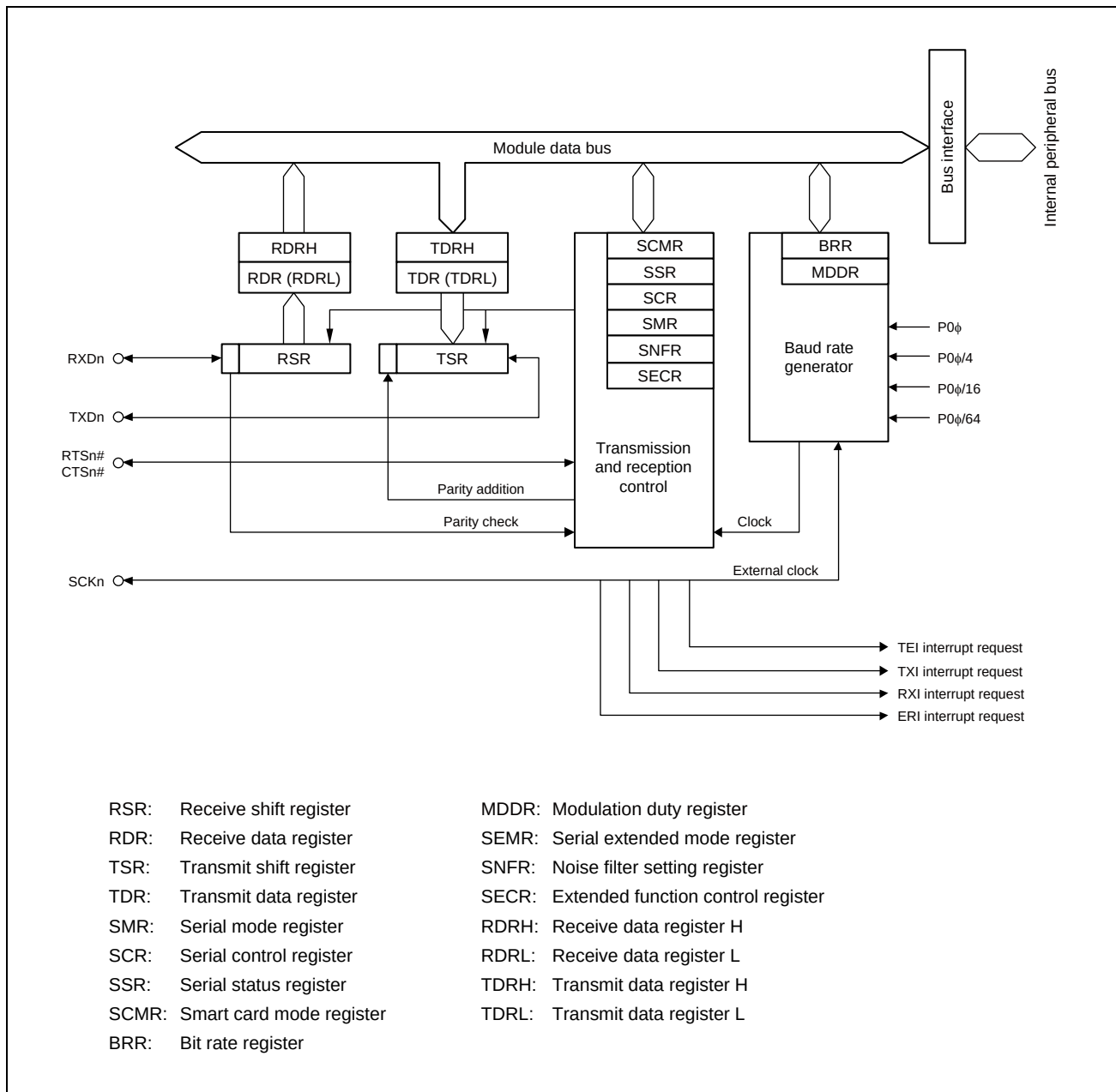
Figure 23.1 Block Diagram of SClg (SCI0 and SCI1)
