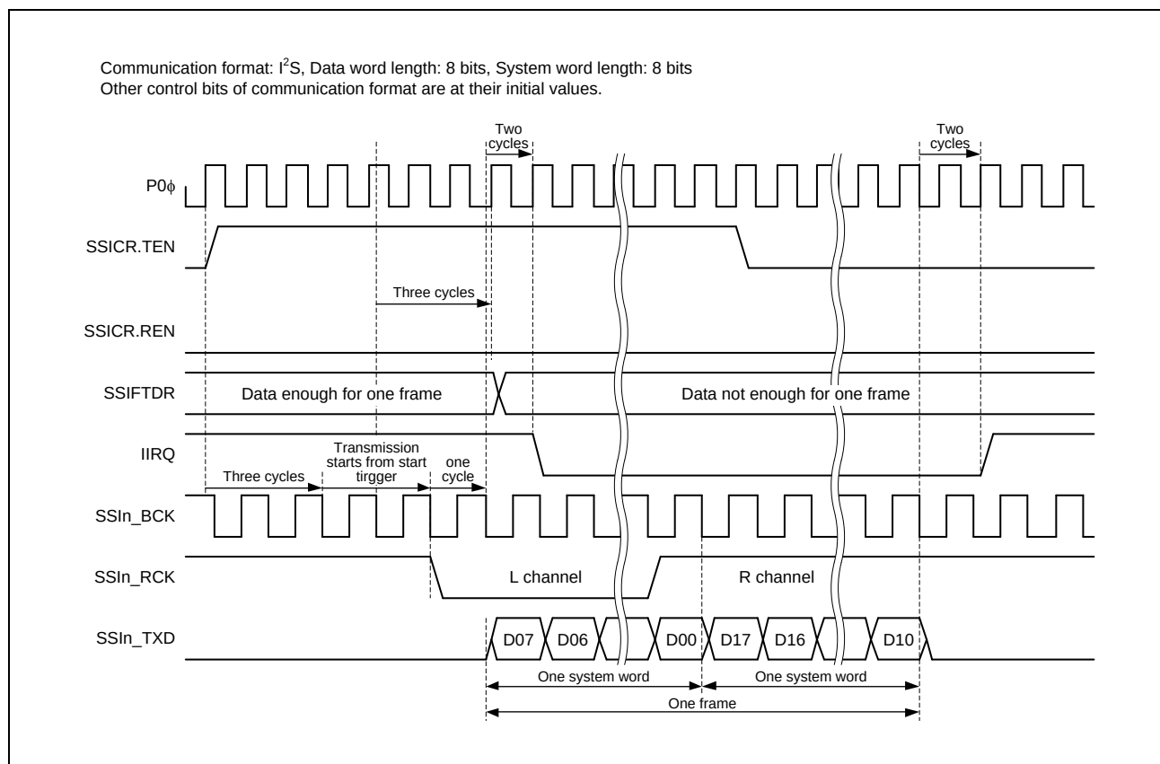
Figure 27.19 IIRQ Setting Timing (Transmission)
