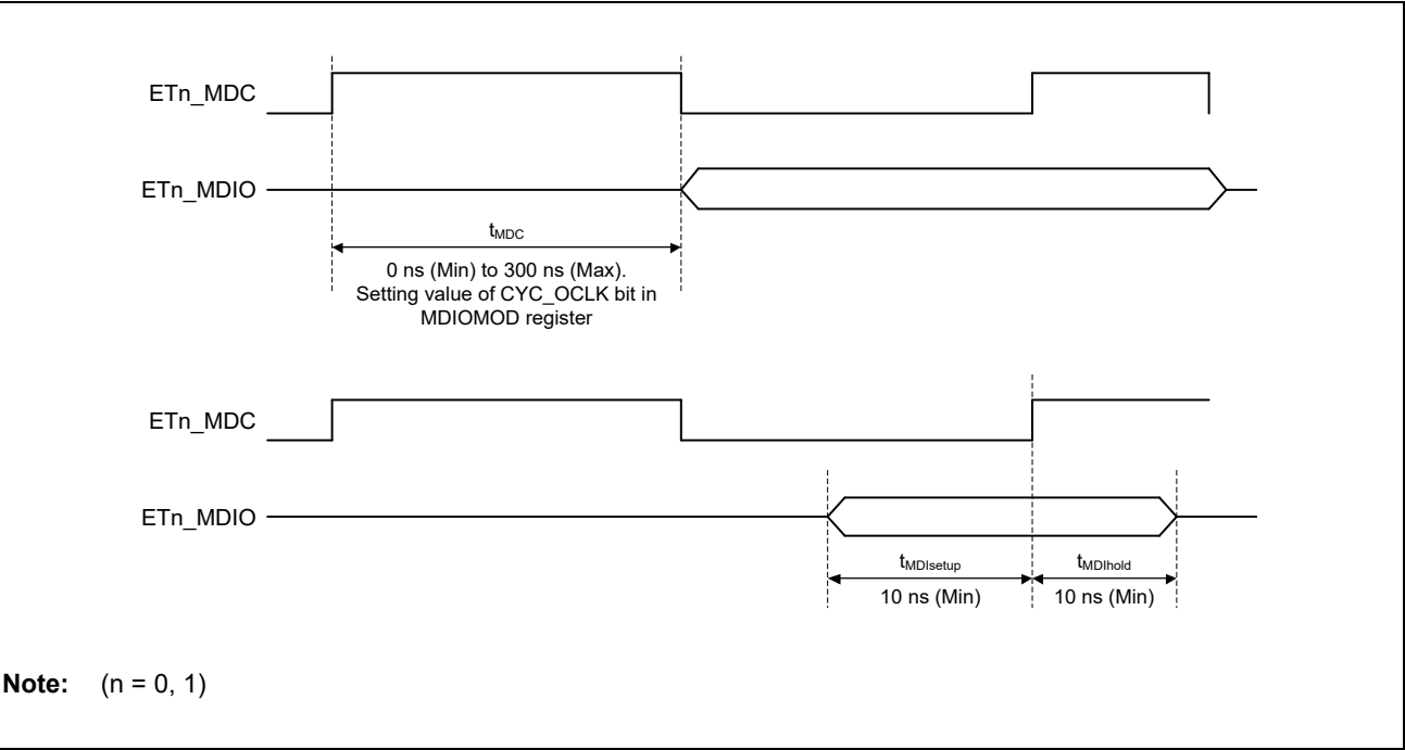
Figure 48.19 Management Interface
