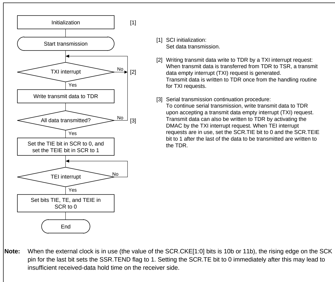
Figure 23.24 Example Flowchart of Serial Transmission in Clock Synchronous Mode
