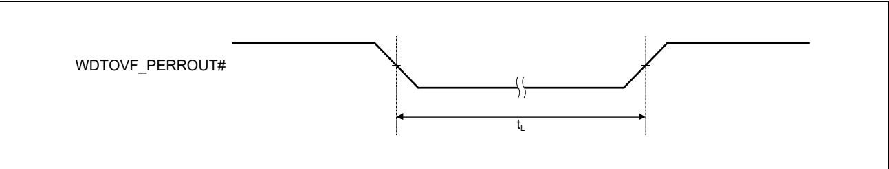
Figure 48.56 Watchdog Timer Output Timing
