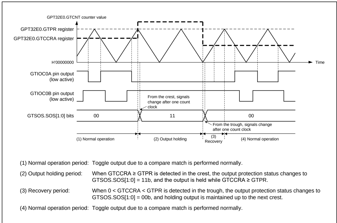
Figure 18.99 Example of output protection function operation when GTCCR \geq GTPR is set during buffer transfer at crests, with 0 < GTCCR < GTPR restored during buffer transfer at troughs, and active-low
