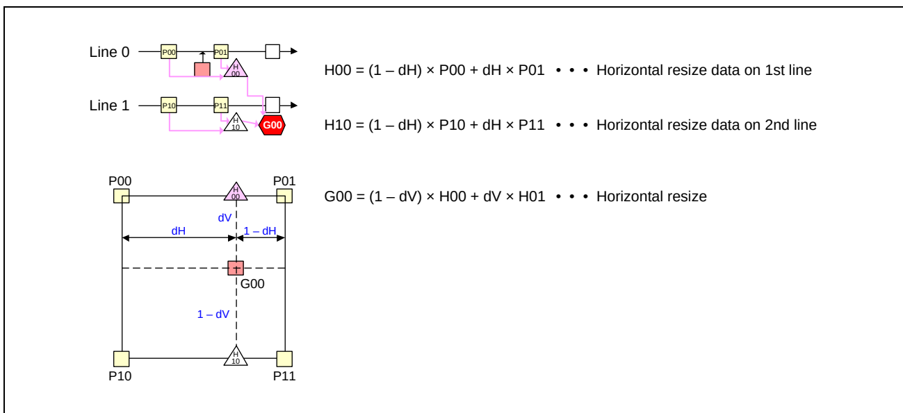
Figure 36.27 Calculation for 4 Points Bi-linear Resize
