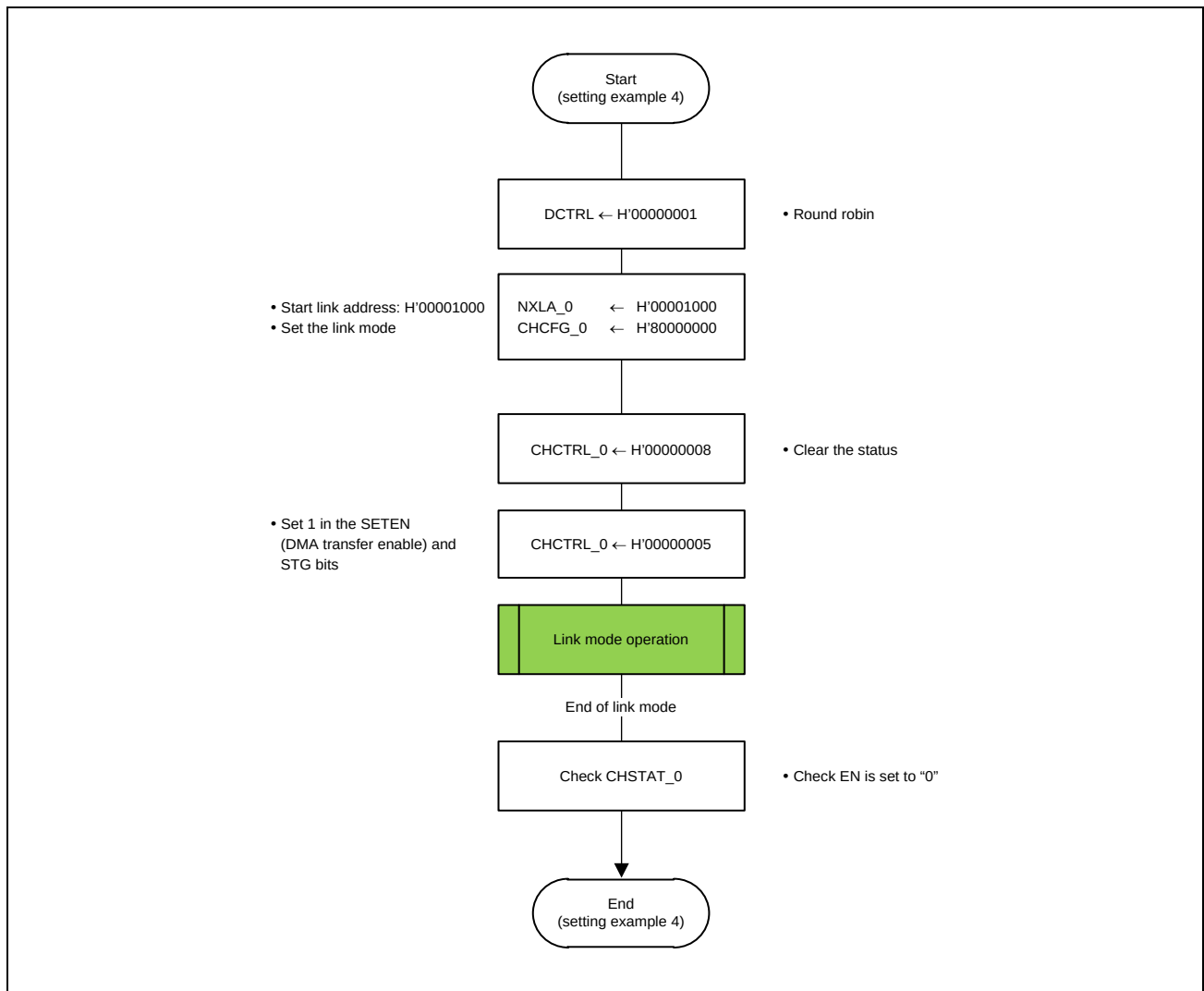
Figure 14.26 Setting Example 4
