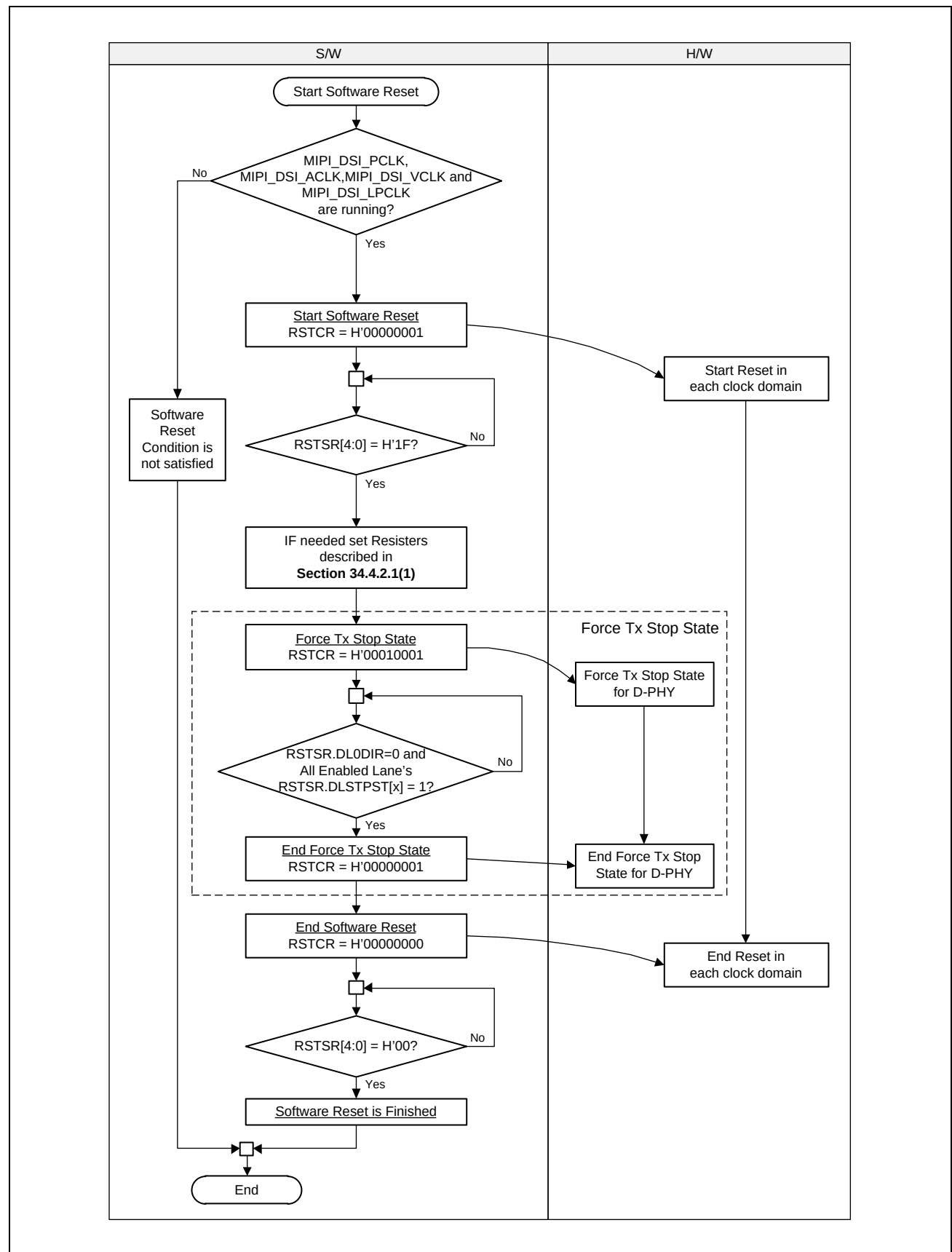
Figure 34.6 Software Reset
