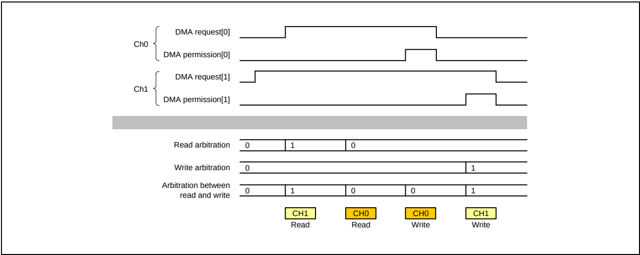
Figure 32B.24 Example of Operation in Round-Robin Mode (with 4 channels, REQD = 1)
