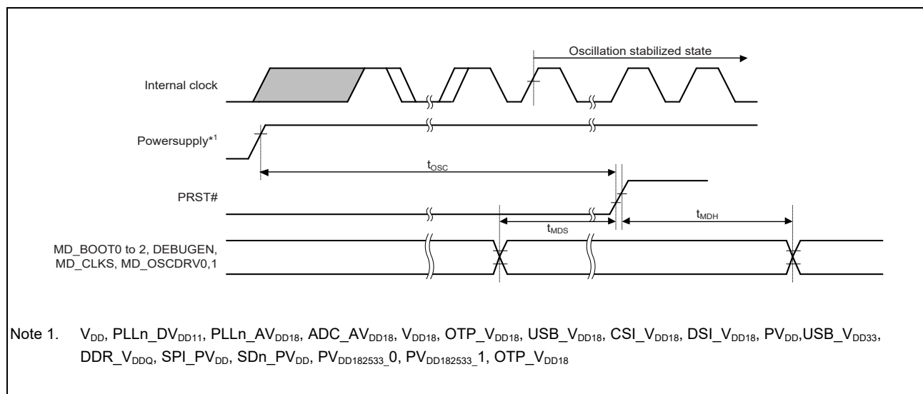
Figure 48.6 Power-On Oscillation Settling Time
