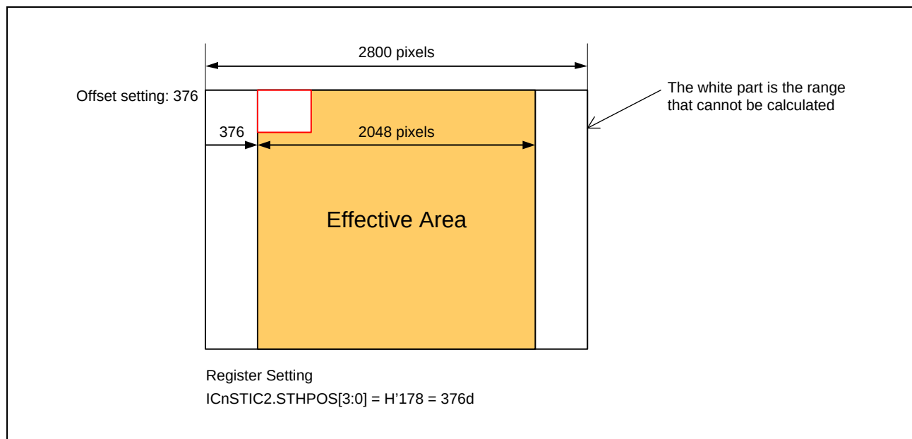
Figure 35.39 Statistics Calculation Example at 2800 Pixels Width
