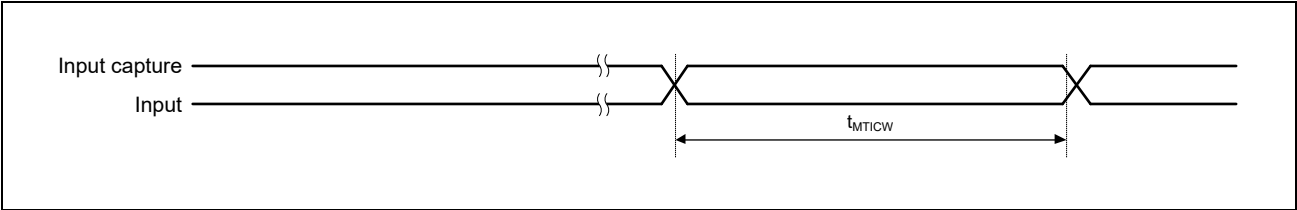
Figure 48.40 MTU3a Input Capture Input Timing
