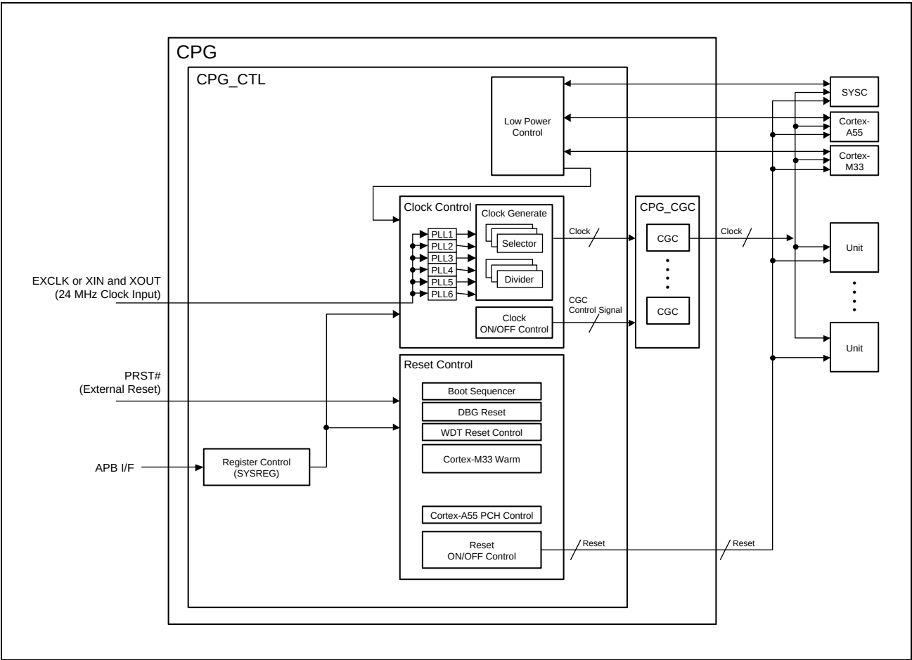
Figure 7.1 CPG Configuration
