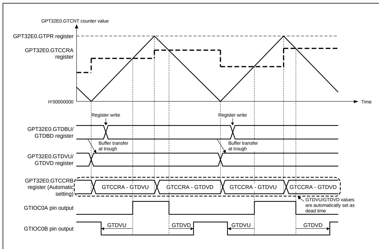
Figure 18.45 Example of automatic compare-match value setting function with dead time, with triangle-wave PWM mode 2 or 3, GTDVU and GTDVD set to buffer operation, and active-high
