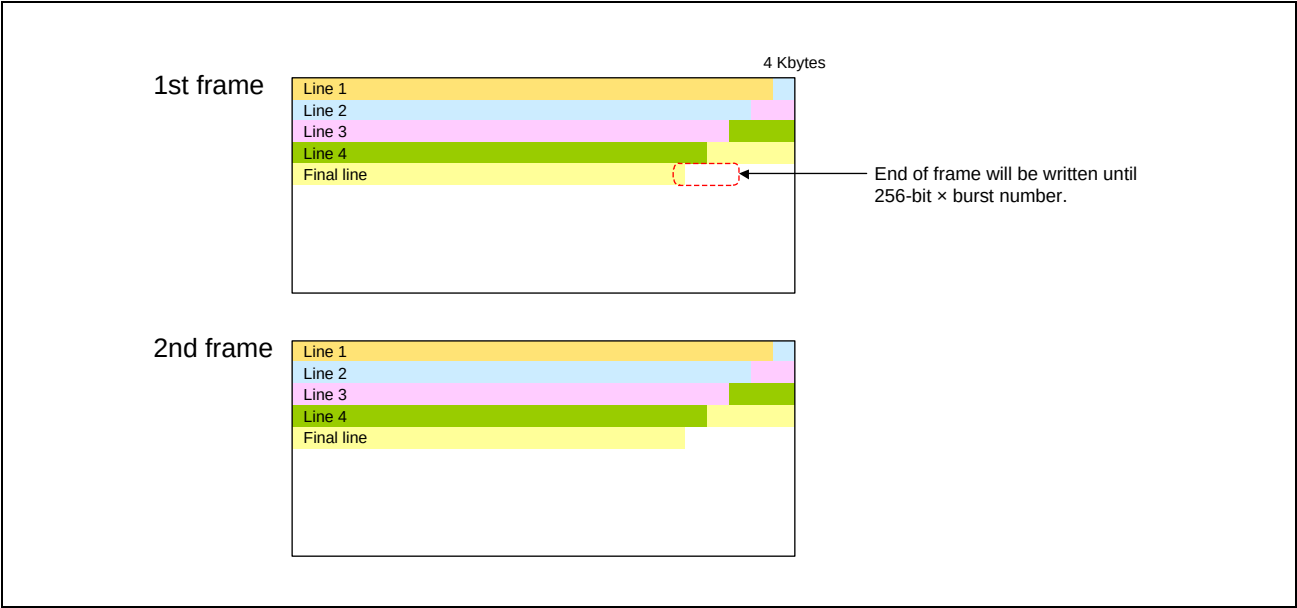
Figure 35.23 Data Storage
