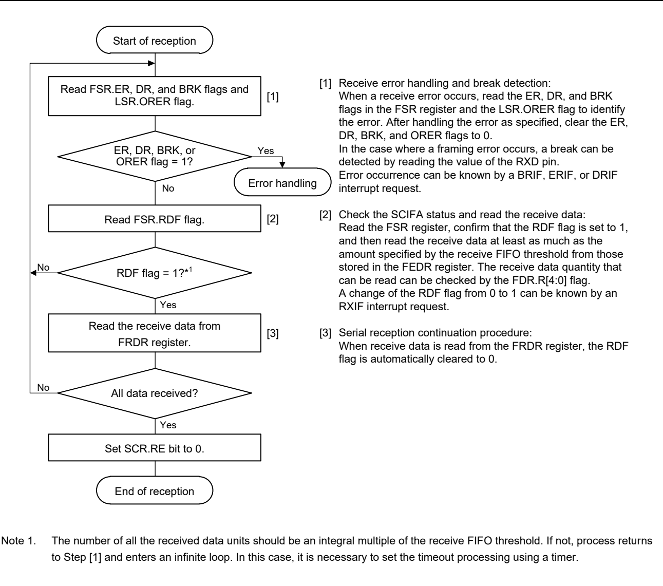
Figure 22.7 Sample Flowchart for Receiving Serial Data in Asynchronous Mode (1)
