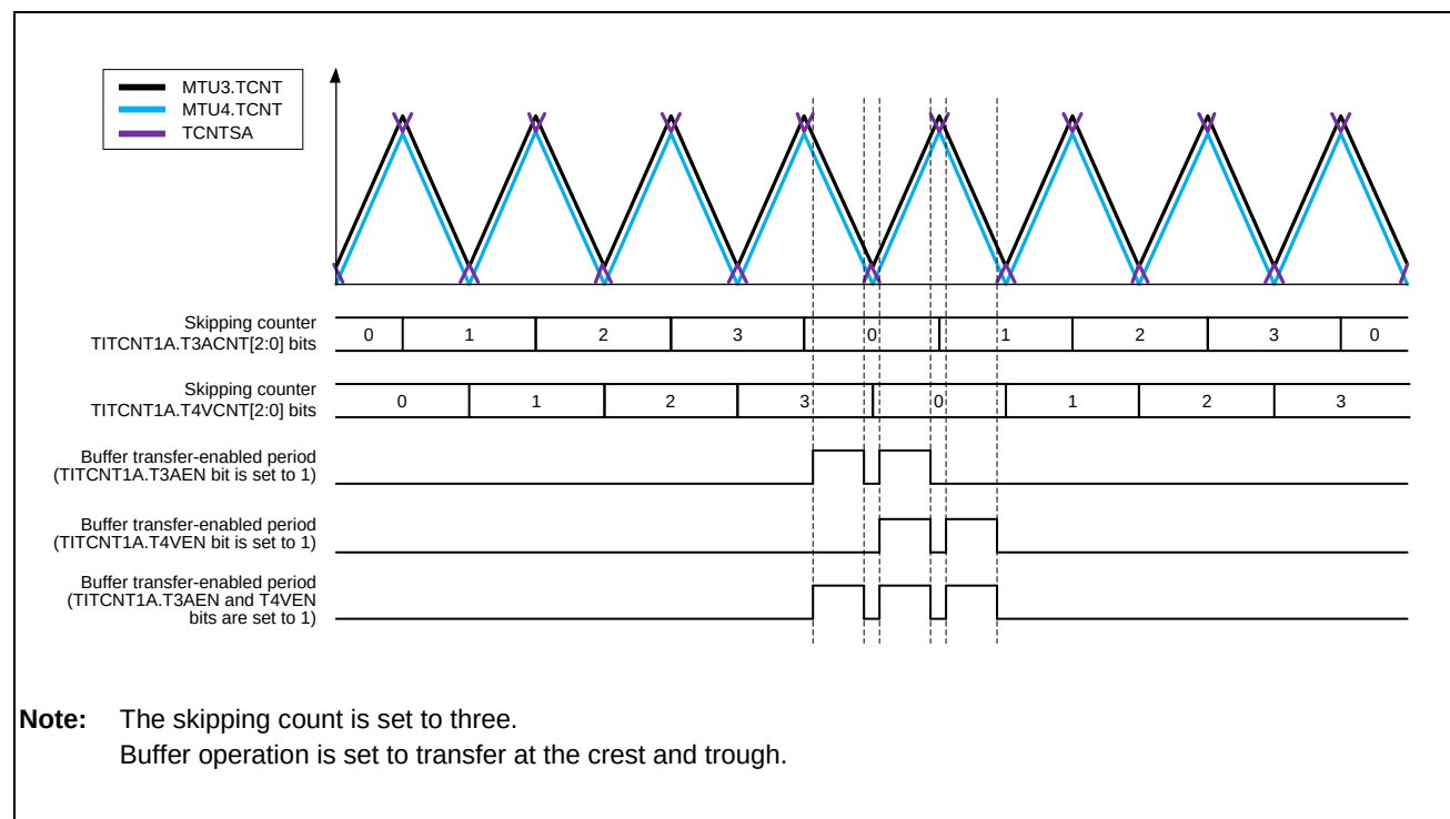
Figure 16.91 Relationship between Bits T3AEN and T4VEN in TITCR1A and Buffer Transfer-Enabled Period
