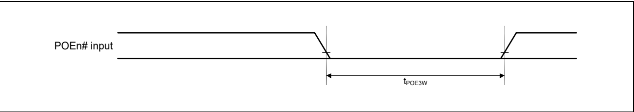
Figure 48.42 POEn# Input Pulse Timing
