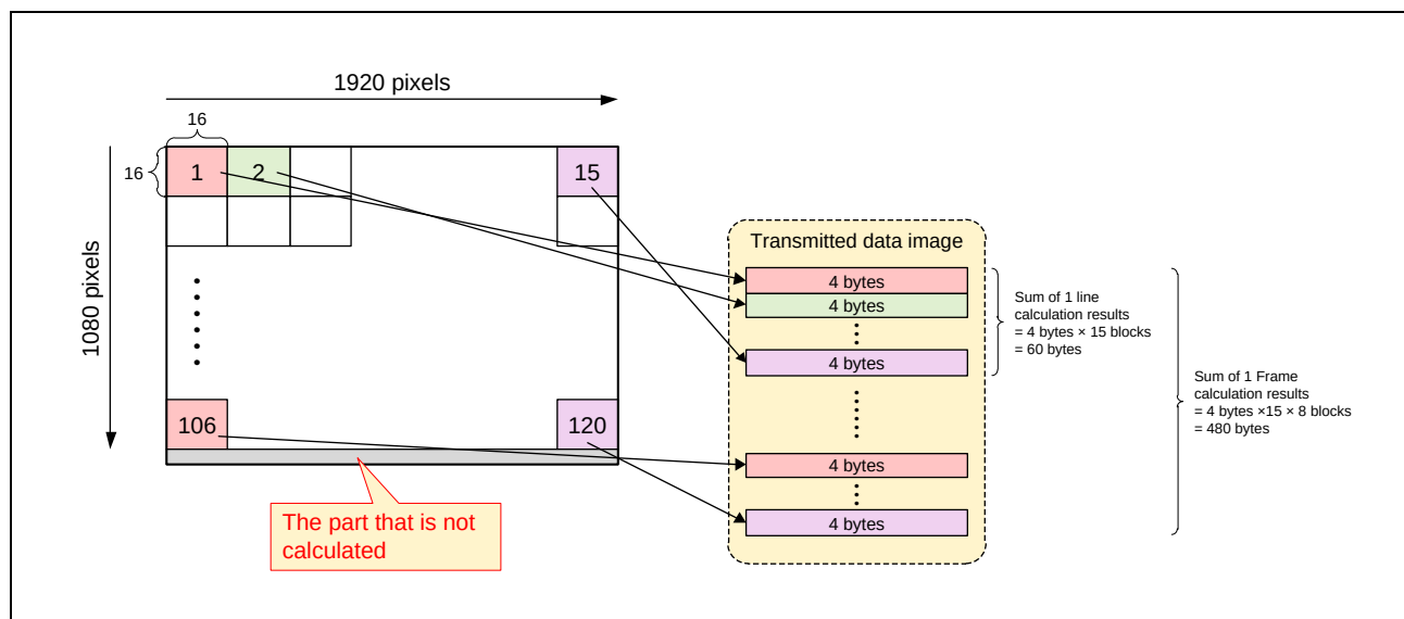
Figure 35.38 Illustration Diagram of the Amounts of Data in the Operations when a 1920×1080 Pixel Area is Set as 16×16 Blocks
