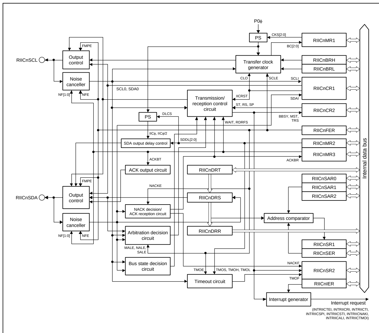
Figure 26.1 Block Diagram of IIC
