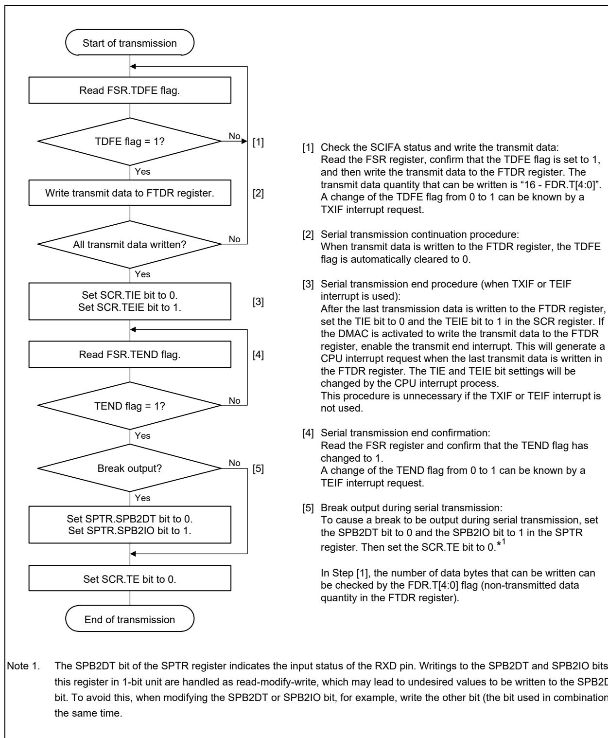
Figure 22.4 Sample Flowchart for Transmitting Serial Data in Asynchronous Mode
