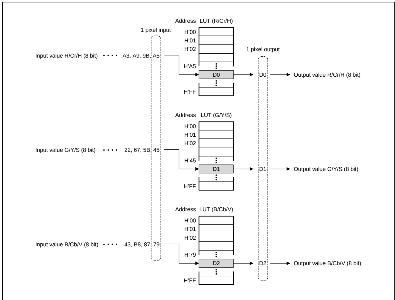
Figure 33.24 Relationship between Input and Output for 1D-LUT Table
