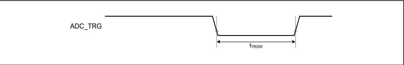
Figure 48.55 ADC Trigger Input Timing
