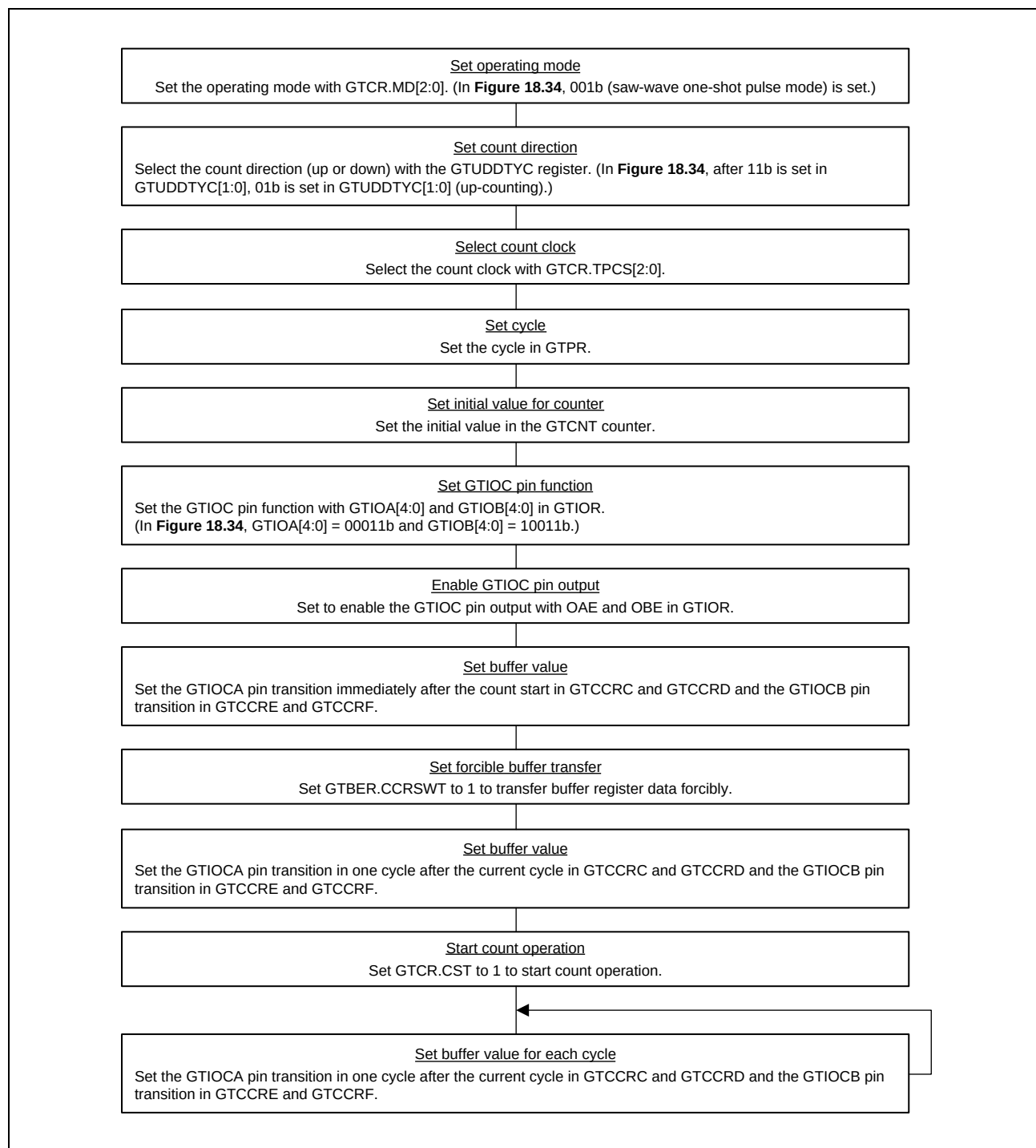
Figure 18.35 Example setting for saw-wave one-shot pulse mode
