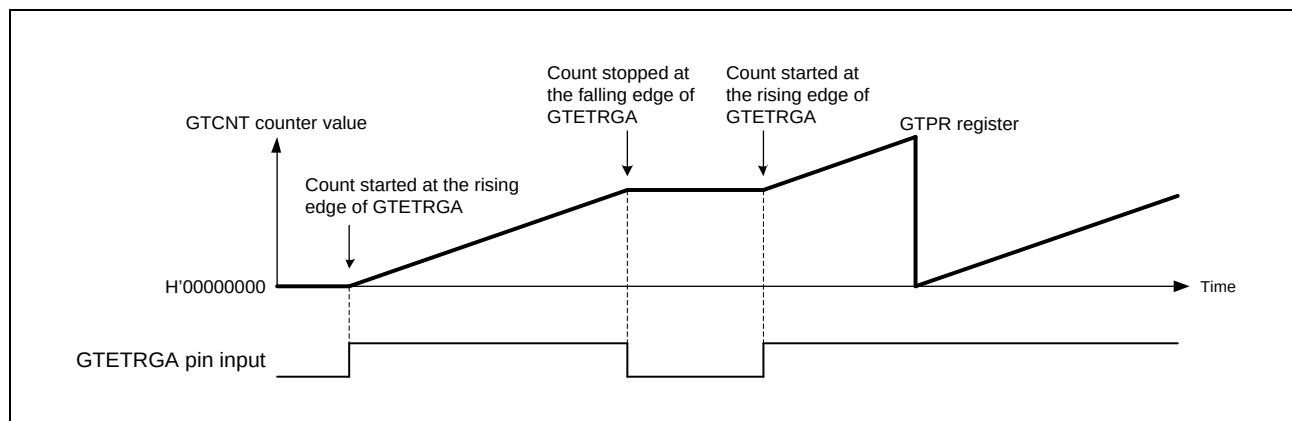
Figure 18.54 Example of count start/stop operation by hardware source, started on the rising edge of the GTETRGA pin input and stopped on the falling edge of the GTETRGA pin input
