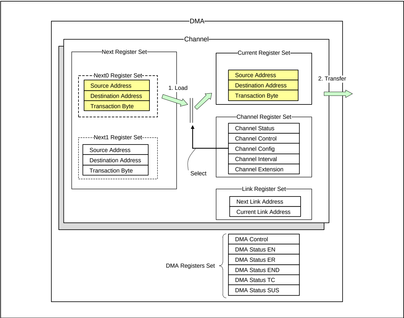
Figure 14.1 Register Configuration
