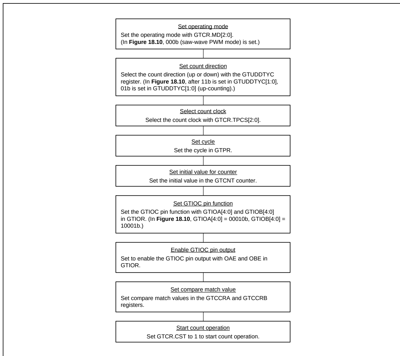
Figure 18.11 Example setting for low output and high output operation
