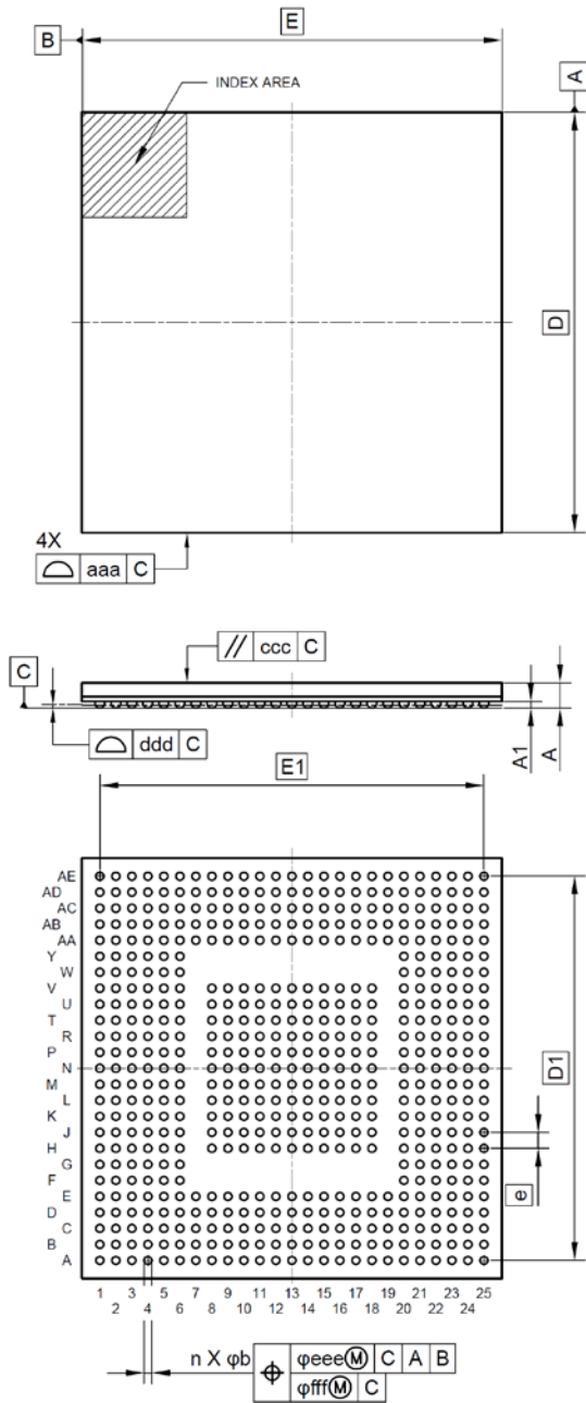
Appendix A.1 Package Dimensions (551-pin BGA, 21-mm Square, 0.8-mm Pitch)
