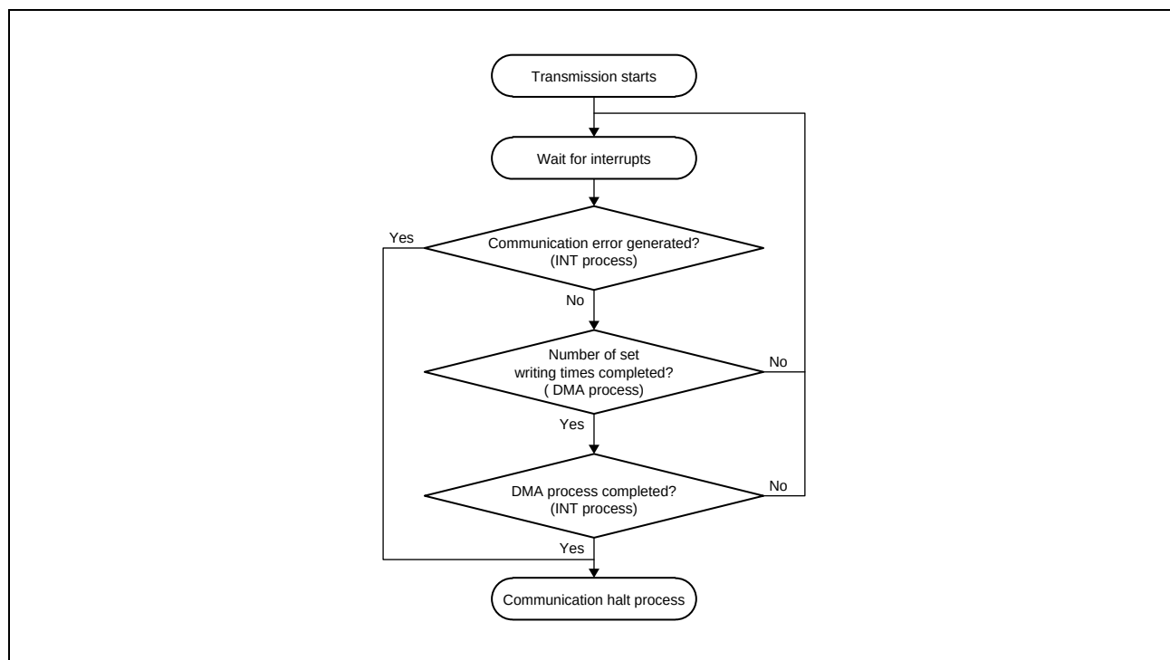
Figure 27.53 Transmission Procedure
