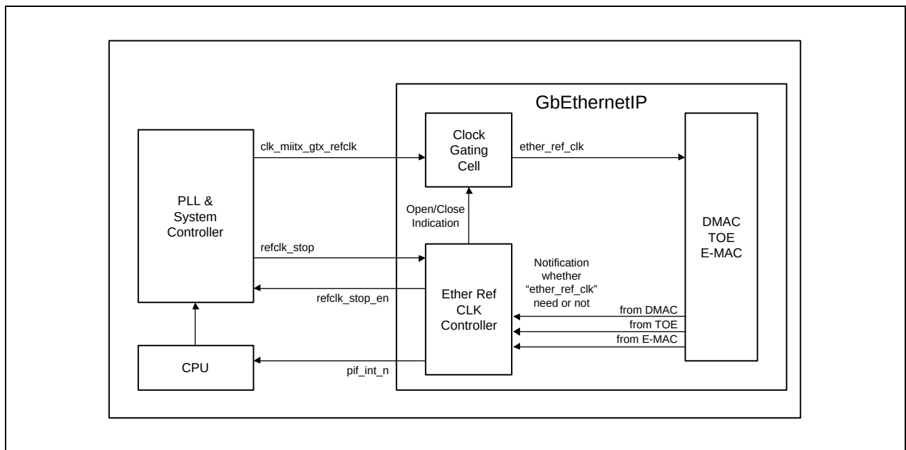
Figure 30.42 Block Diagram
