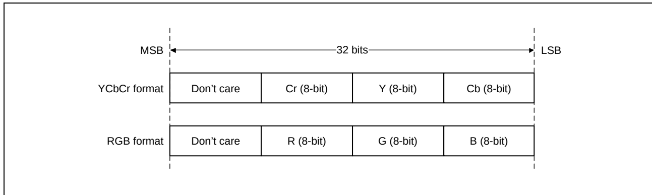
Figure 33.37 VI6_LUT_TBL Formats
