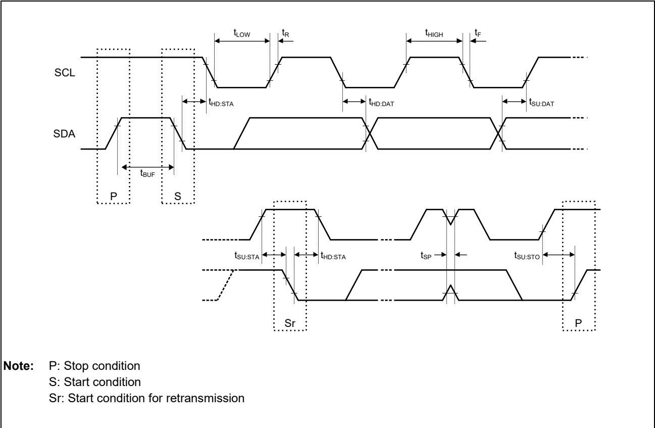
Figure 48.45 Input/Output Timing
