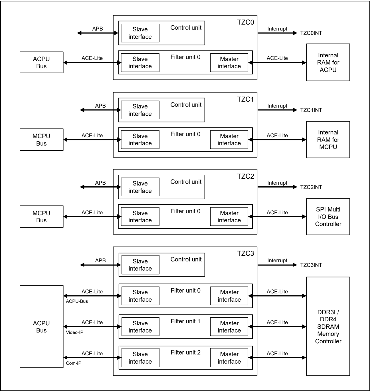
Figure 13.1 Block Diagram
