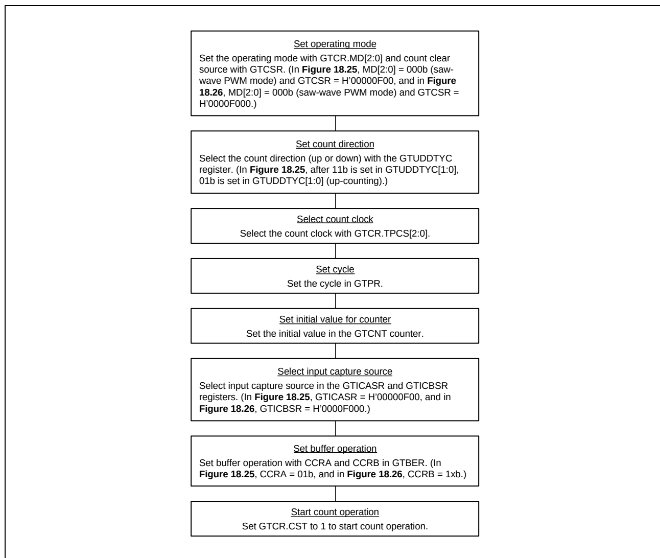
Figure 18.27 Example setting for GTCCRA and GTCCRB buffer operation with input capture
