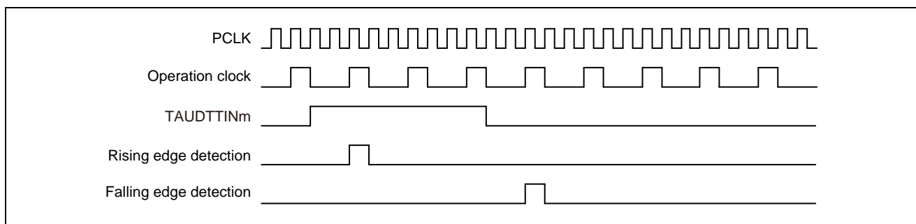
Figure 20.25 Basic Edge Detection Timing
