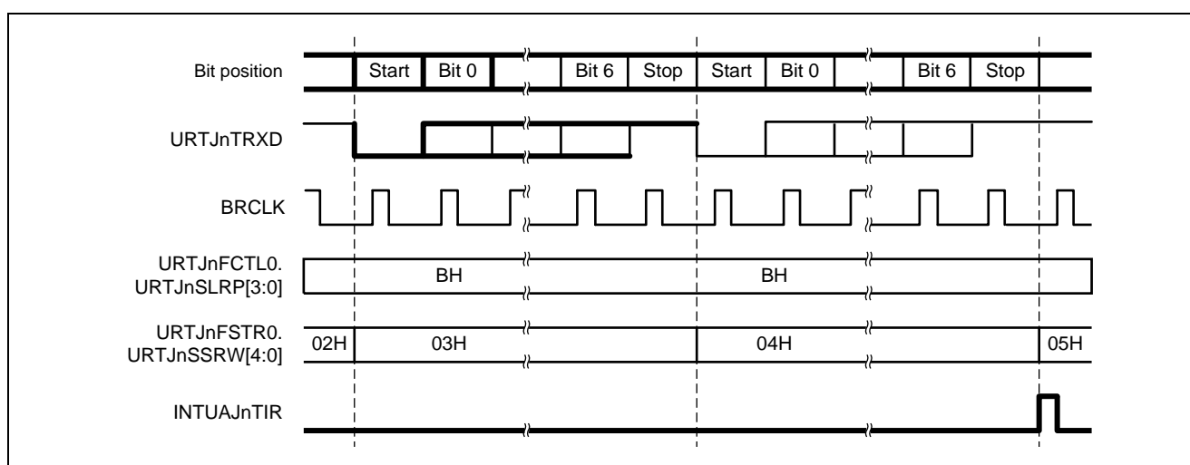
Figure 22.3 Reception Interrupt Request Timing
