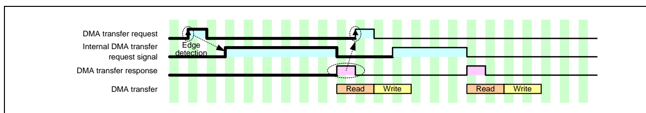
Figure 18.22 Edge Detection Mode Operation Example 1
