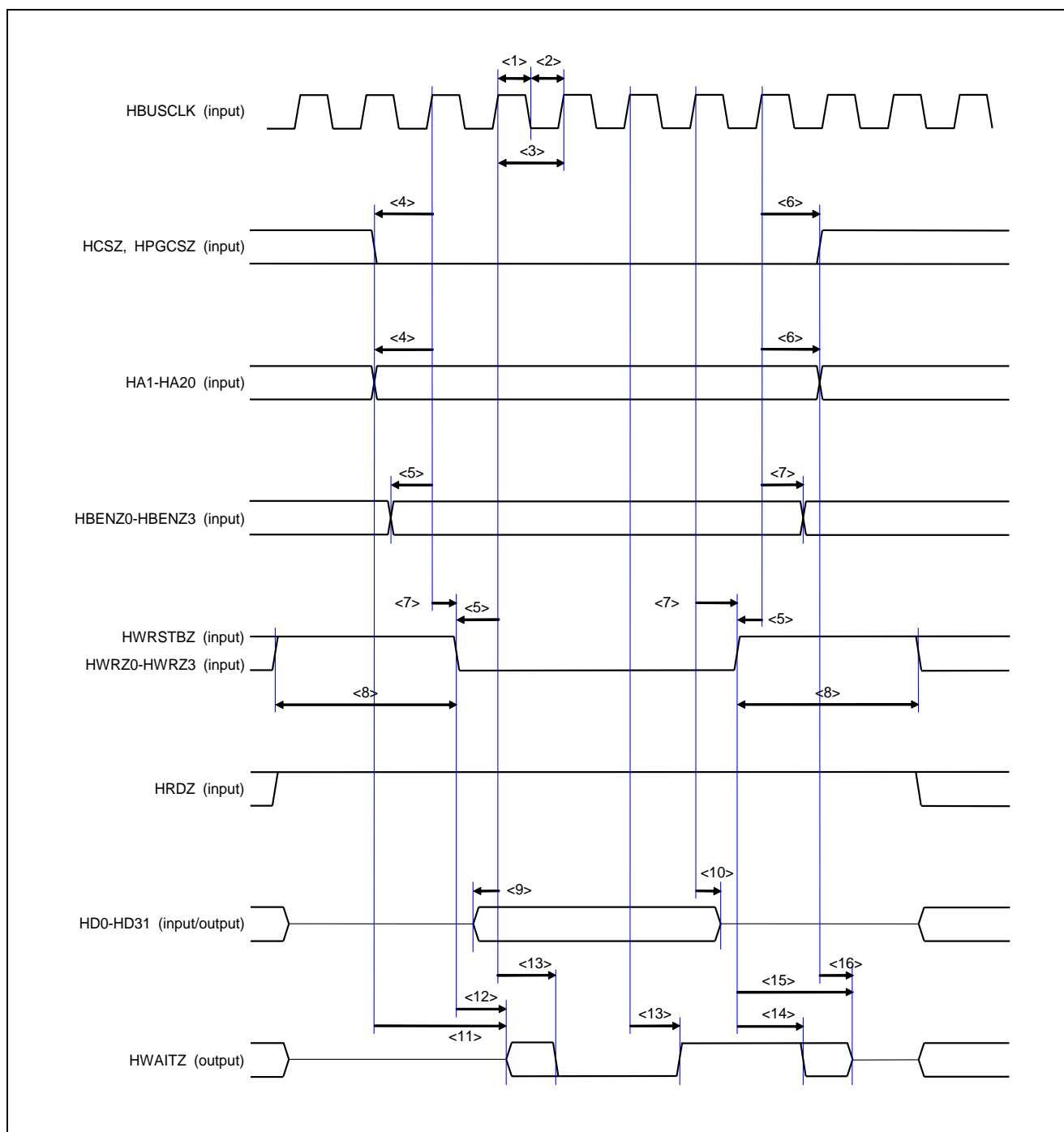
Figure 29.11 External MCU Interface Write Timing (MEMCSEL=L, HIFSINC=H)
