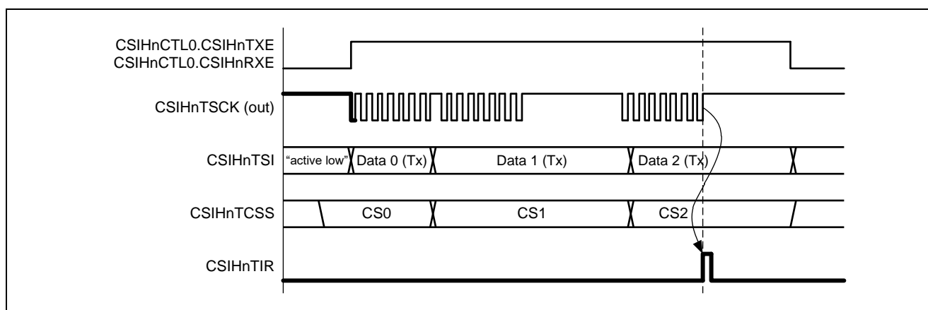
Figure 23.26 CSIHnTIR Generation in Dual Buffer Mode
