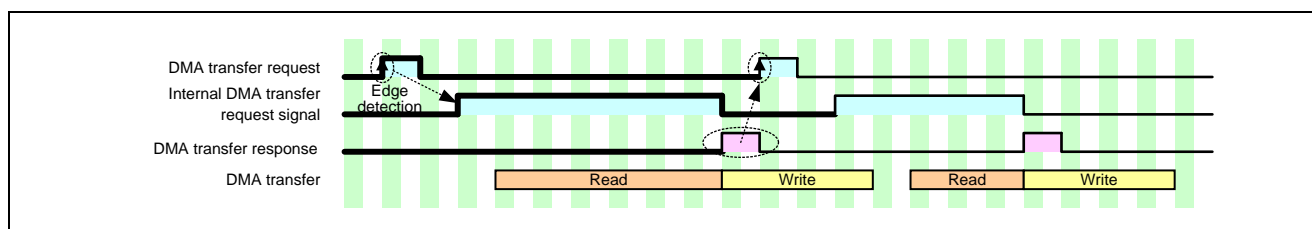
Figure 18.23 Edge Detection Mode Operation Example 2
