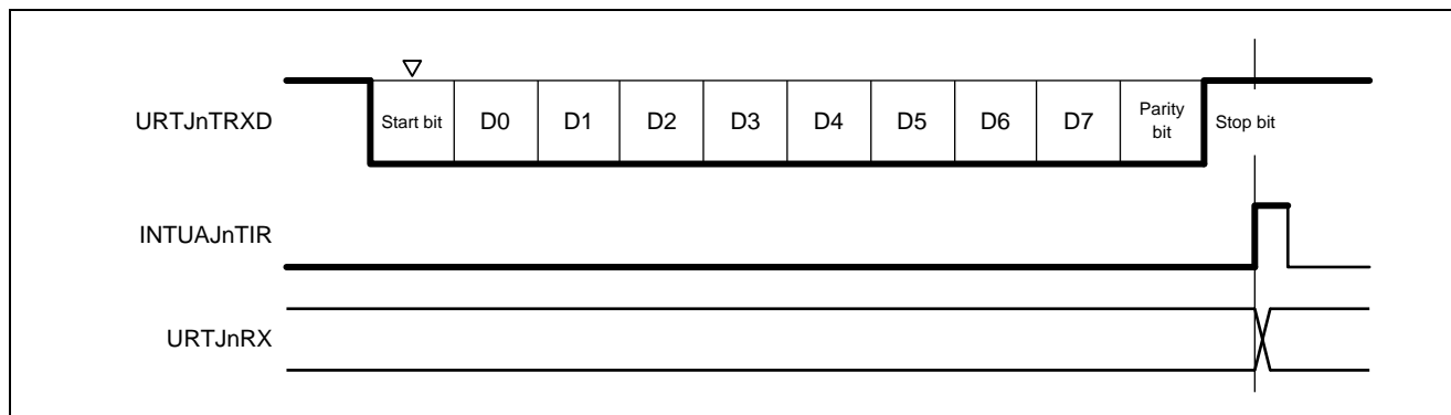
Figure 22.13 UARTJn Reception
