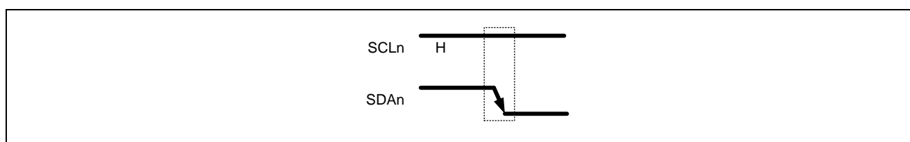
Figure 24.4 Start Condition
