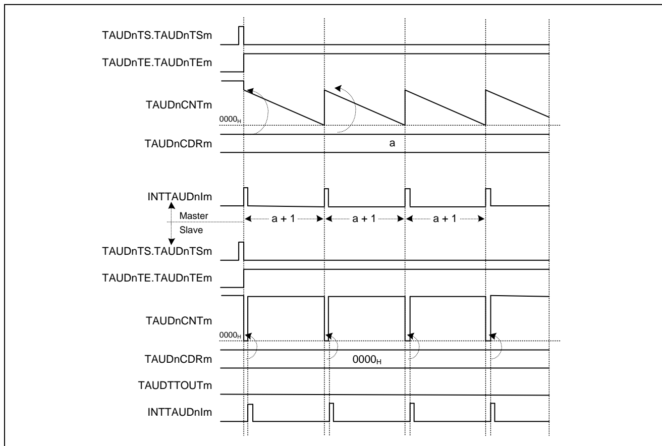
Figure 20.90 TAUDnCDRm (Slave) = 0000_H , Positive Logic (TAUDTOL.TAUDTOLm (Slave) = 0)
