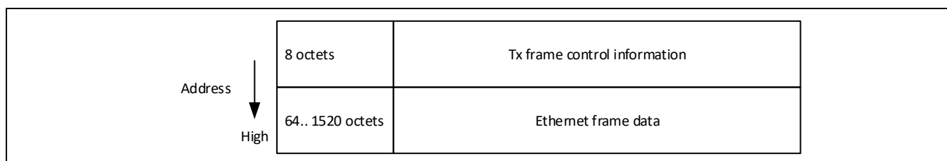
Figure 12.12 TX Data Format
