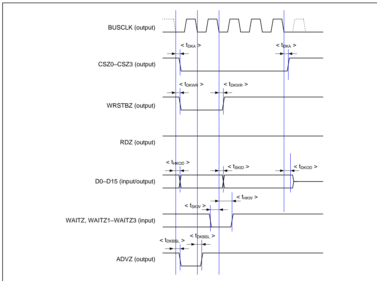
Figure 29.10 Memory Controller Write Timing (Clock Synchronous Memory)
