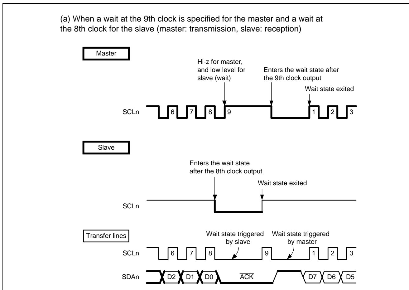
Figure 24.9 Wait State (1/2)
