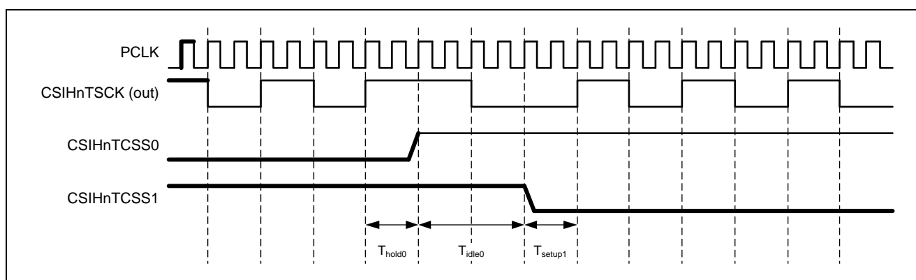
Figure 23.9 Clock Phase Timing (in the case of \text{PCLK}/4 , T_{\text{hold0}} = T_{\text{setup1}} = 0.5 \text{ SCK} , T_{\text{idle0}} = 1.0 \text{ SCK} , \text{CKP0} = 0 ( \text{CSIHnTCSS0} ) \rightarrow \text{CKP1} = 1 ( \text{CSIHnTCSS1} ))
