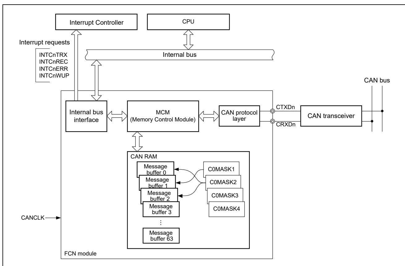
Figure 25.1 Block Diagram of the CAN Controller
