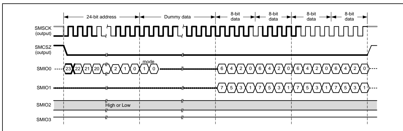
Figure 17.20 Bus Cycles for Fast Read Dual Output (in Instruction-Omission Mode)
