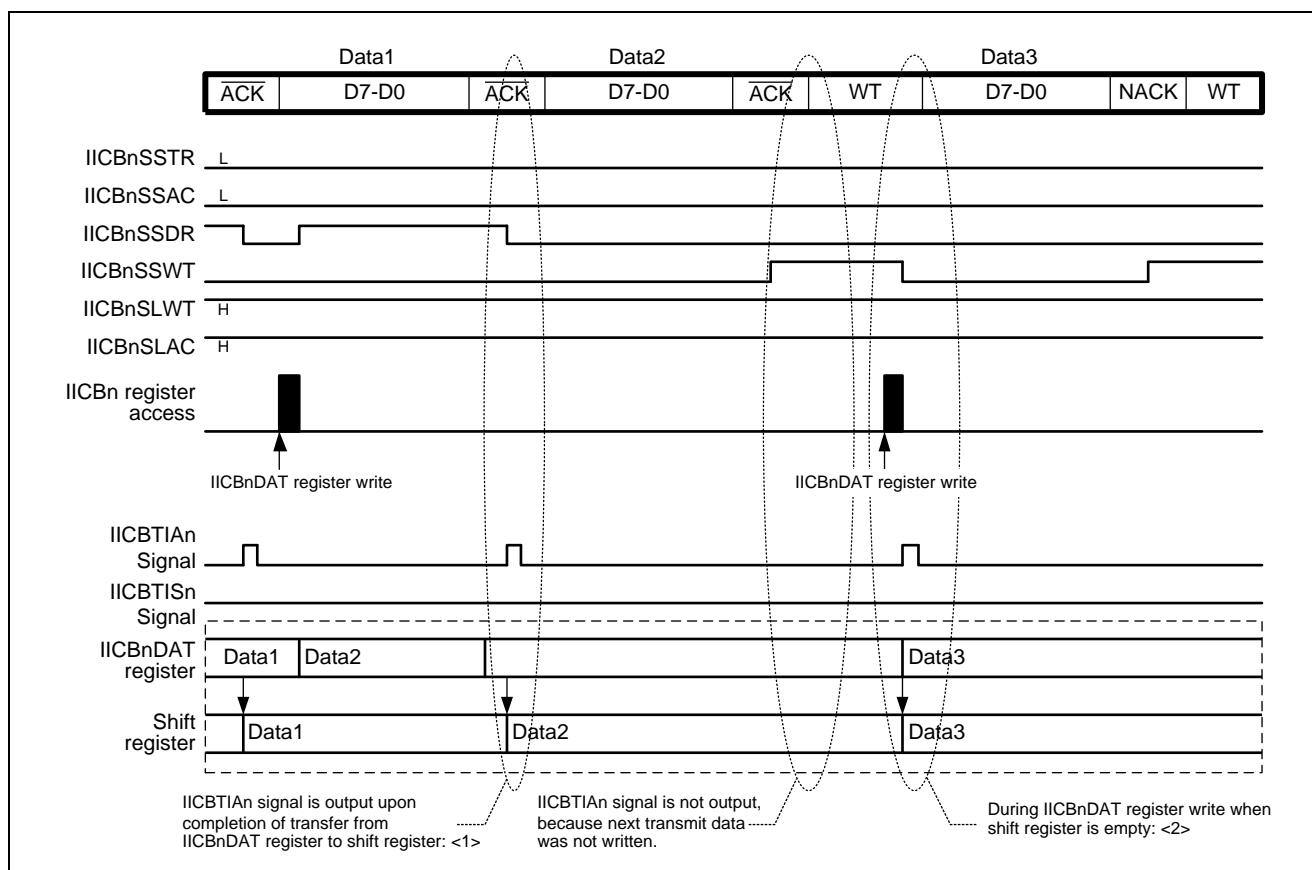
Figure 24.13 IICBTIA signal Output Timing (Transmission in Continuous Transfer Mode)
