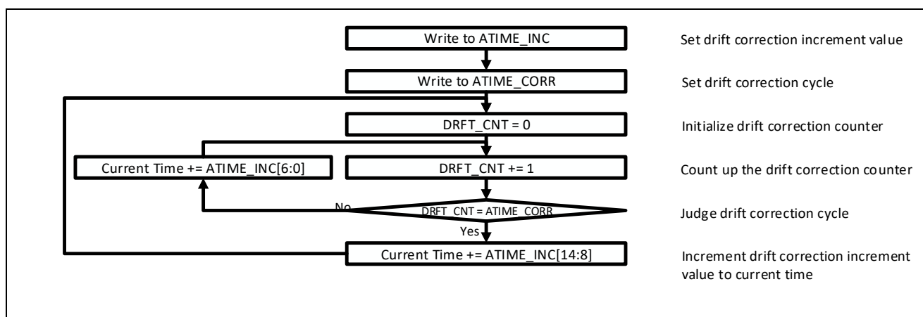
Figure 13.16 Drift Correction
