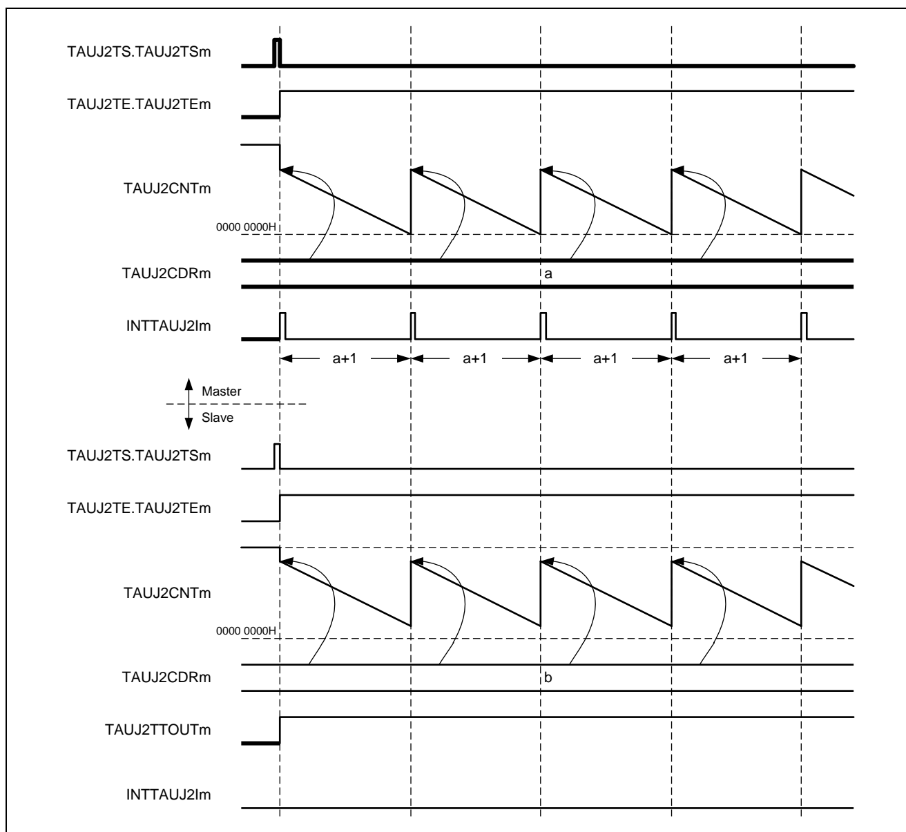
Figure 19.39 TAUJ2CDRm (Slave) \geq TAUJ2CDRm (Master) + 1, Positive Logic (TAUJ2TOL.TAUJ2TOLm (Slave) = 0)
