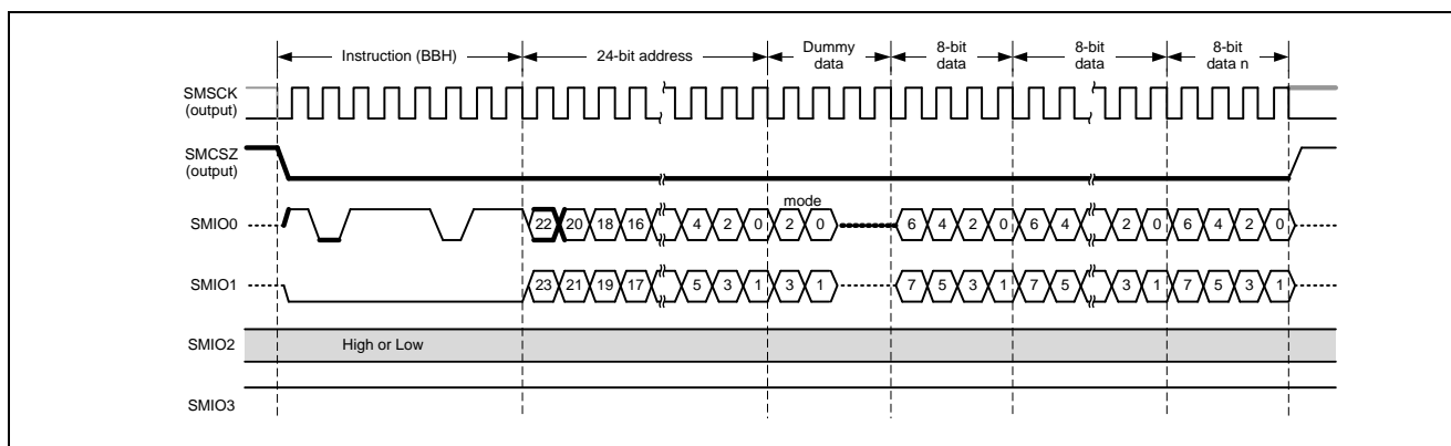
Figure 17.21 Bus Cycles for Fast Read Dual I/O
