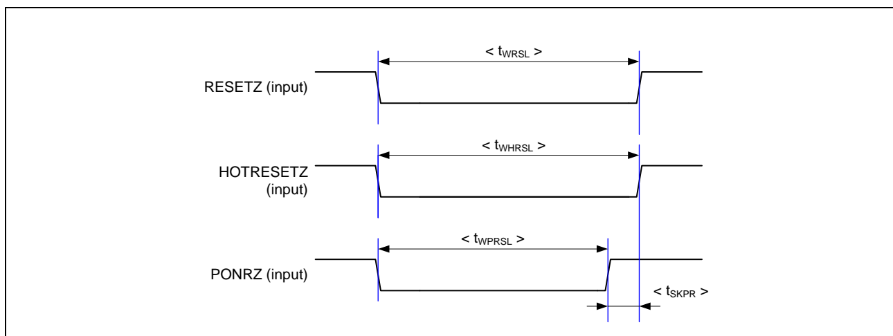
Figure 29.6 Reset Timing
