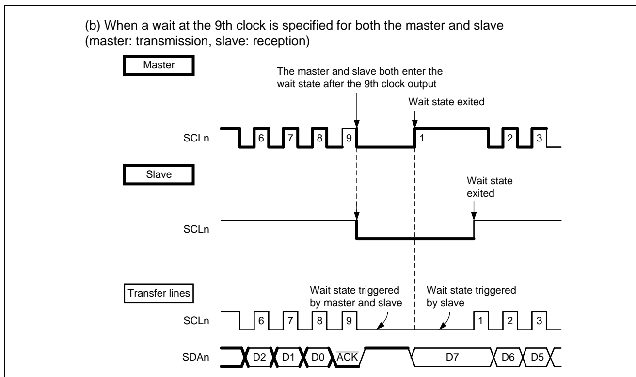
Figure 24.9 Wait State (2/2)
