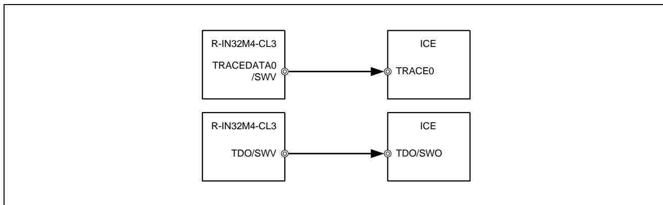
Figure 9.6 SWV Interface Connection Example
