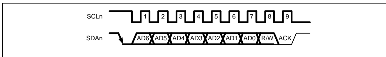
Figure 24.7 Acknowledge (ACK)
