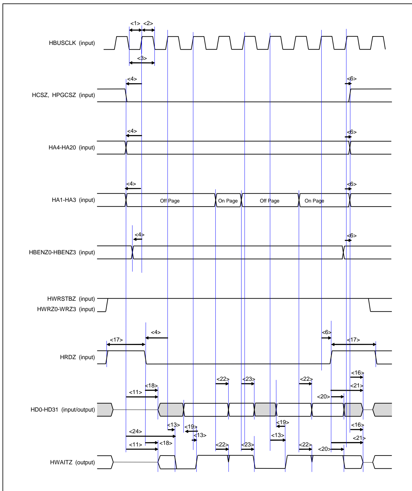
Figure 29.13 External MCU Interface Page Read Timing (MEMCSEL=L, HIFSYNC=H)
