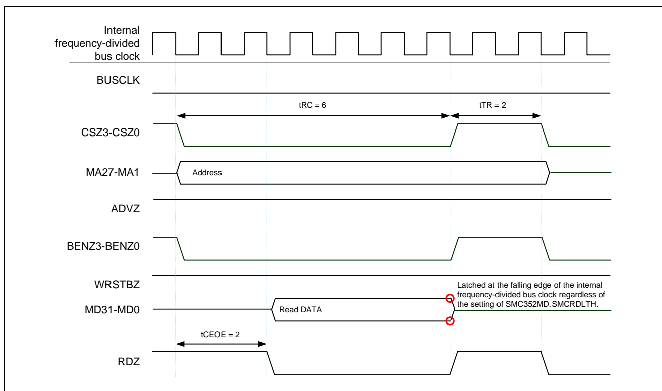
Figure 15.8 Asynchronous SRAM, Separate Bus Mode, Read Access, ADVZ Disabled
