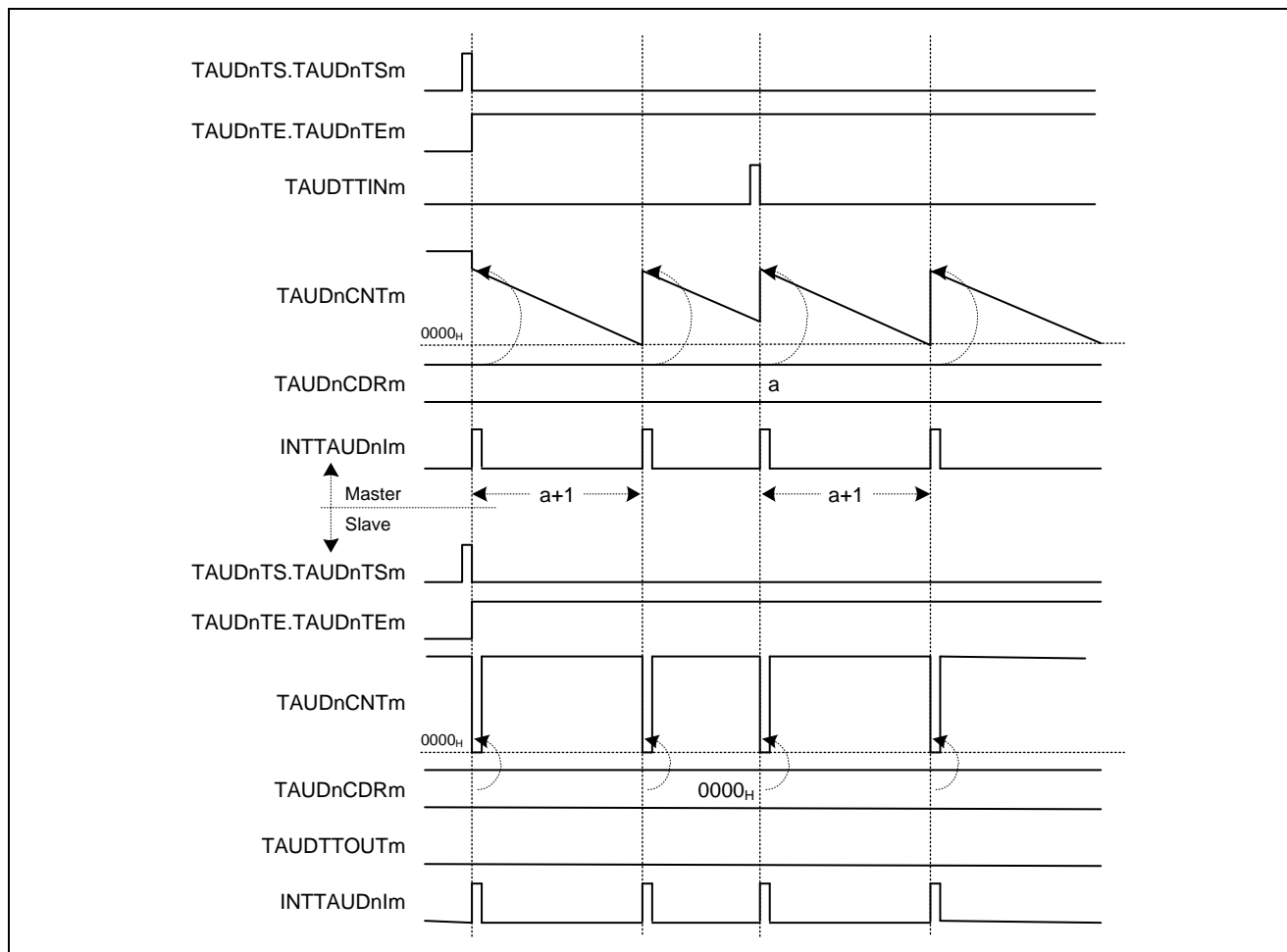
Figure 20.101 TAUDCDRm (Slave) = 0000H, Positive Logic (TAUDTOL.TAUDTOLm (Slave) = 0) Detection of Falling Edges (TAUDCMURm.TAUDTIS[1:0] = 00B)
