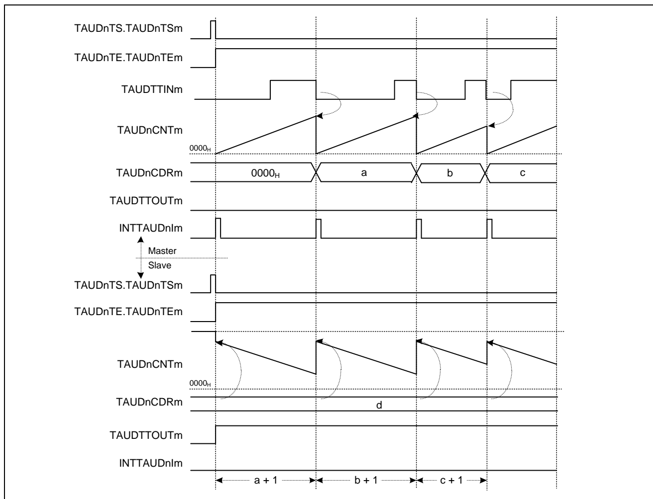
Figure 20.111 TAUDCDRm (Slave) \geq TAUDCDRm (Master) + 1
