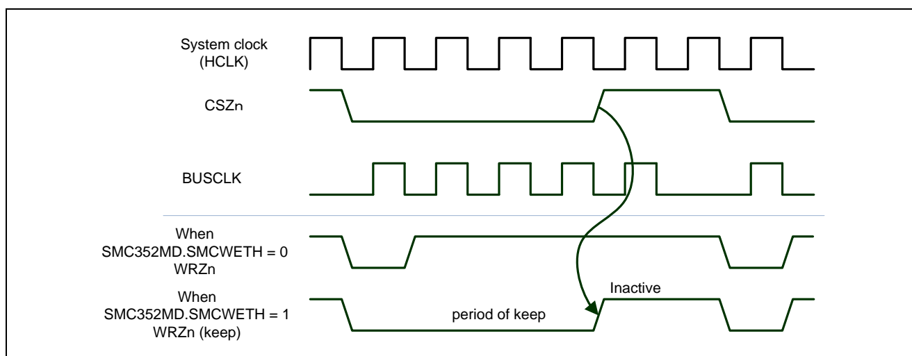
Figure 15.4 Write Enable Signal Operation
