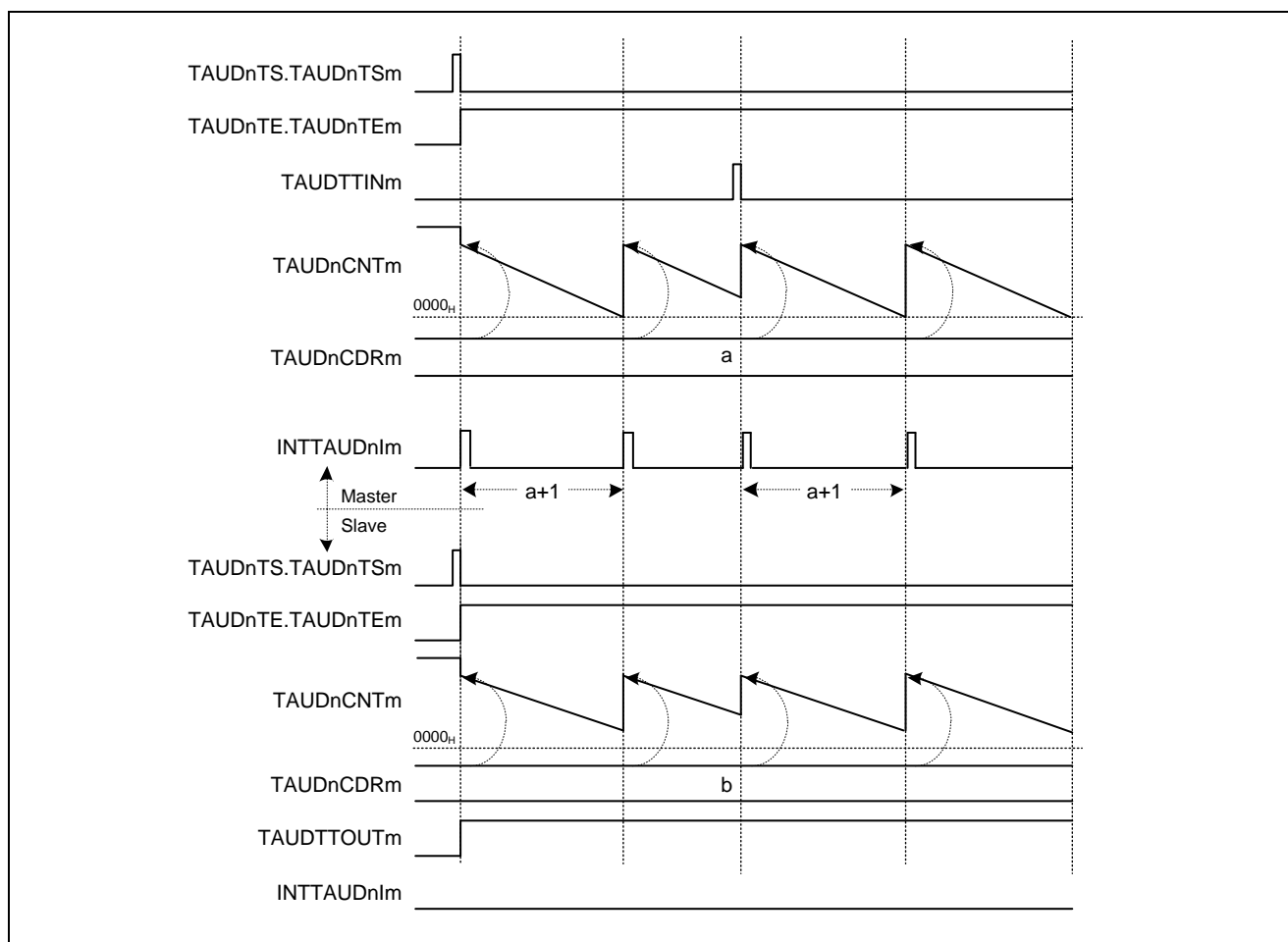
Figure 20.102 TAUDCDRm (Slave) \geq TAUDCDRm (Master) + 1, Positive Logic (TAUDTOL.TAUDTOLm (Slave) = 0) Falling Edge Detection (TAUDCMURm.TIS[1:0] = 00B)
