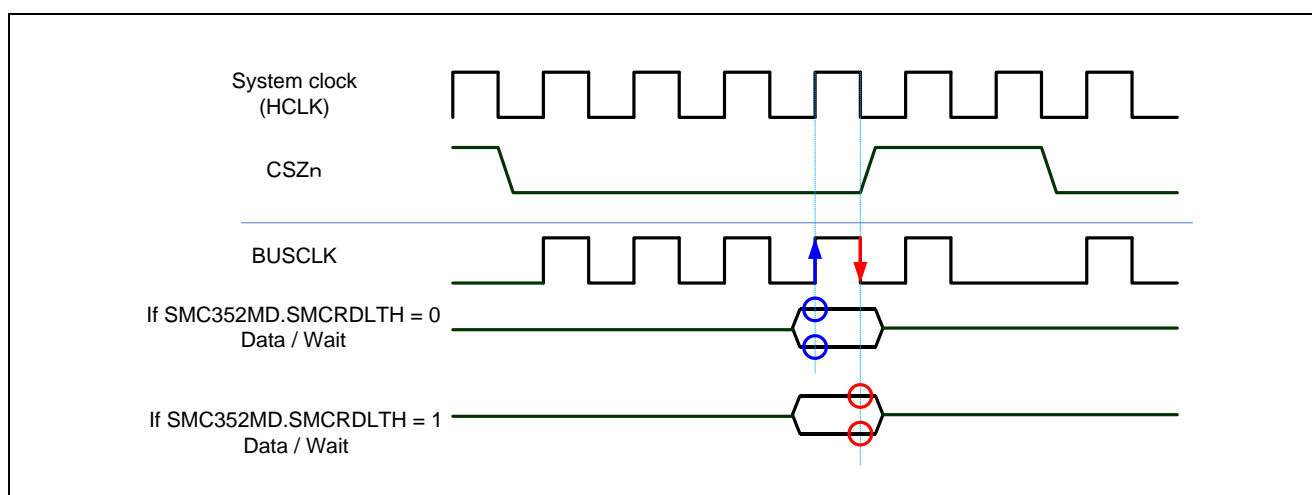
Figure 15.5 Read Data Timing Control
