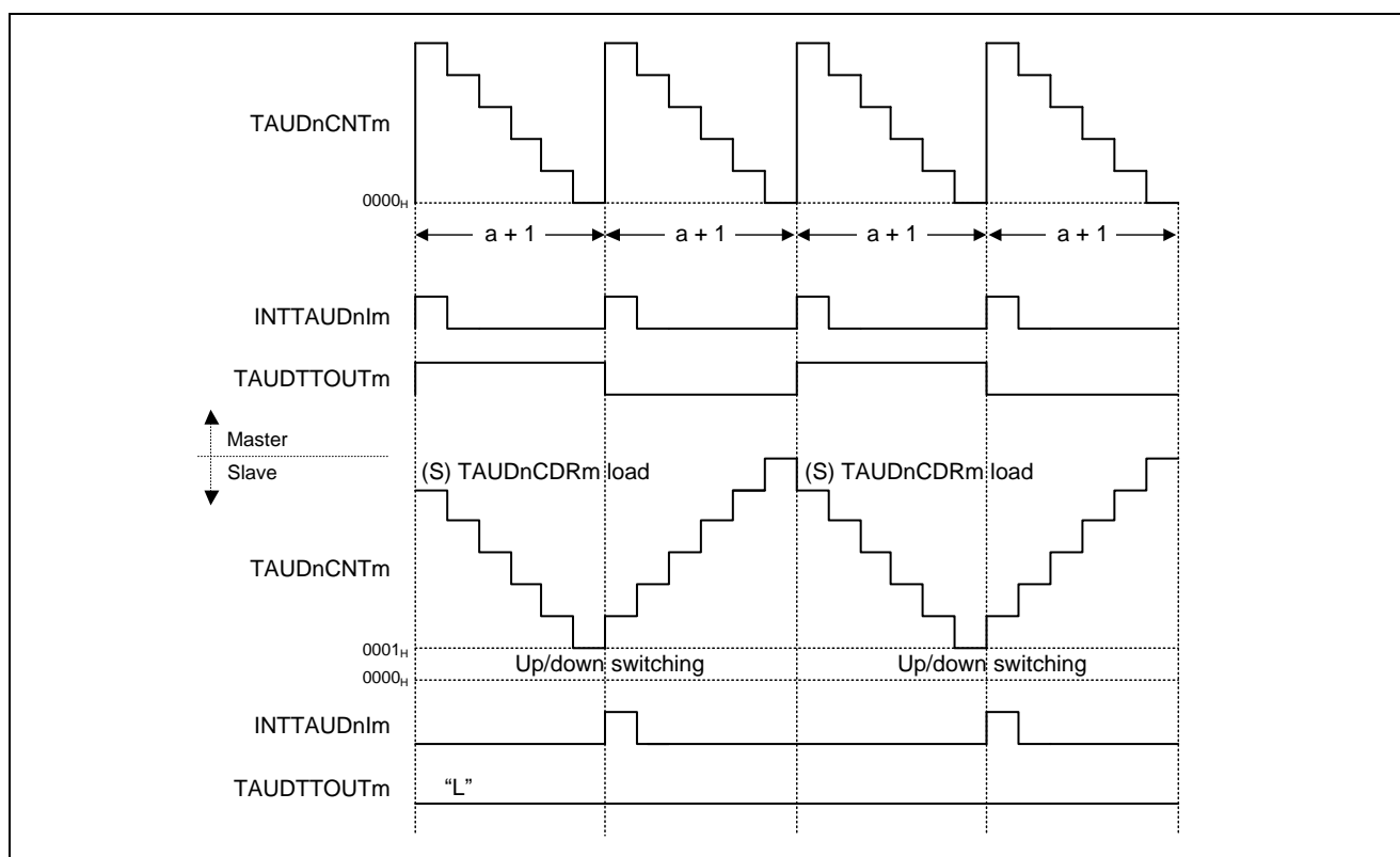
Figure 20.114 TAUDCDRm (Slave) \geq TAUDCDRm (Master) + 1
