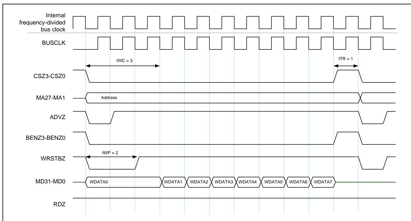
Figure 15.19 Synchronous SRAM, Separate Bus Mode, Burst Write Access (8-Beat), ADVZ Enabled
