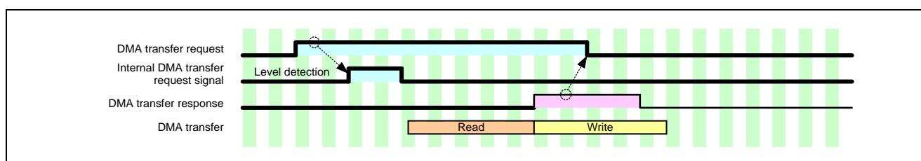
Figure 18.25 Level Detection Mode Operation Example 2
