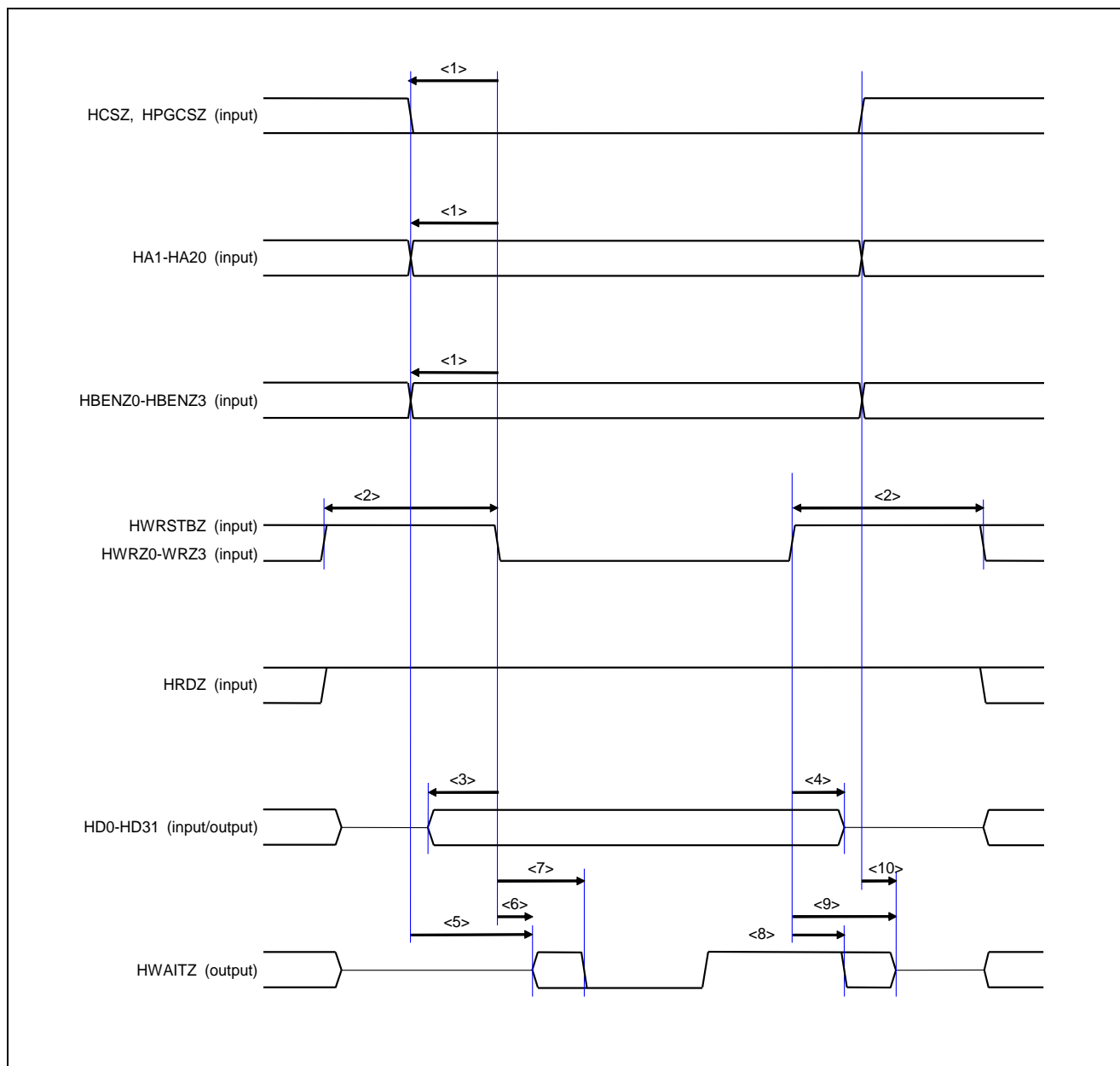
Figure 29.14 External MCU Interface Write Timing (MEMCSEL=L, HIFSUNC=L)
