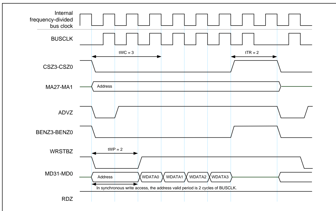
Figure 15.21 Synchronous SRAM, Multiplexed Bus Mode, Burst Write Access (4-Beat), ADVZ Enabled
