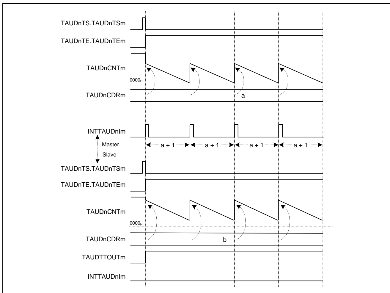
Figure 20.91 TAUDCDRm (Slave) \geq TAUDCDRm (Master) + 1 Positive Logic (TAUDTOL.TAUDTOLm (Slave) = 0)
