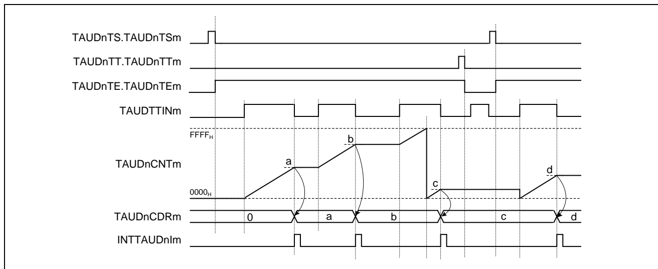
Figure 20.67 Operation Stop and Restart (TAUDCMURm.TAUDTIS[1:0] = 11B)
