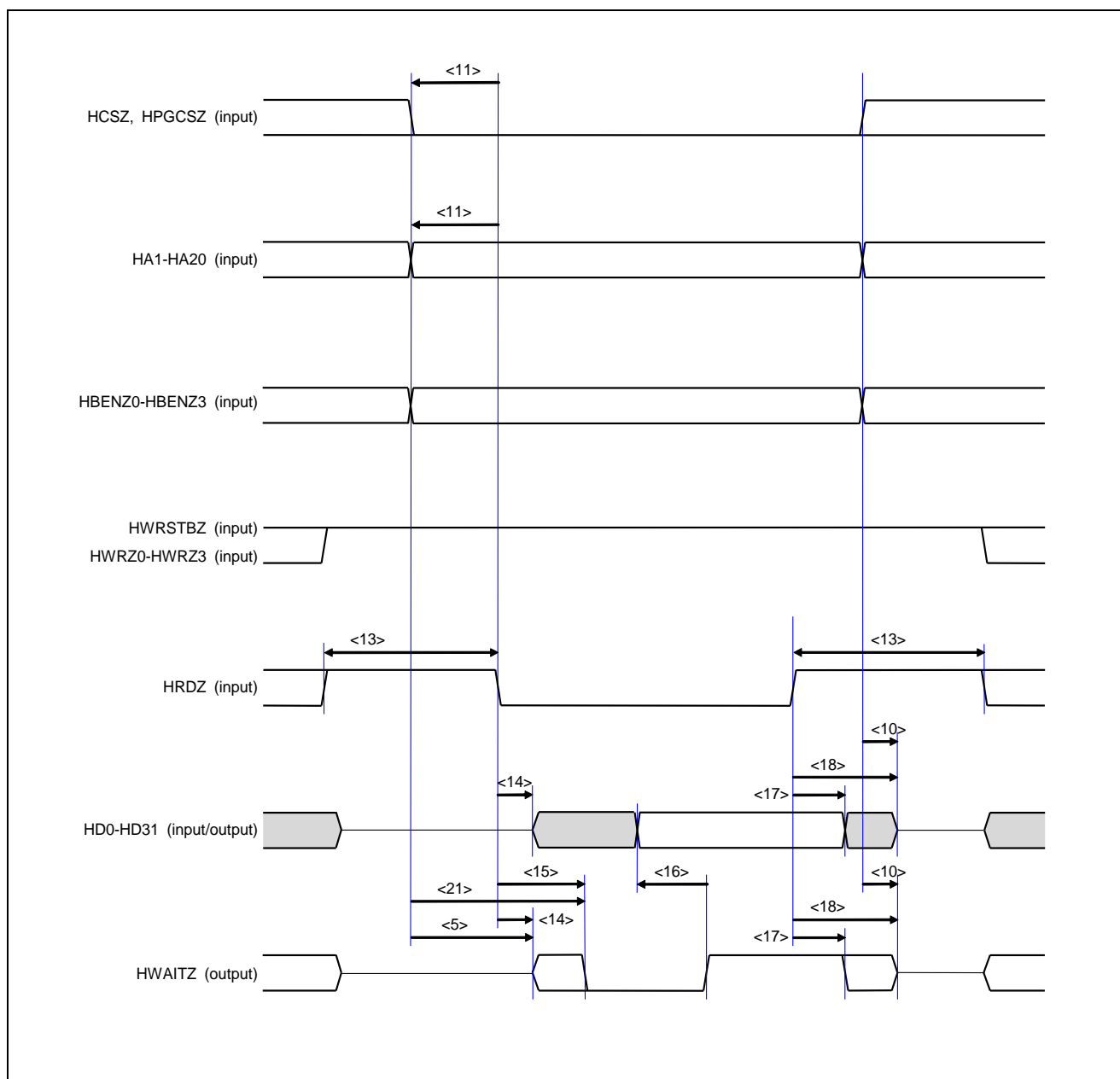
Figure 29.15 External MCU Interface Read Timing (MEMCSEL=L, HIFSYNC=L)
