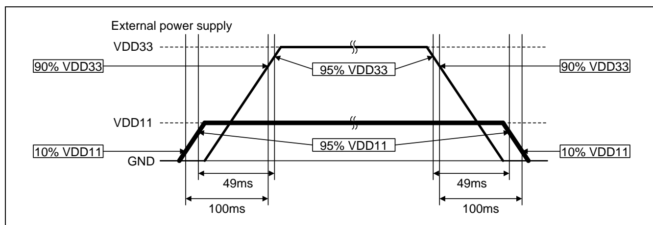
Figure 29.3 Power-On/Off Sequence (with 2.5-V built-in Regulator)
