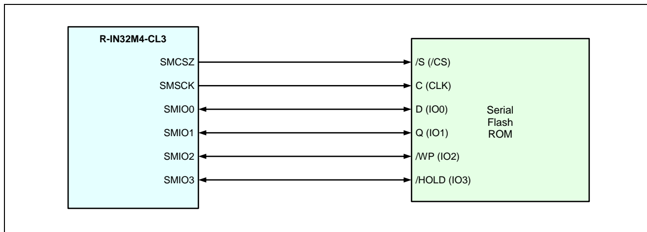
Figure 17.1 Connection with Serial Flash ROM
