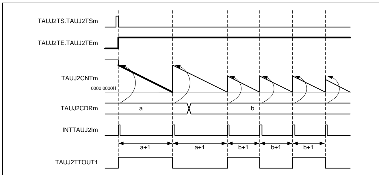
Figure 19.6 General Timing Diagram of Interval Timer
