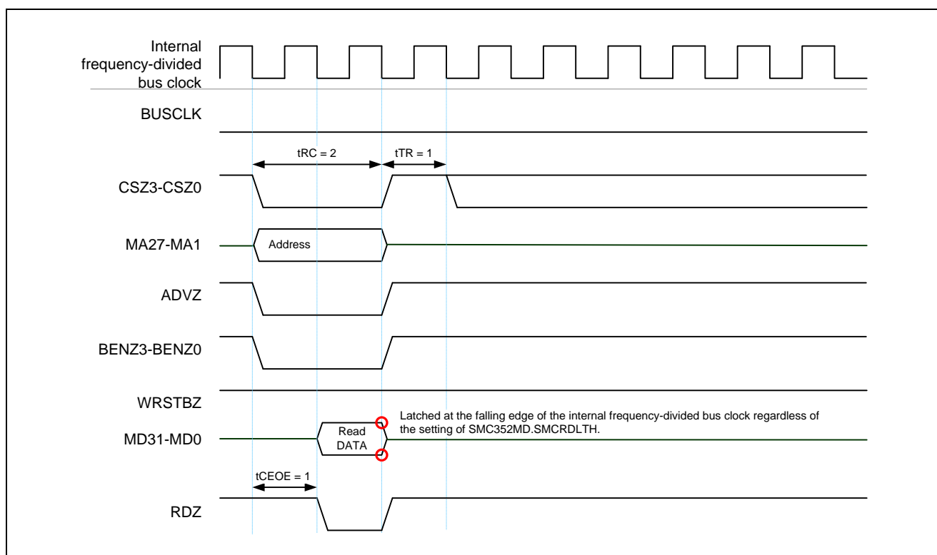
Figure 15.7 Asynchronous SRAM, Separate Bus Mode, Read Access, ADVZ Enabled
