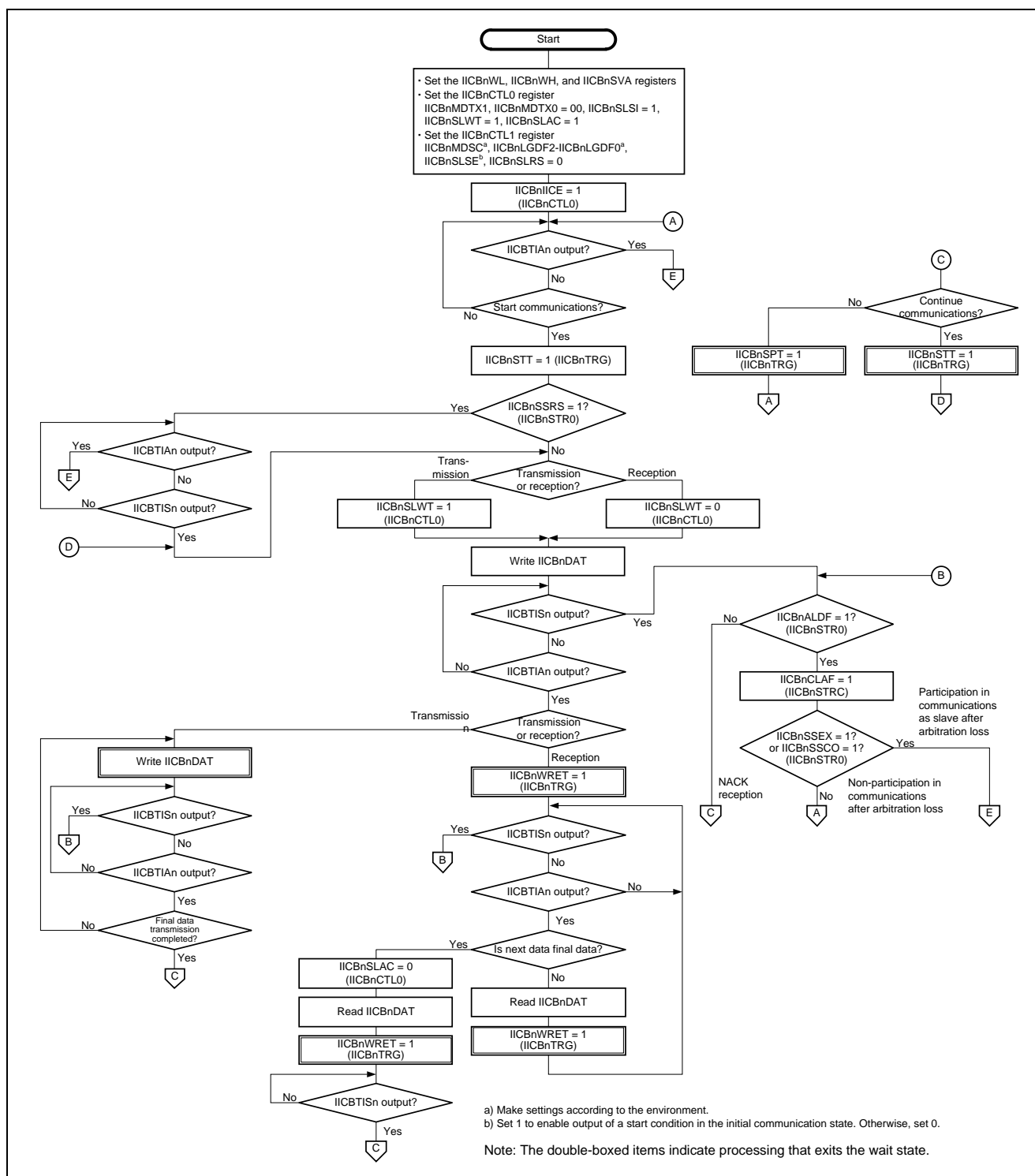
Figure 24.18 Single Transfer Mode Setting Procedure when Communication Reserve Function is Enabled (IICBnCTL1.IICBnSLRS bit = 0) (Multi-Master Environment) (1/2)
