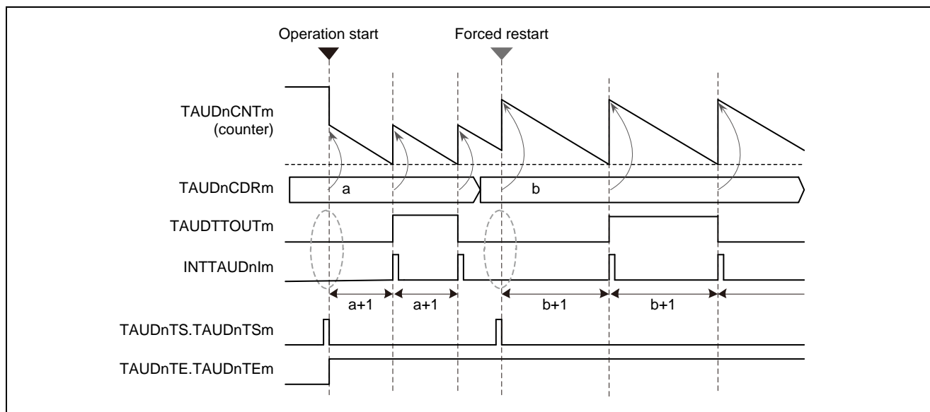
Figure 20.32 Forced Restart Operation (TAUDCMORM.TAUDMD0 = 0)
