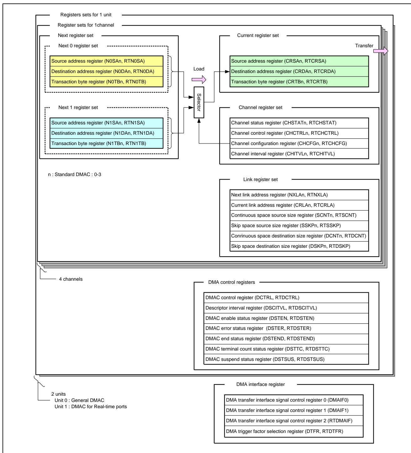
Figure 18.3 Register Block Diagram of DMA
