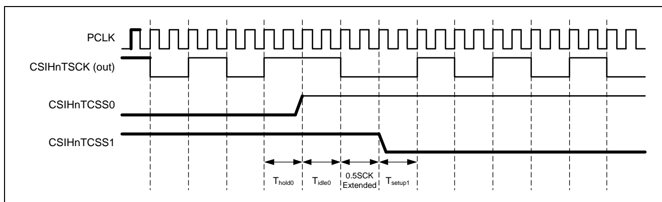
Figure 23.8 Clock Phase Timing (in the case of \text{PCLK}/4 , T_{\text{hold0}} = T_{\text{setup1}} = 0.5 \text{ SCK} , T_{\text{idle0}} = 0.5 \text{ SCK} , \text{CKP0} = 0 ( \text{CSIHnTCSS0} ) \rightarrow \text{CKP1} = 1 ( \text{CSIHnTCSS1} ))
