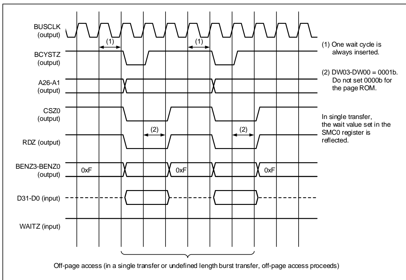
Figure 14.14 Page ROM Read Cycles (Single Transfer)
