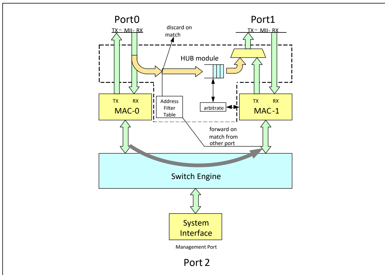
Figure 13.12 Operation of the Hub when Transfer from Port 0 to Port 1 is Enabled
