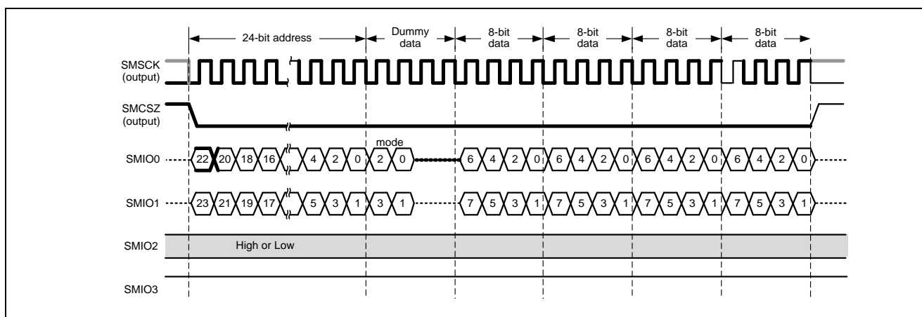
Figure 17.22 Bus Cycles for Fast Read Dual I/O (in Instruction-Omission Mode)
