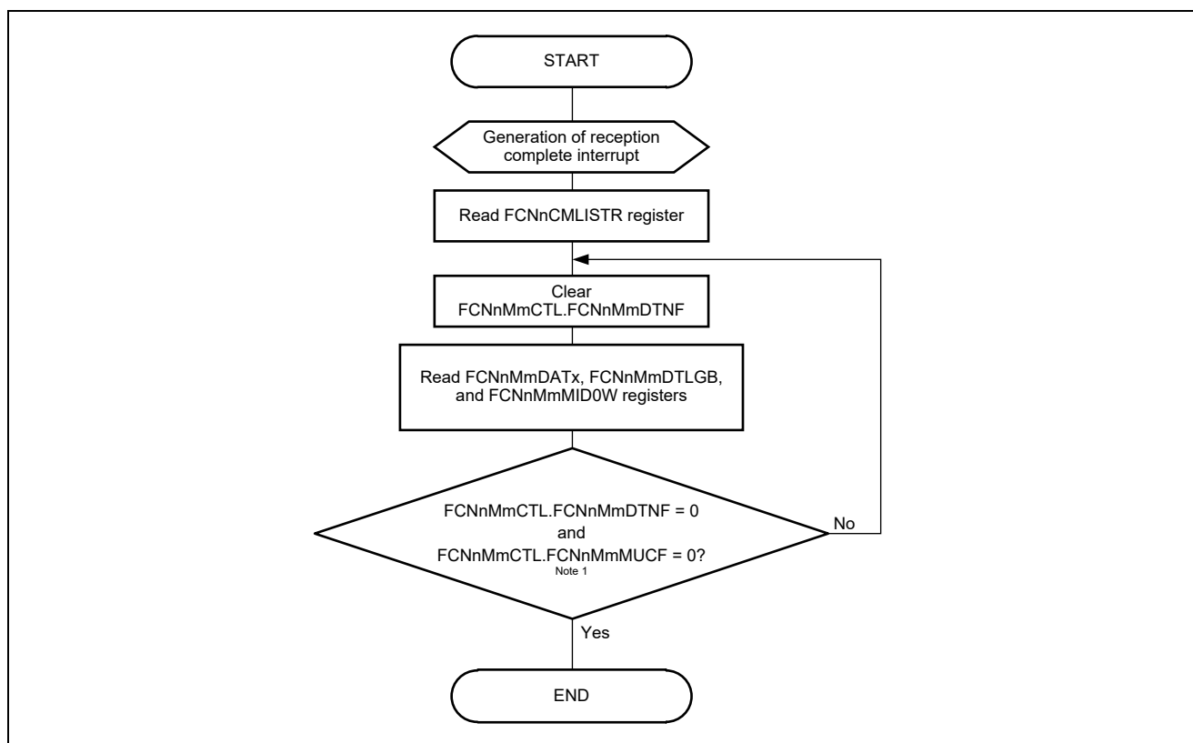
Figure 25.31 Reception via Interrupt (Using FCNnCMILSTR Register)
