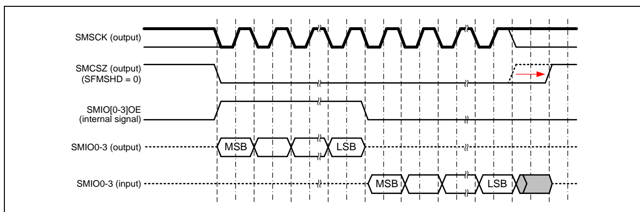
Figure 17.9 SMCSZ Signal Hold Time Adjustment by Using the SFMSSHD Bit
