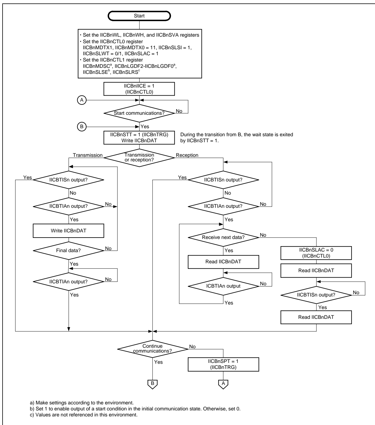
Figure 24.16 Master Operation Setting Procedure during Continuous Transfer Mode (Single Master Environment)
