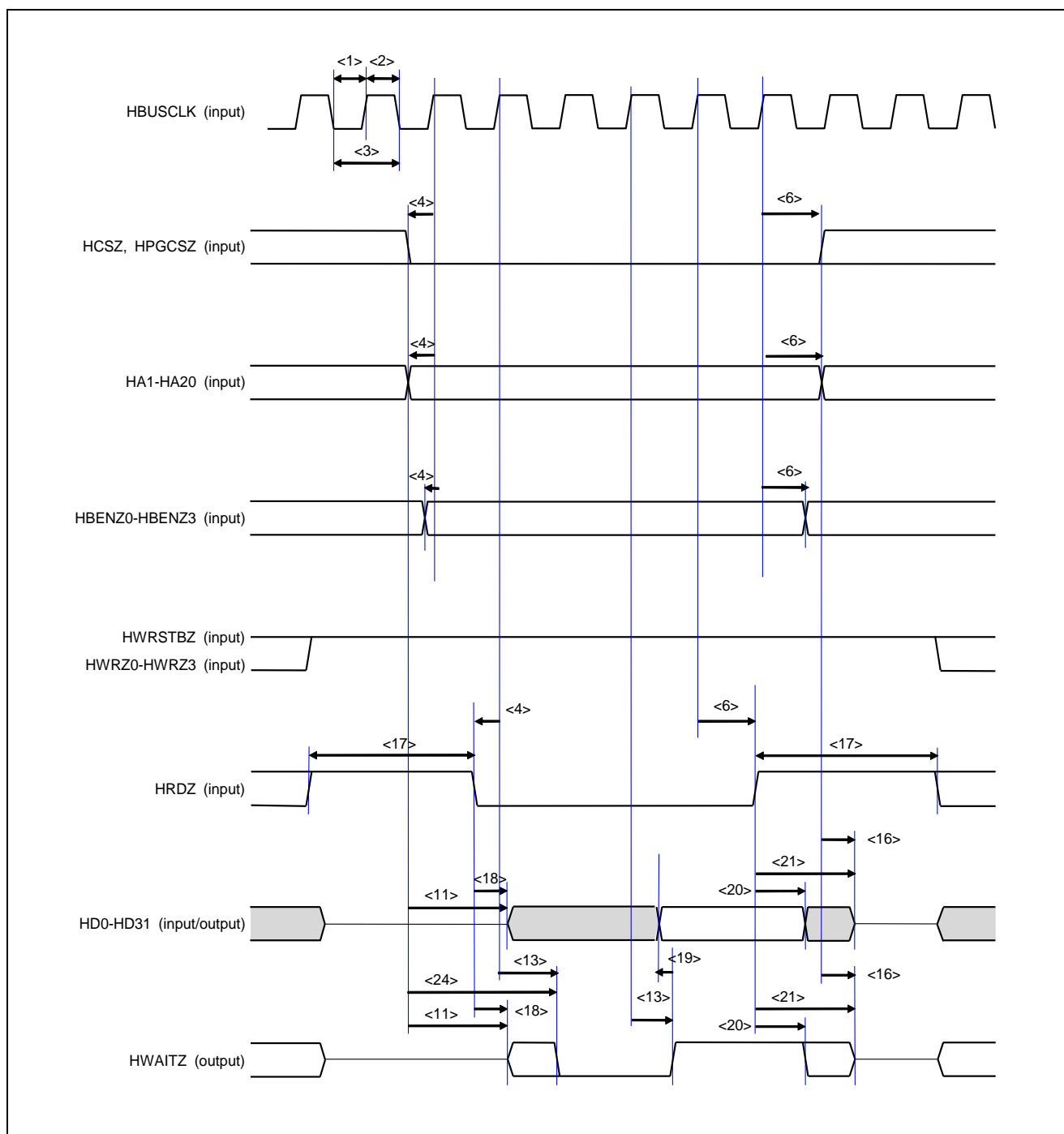
Figure 29.12 External MCU Interface Read Timing (MEMCSEL=L, HIFSYNC=H)
