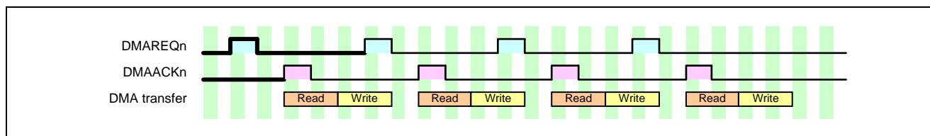
Figure 18.36 When the Transfer Size of the Destination Is Equal to That of the Source
