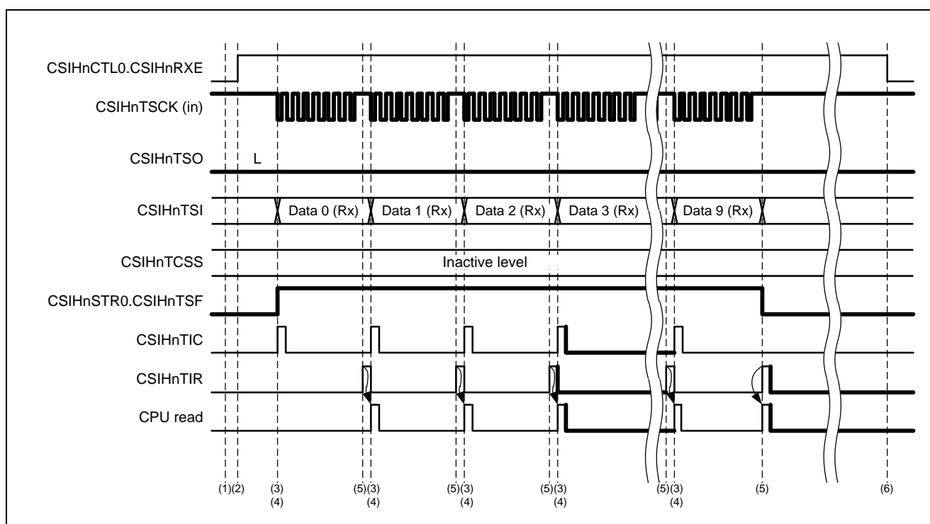
Figure 23.41 Direct Access Mode (for Reception in Slave Mode, and when Job Mode is Disabled)
