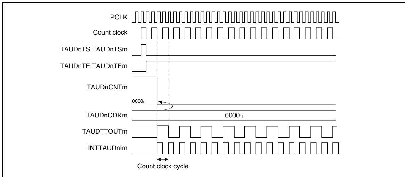
Figure 20.28 \text{TAUDCDRm} = 0000\text{H} , Count Clock = \text{PCLK}/2
