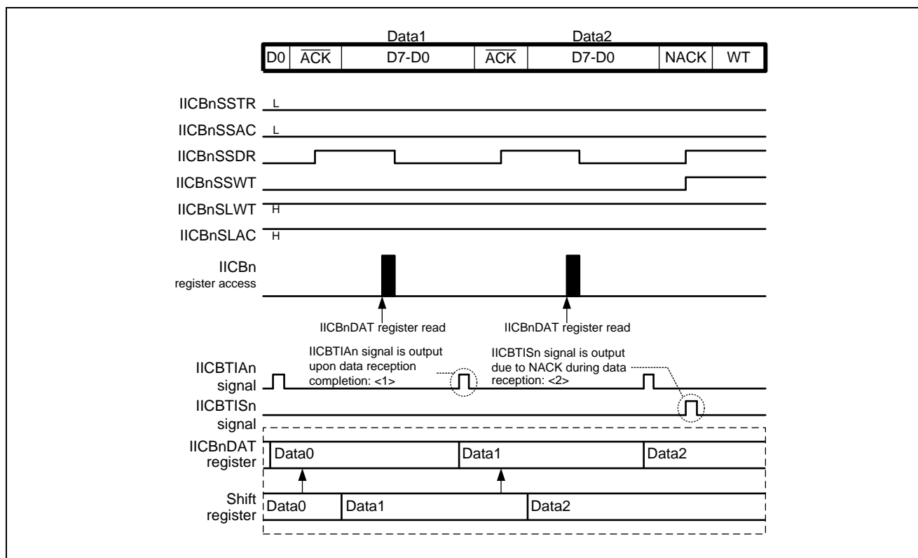
Figure 24.12 IICBTIA Signal Output Timing (Reception in Continuous Transfer Mode)
