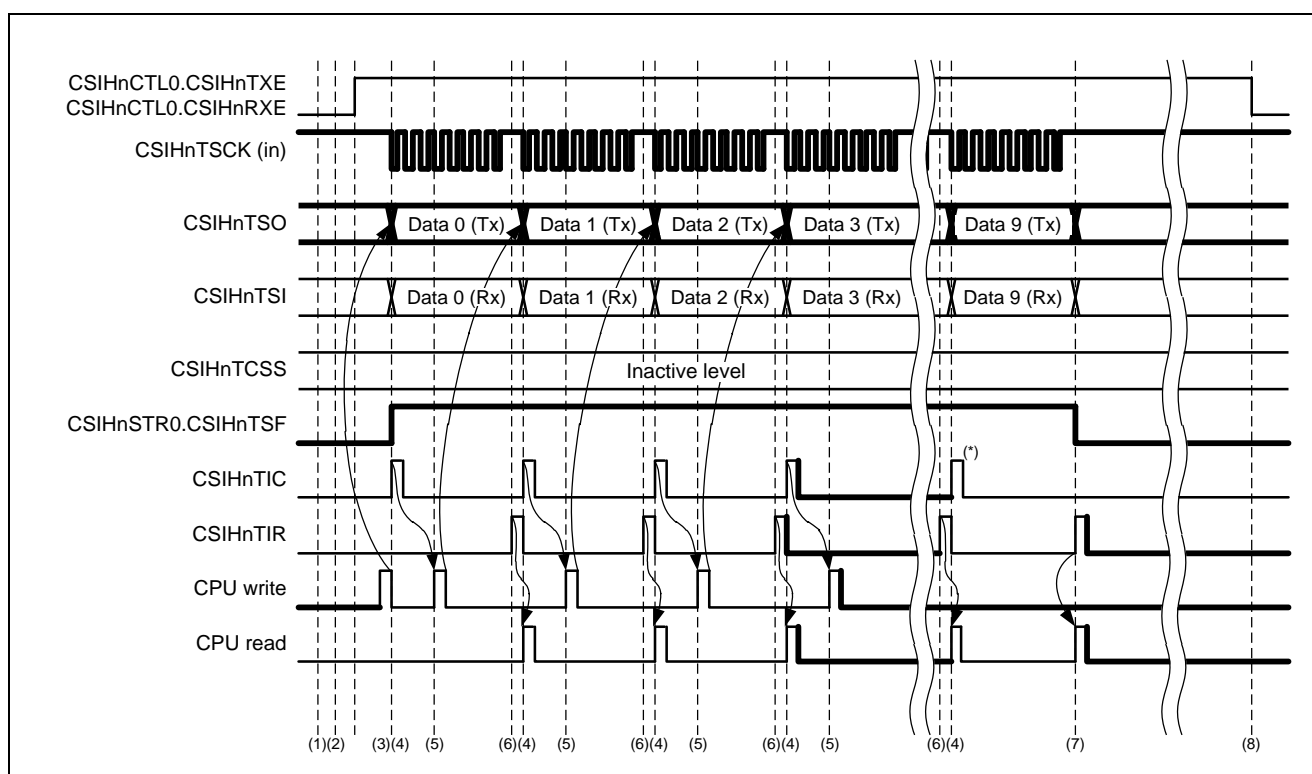
Figure 23.40 Direct Access Mode (for Transmission/Reception in Slave Mode, and when Job Mode is Disabled)
