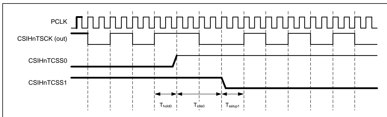
Figure 23.10 Clock Phase Timing (in the case of PCLK/4, T_{hold0} = T_{setup1} = 0.5 \text{ SCK} , T_{idle0} = 0.5 \text{ SCK} , CKP0 = 0 (CSIHnTCSS0) \rightarrow CKP1 = 0 (CSIHnTCSS1))
