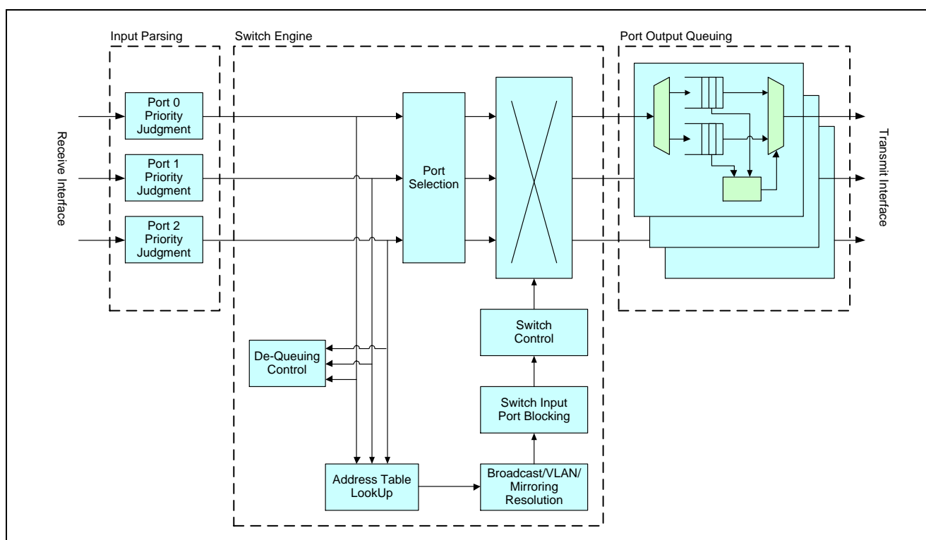
Figure 13.2 Switching Engine Overview
