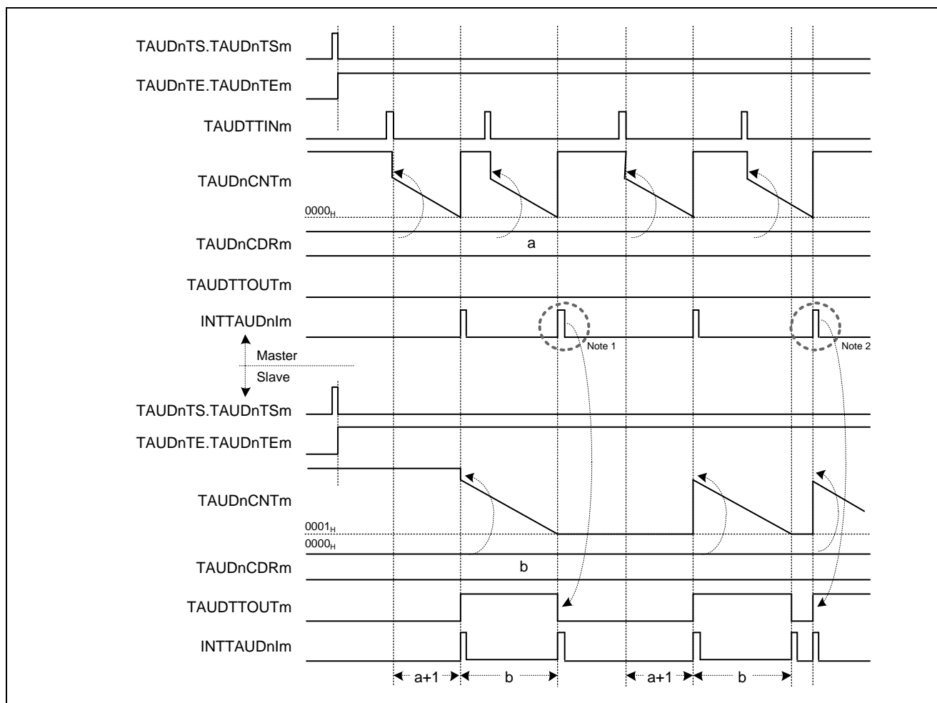
Figure 20.98 TAUDTTINm input interval \leq Delay Time + Pulse Width + 1
