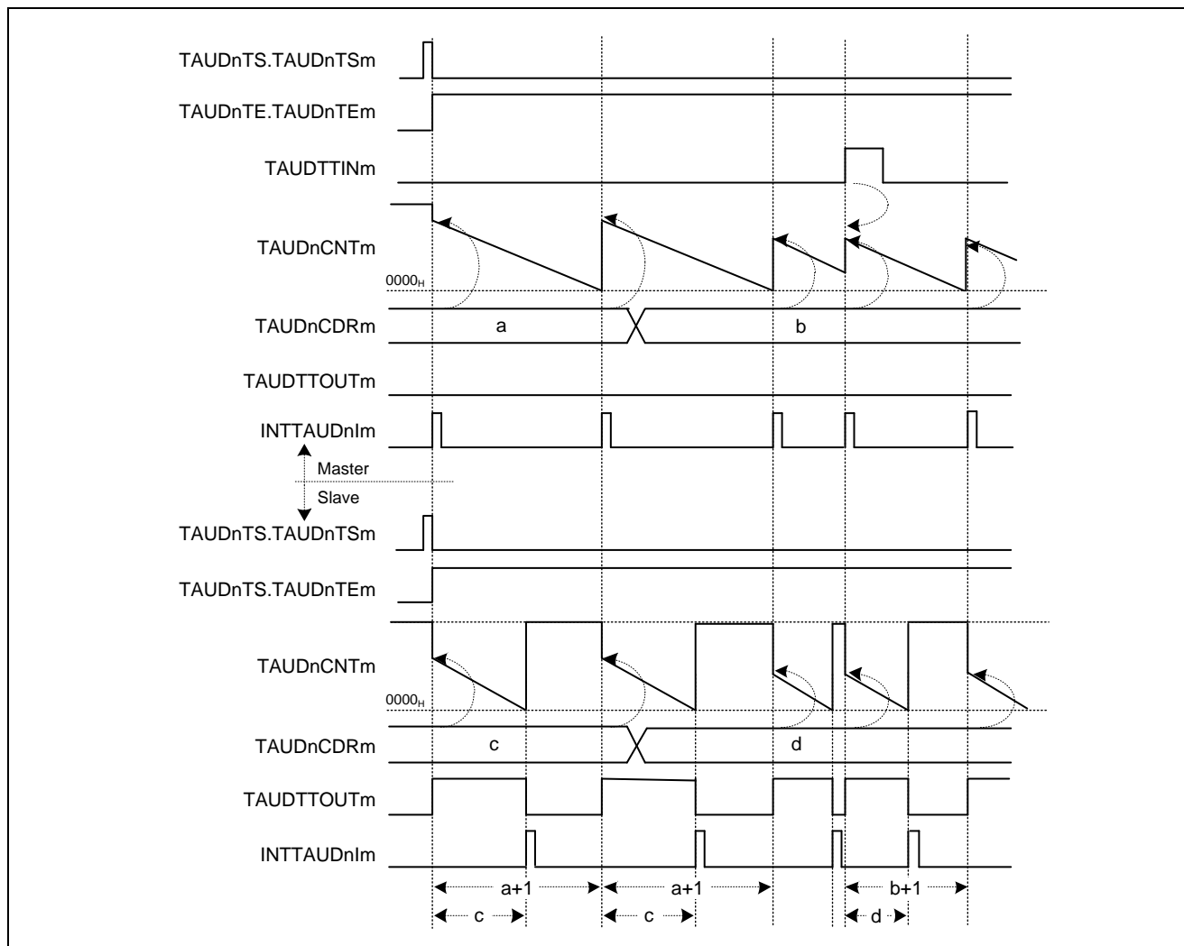
Figure 20.100 General Timing Diagram for Trigger Start PWM Output
