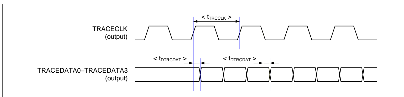
Figure 29.29 Trace Interface
