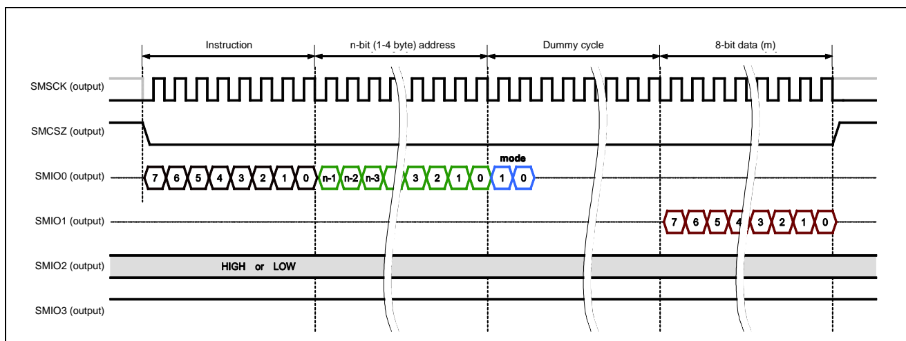
Figure 17.2 Example 1 of Extended SPI Protocol (Fast Read)
