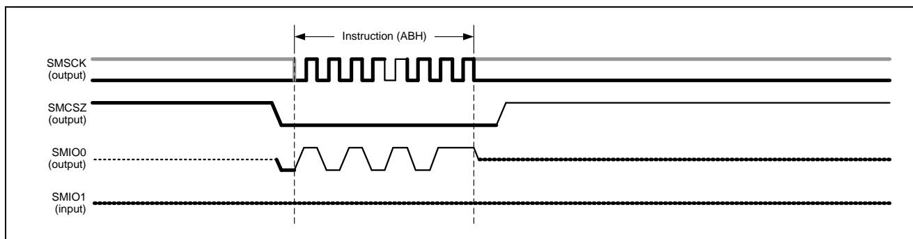
Figure 17.27 Bus Cycles for Release from Deep Power-Down
