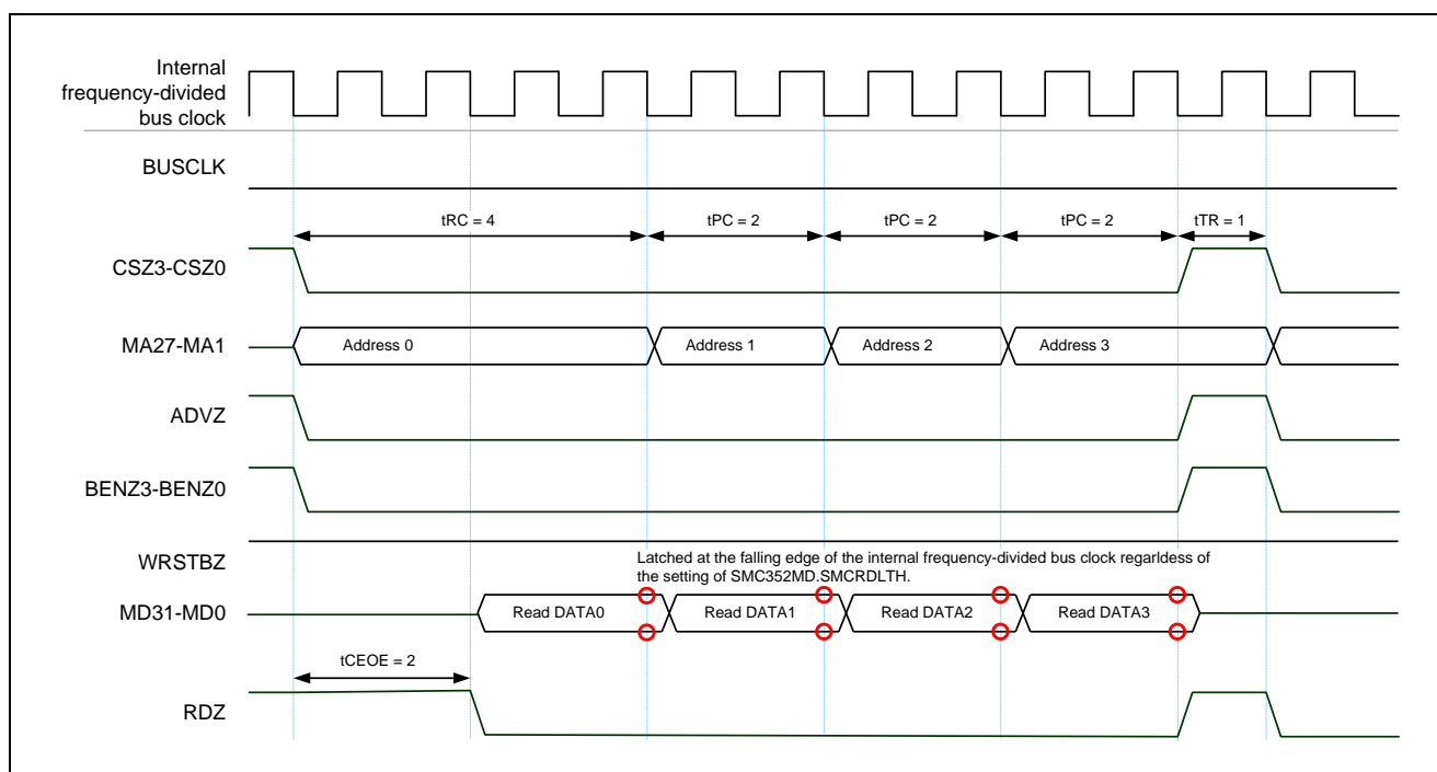
Figure 15.9 Asynchronous Page ROM, Separate Bus Mode, Read Access, ADVZ Enabled
