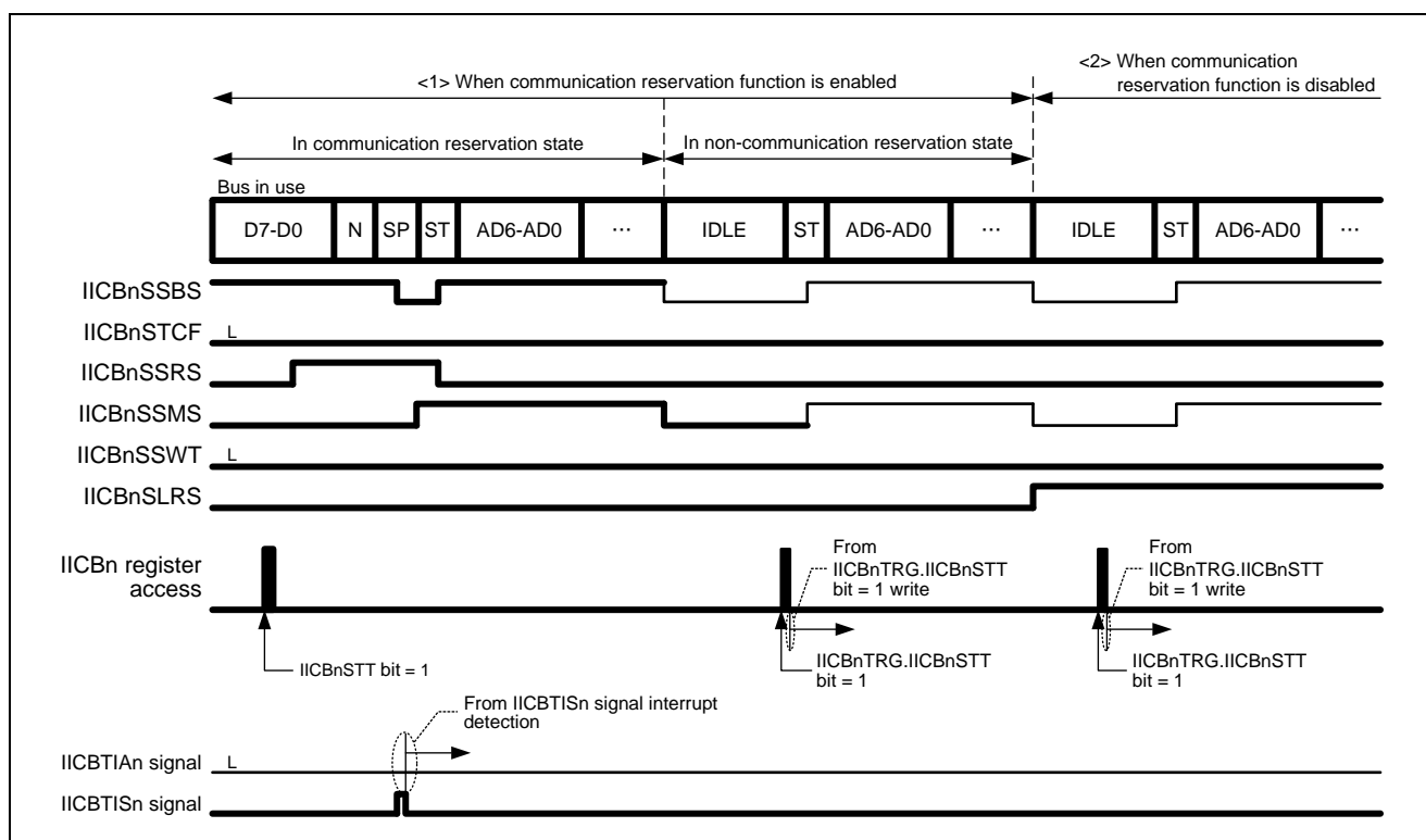
Figure 24.11 Valid Times to Write to IICBnDAT Register
