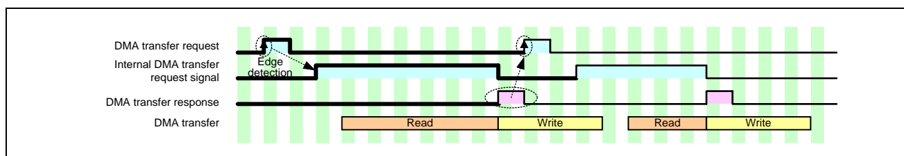
Figure 18.27 Pulse Output Mode Operation Example 2
