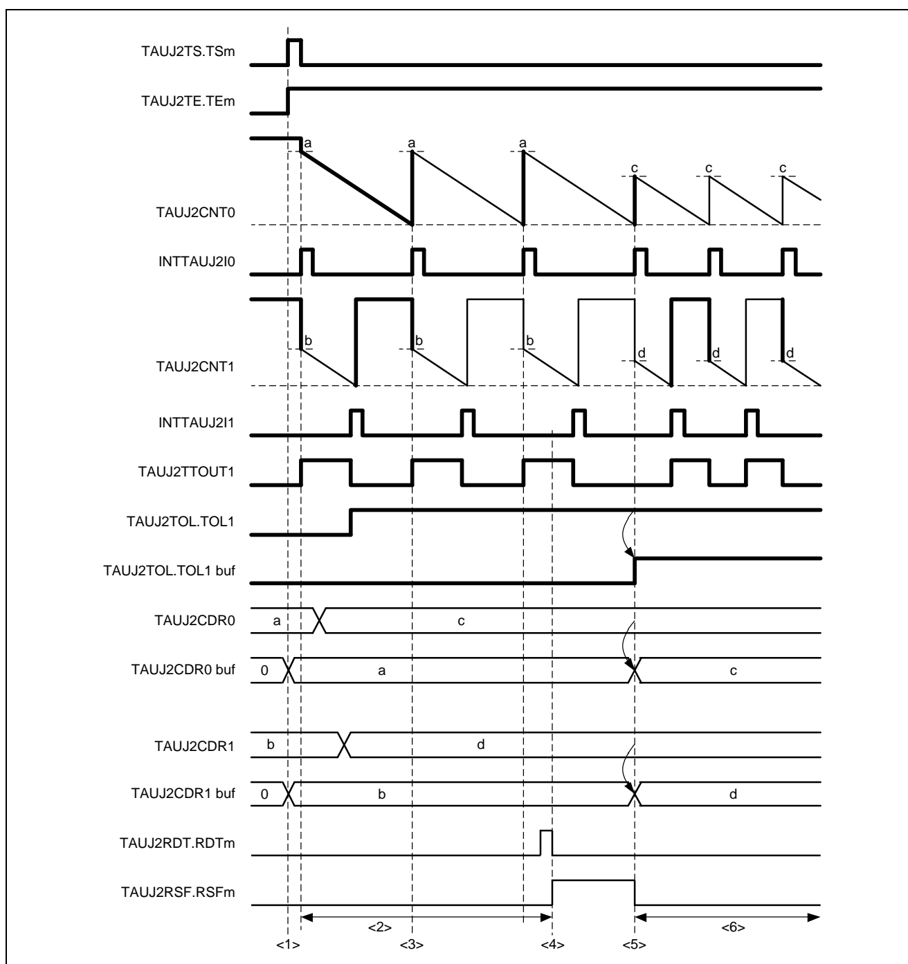
Figure 19.41 Simultaneous Reloading of the Master Channel
