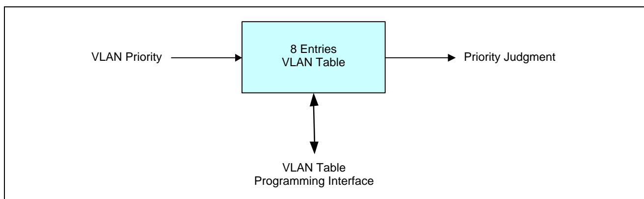
Figure 13.3 VLAN Priority Table Overview
