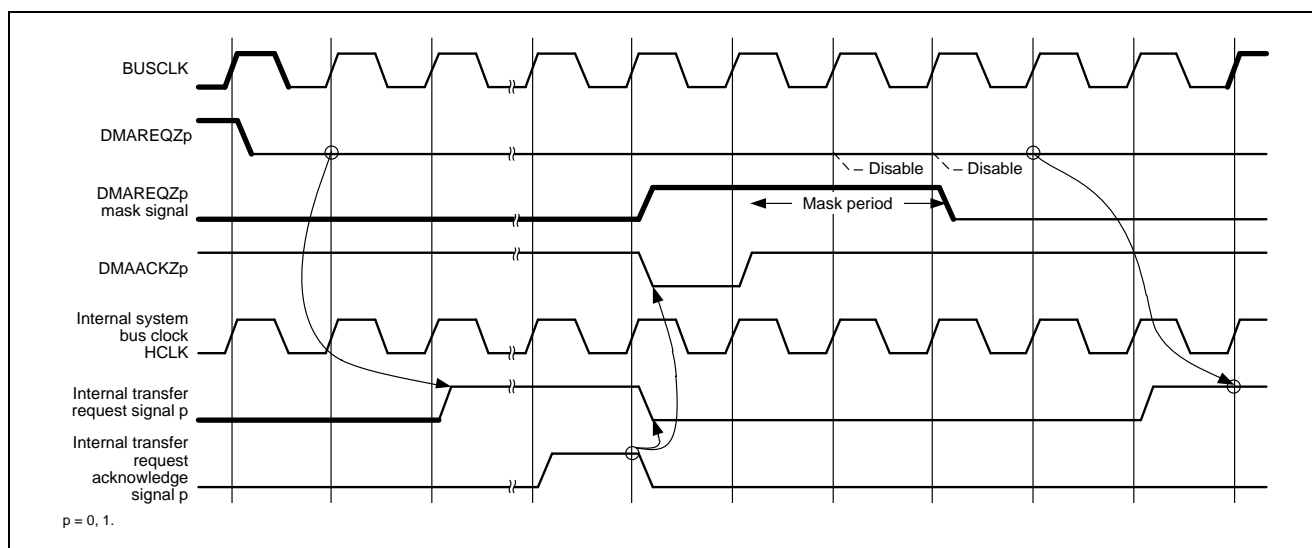
Figure 18.10 DMA Pin Signals and Internal Signals (3) (DMAIFCp = 8000 0200H)
