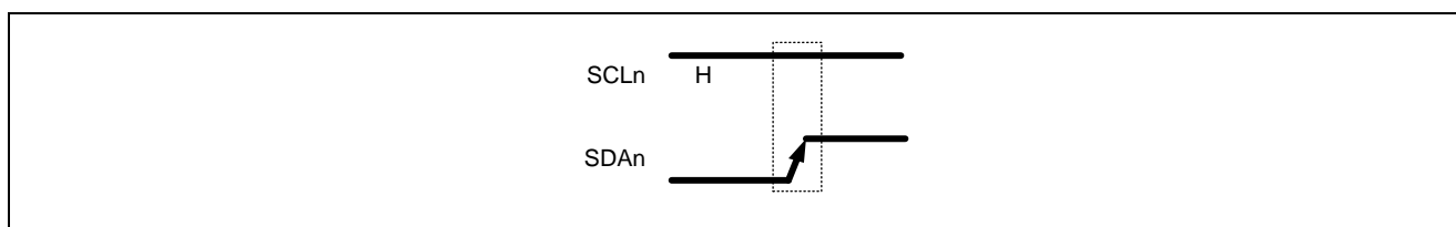
Figure 24.8 Stop Condition
