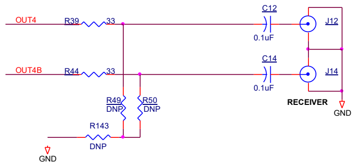
Figure 11. Output Termination Options
