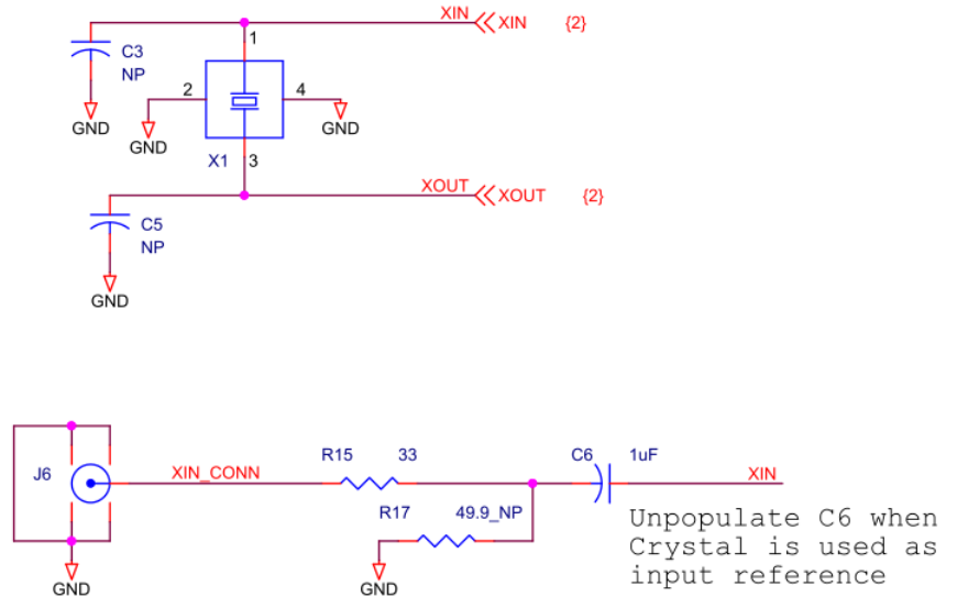
Figure 6. Crystal Circuit
