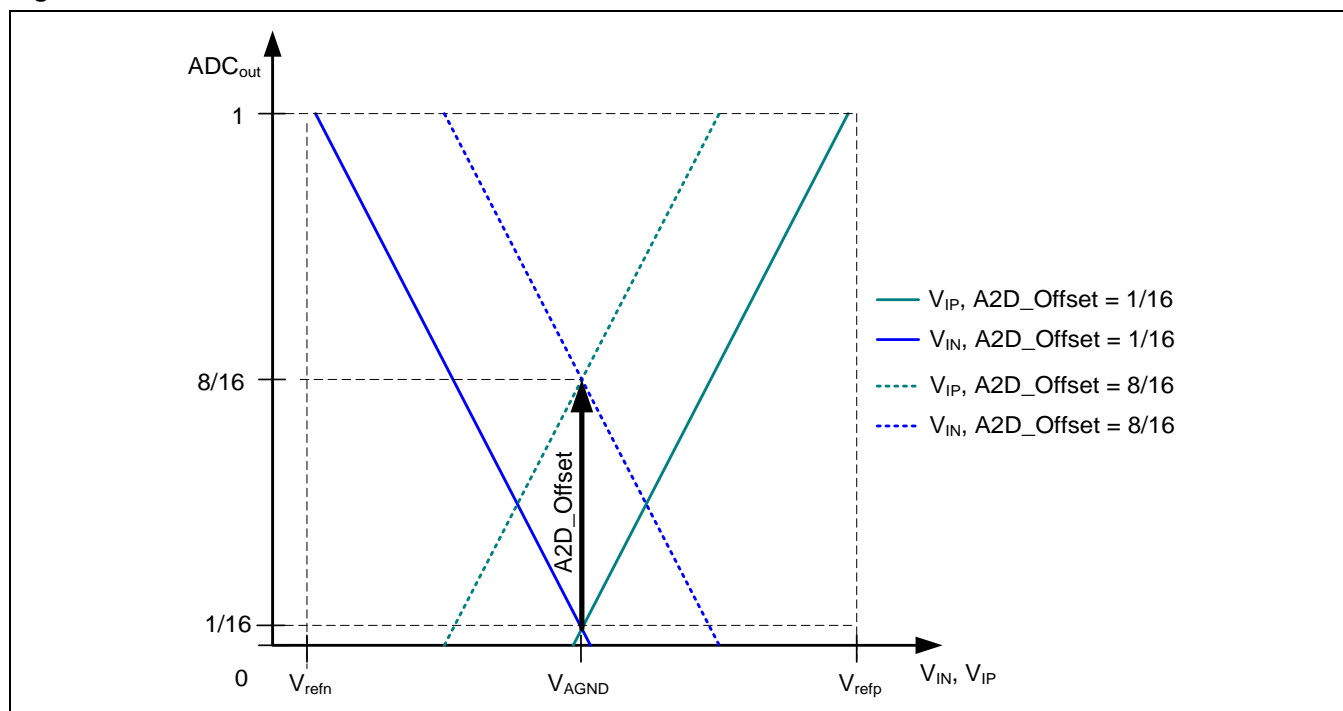
Figure 2.2 ADC Offset
