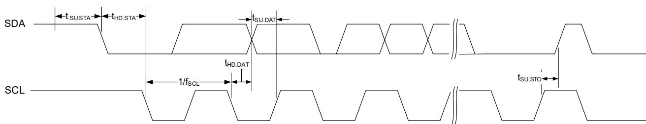
Figure 9. I 2 C Timing Diagram
