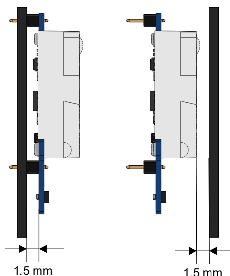
Figure 5. Sensor Placement Recommendation
