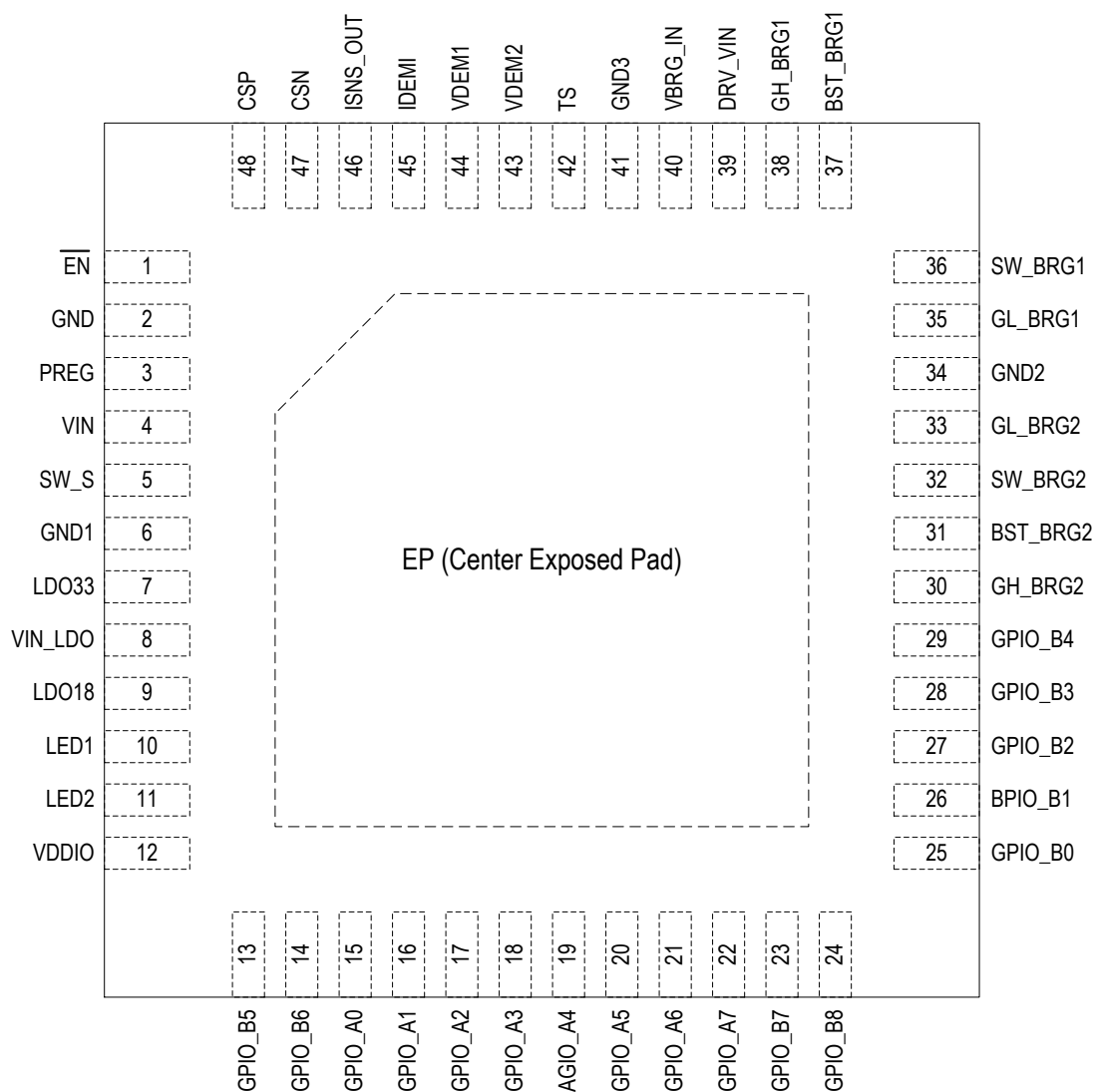
Figure 1. Pin Assignments
