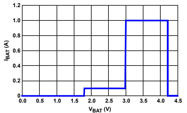
FIGURE 25. BATTERY VOLTAGE vs CHARGE CURRENT (CC MODE)
