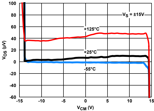
FIGURE 17. INPUT V_{OS} vs INPUT COMMON-MODE VOLTAGE, V_S = \pm 15
