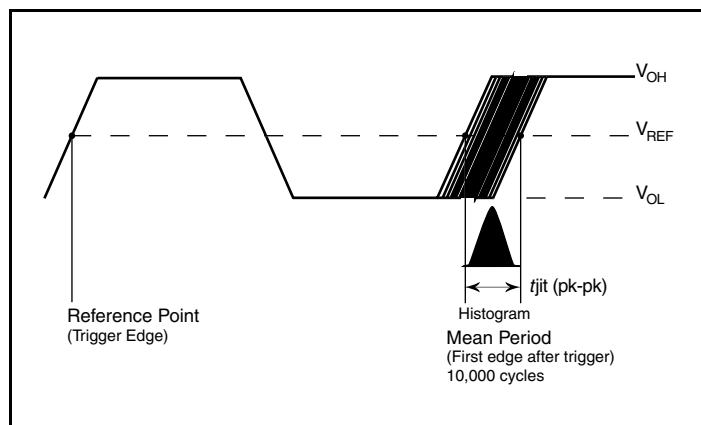
Period Jitter, Peak-to-Peak
