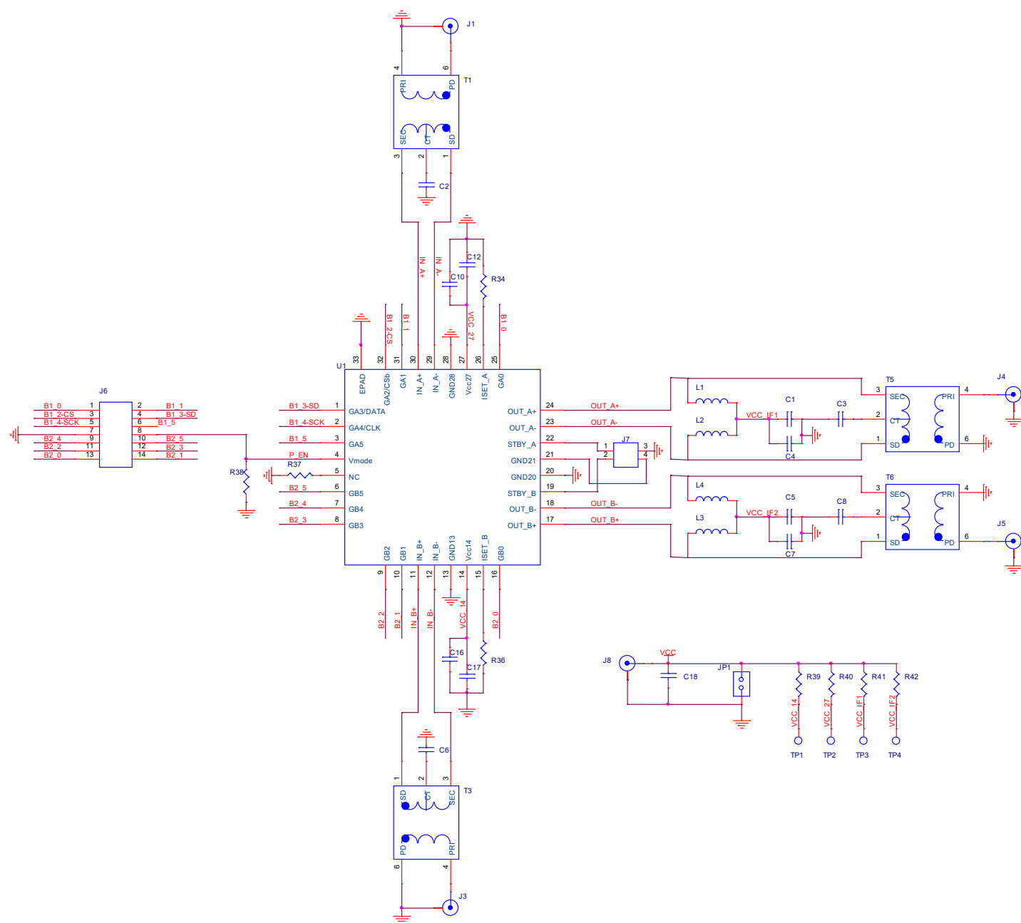
Figure 46. Electrical Schematic
