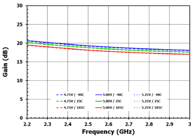
Figure 2. Gain
