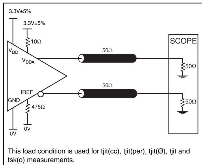
3.3V HCSL Output Load AC Test Circuit 2
