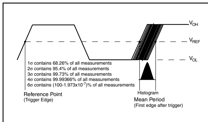
Period Jitter
