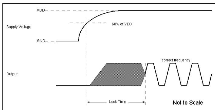
PLL Lock Time
