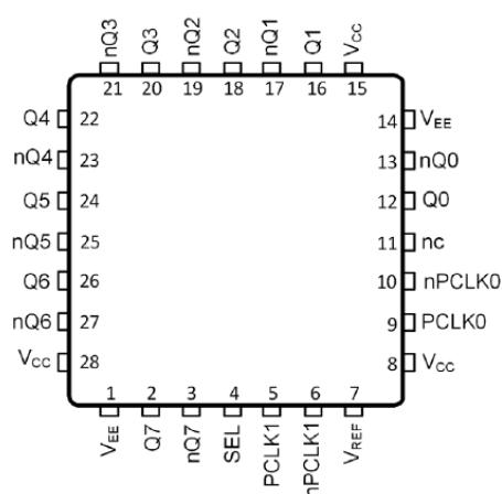
8SLVP1208 28-VFQFPN Top View
