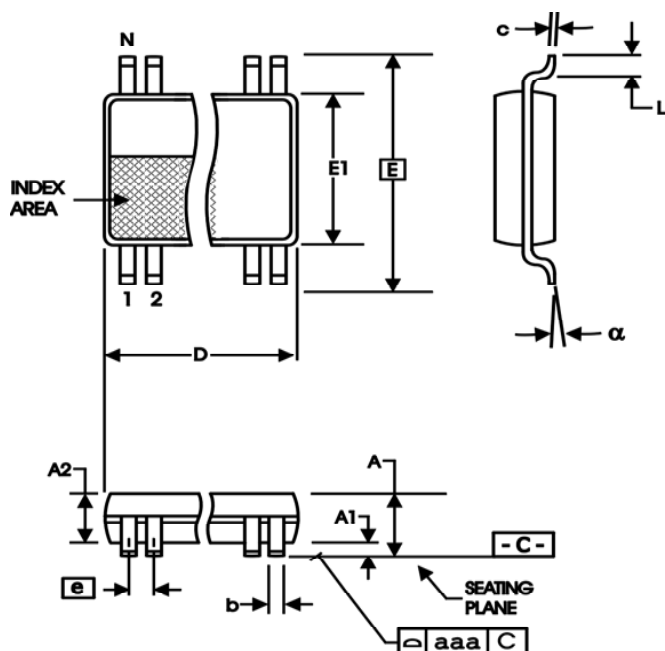
Package Outline - G Suffix for 16 Lead TSSOP
