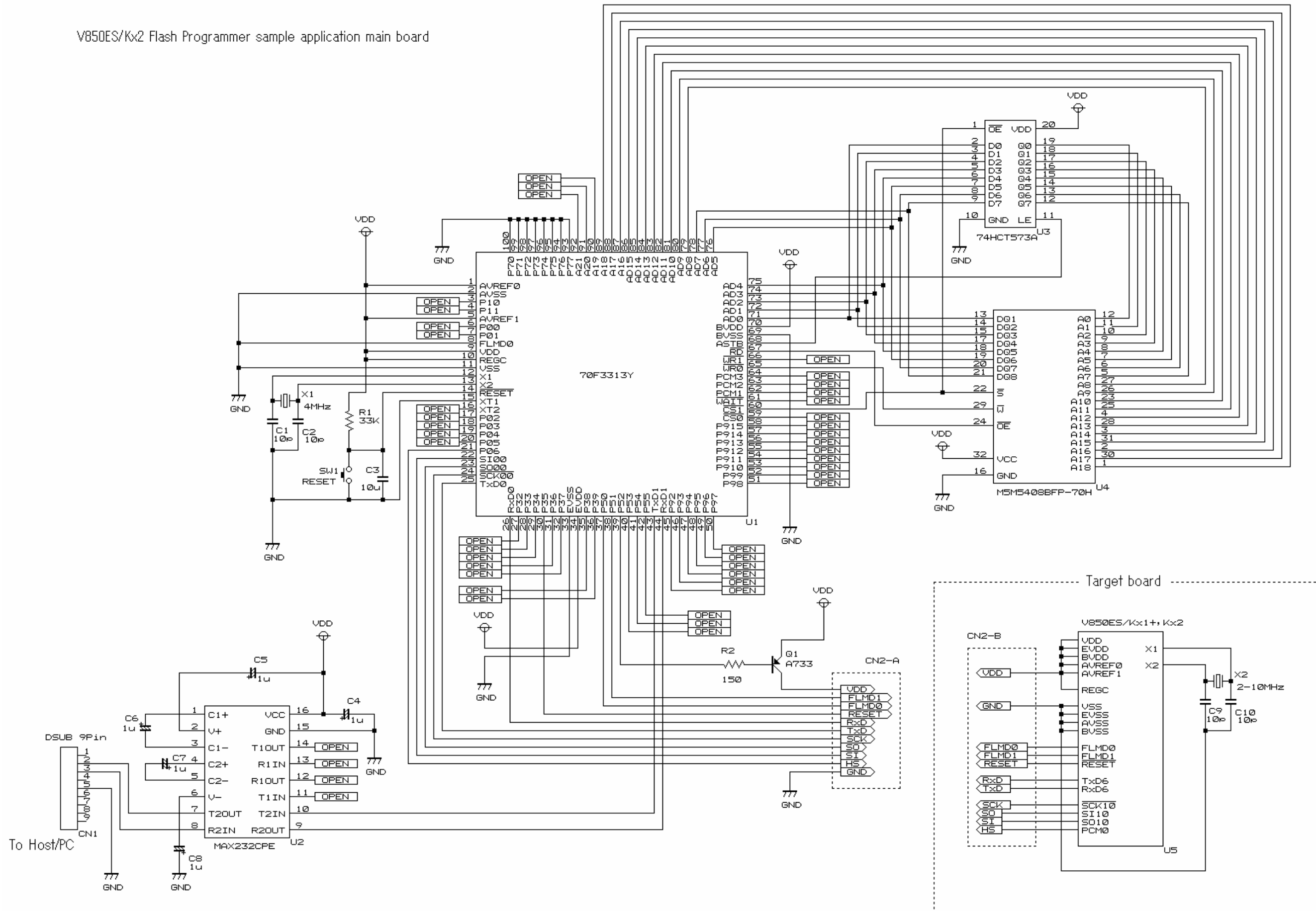
Figure A-1. Reference Circuit Diagram of Programmer and V850ES/Kx2
