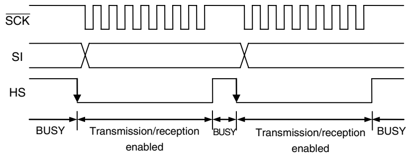
Figure 2-7. Timing Chart of CSI + HS Communication
