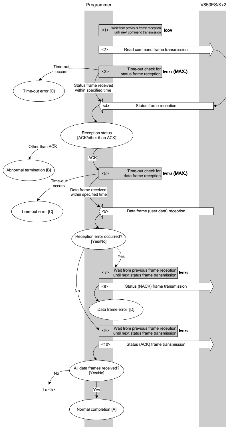
Read command processing sequence
