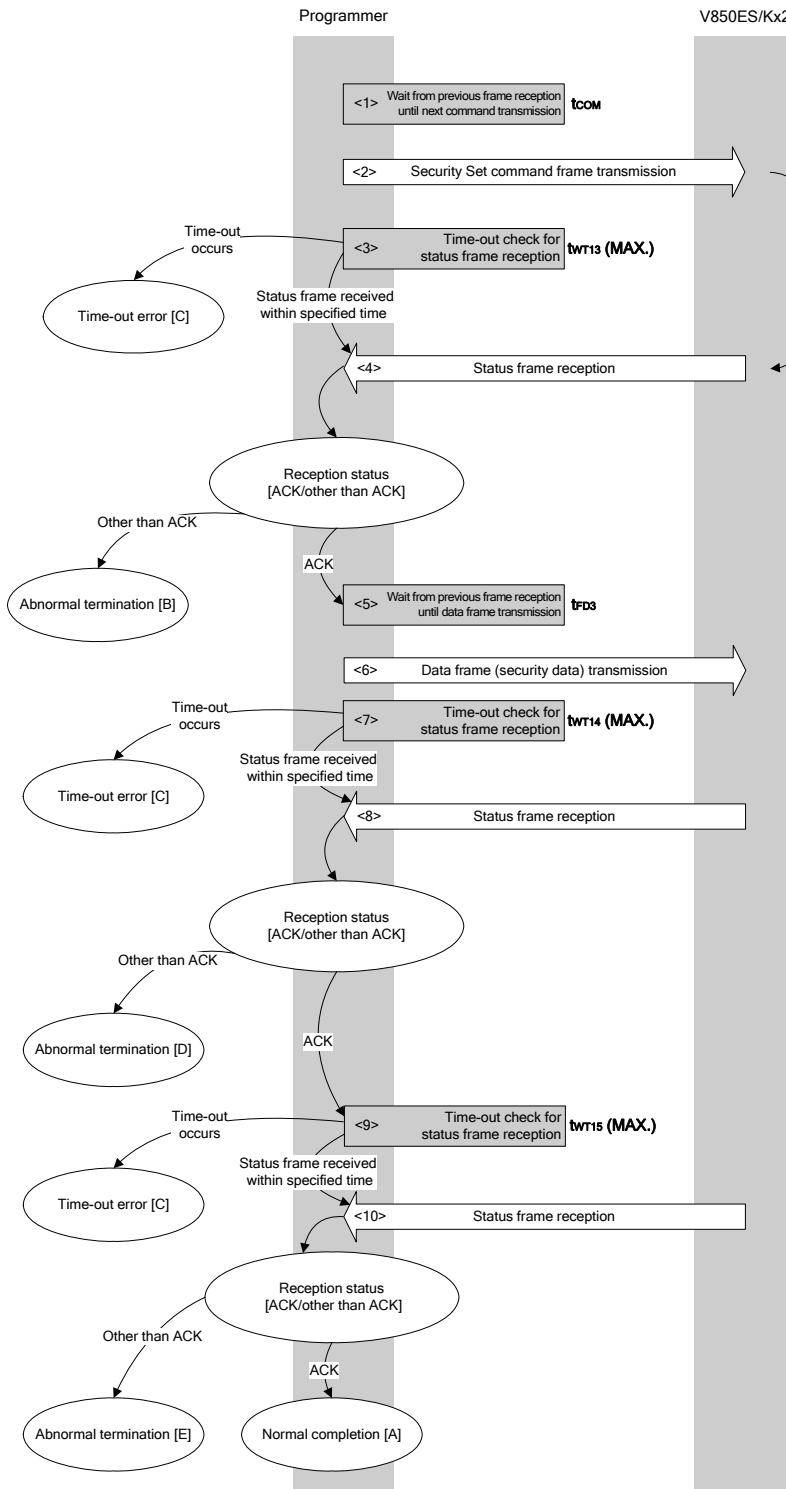
Security Set command processing sequence
