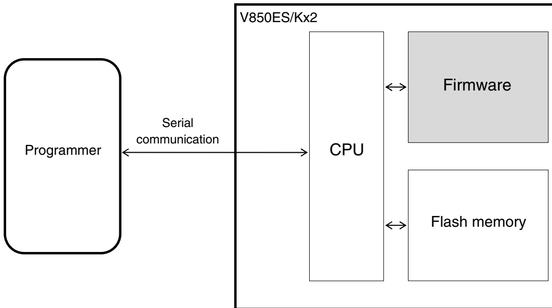
Figure 1-1. System Outline of Flash Memory Programming in V850ES/Kx2
