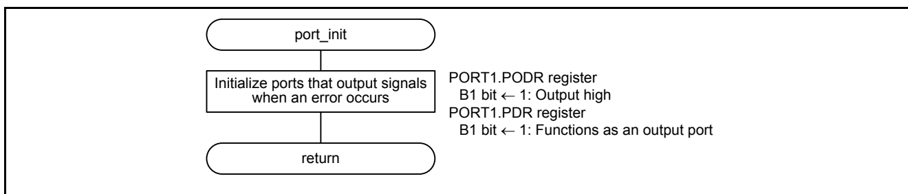
Figure 5.4 Port Initialization
