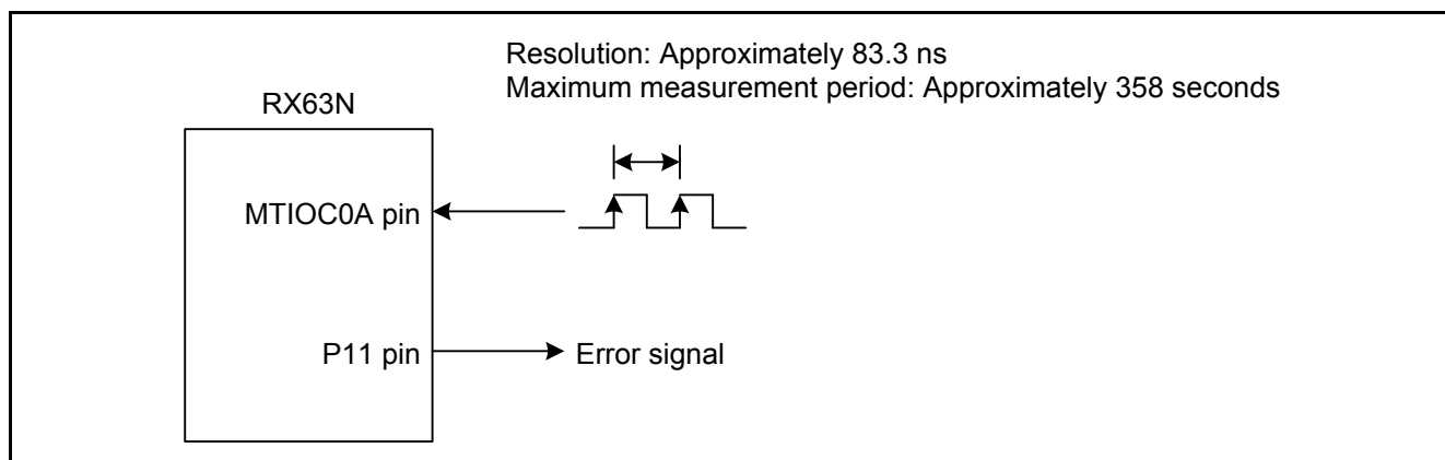
Figure 1.1 Connection Diagram
