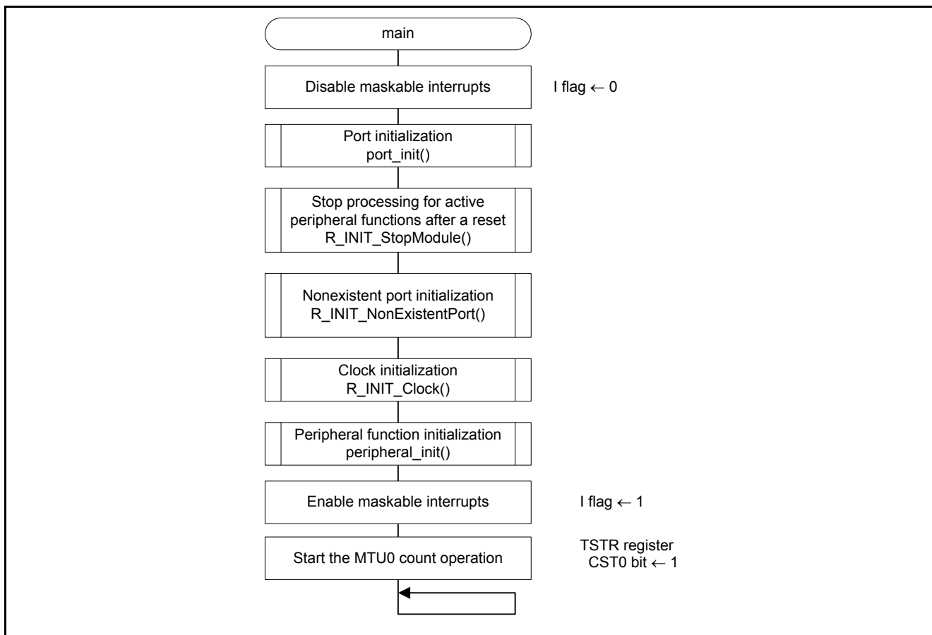
Figure 5.3 Main Processing
