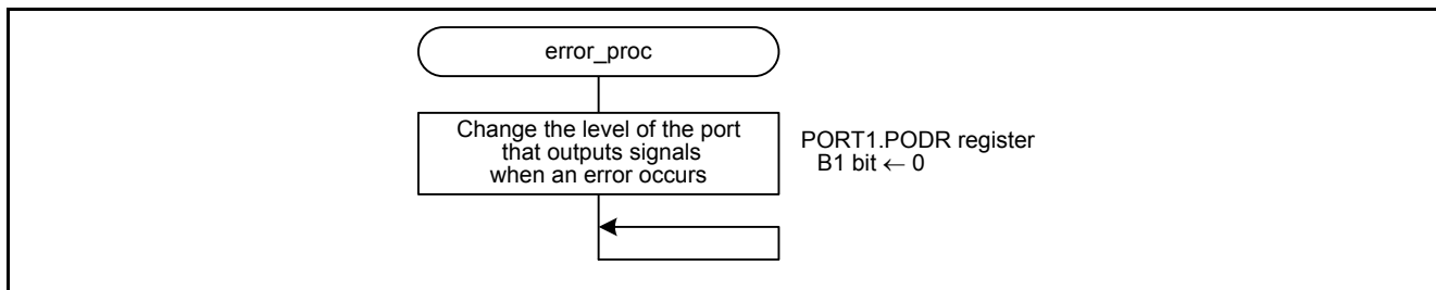
Figure 5.7 Error Processing
