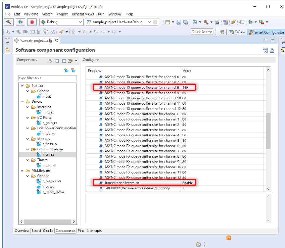
Figure 5-16 r_sci_rx Configuration (3)
