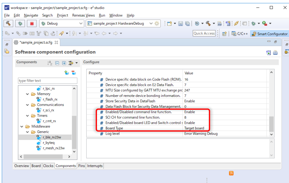
Figure 5-13 r_ble_rx23w Configuration (2)
