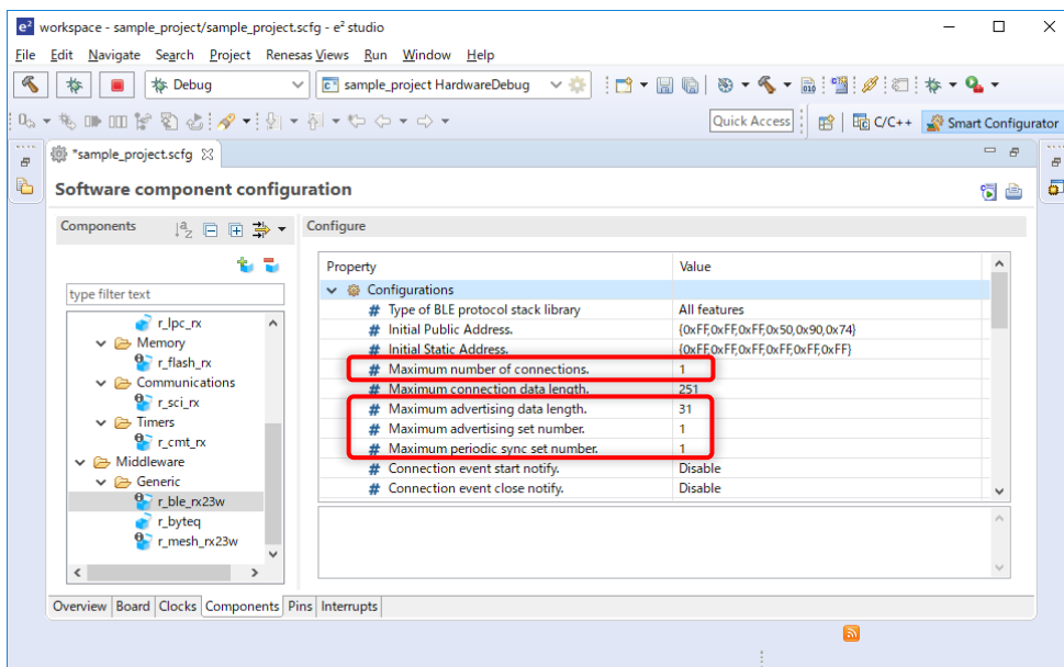
Figure 5-12 r_ble_rx23w Configuration (1)
