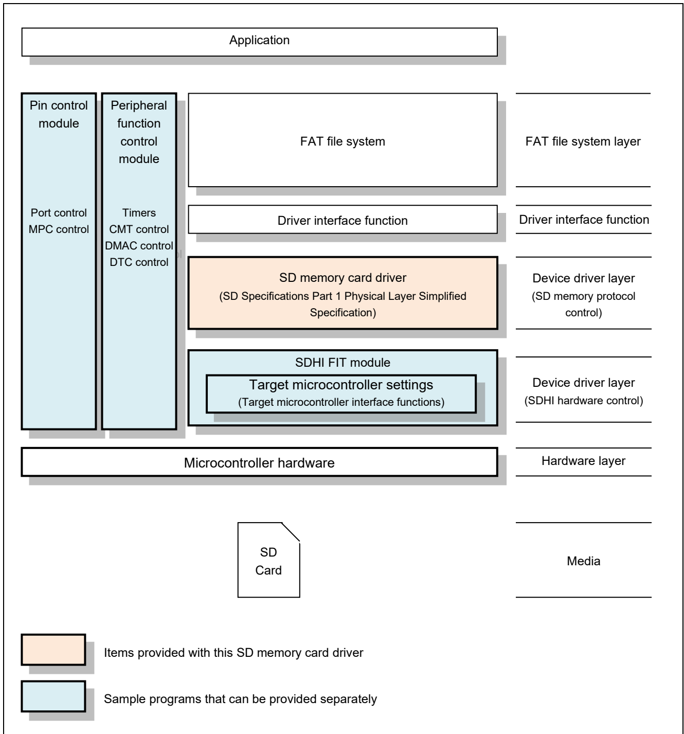
Figure 1.1 Application Structure
