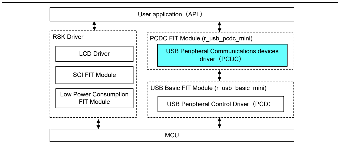
Figure 2-1 Module Configuration
