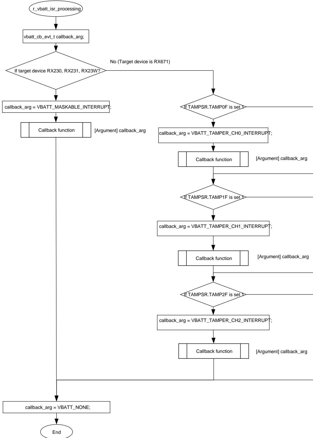
Figure 1.4 r_vbatt_isr() Function Flowchart
