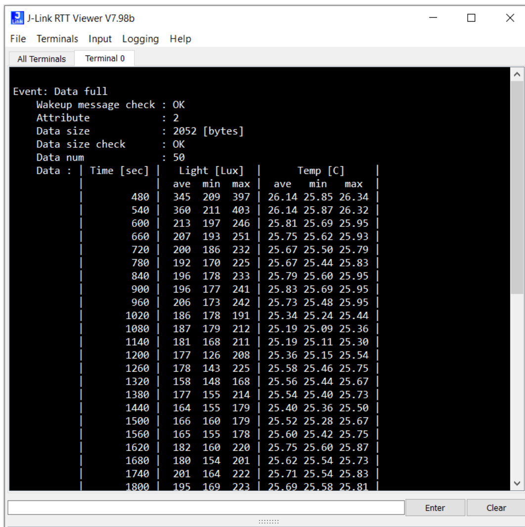
Figure 4.10. Example of data acquisition triggered by data full state
