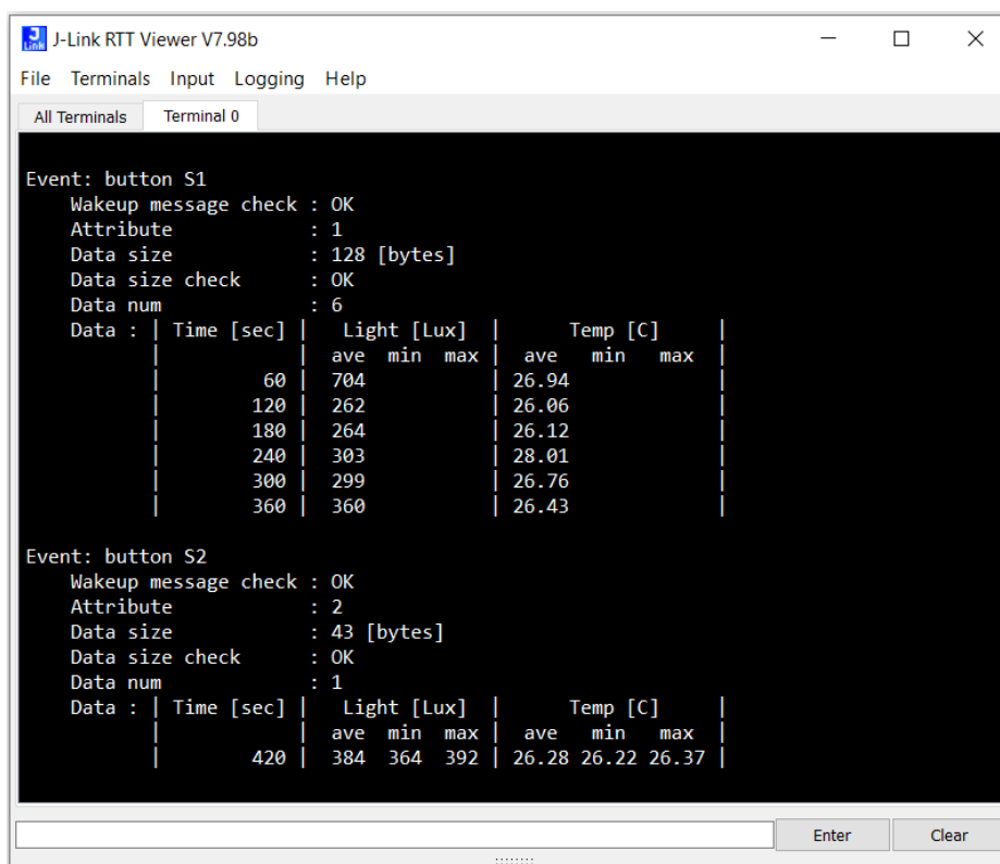
Figure 4.12. Example of data acquisition triggered by pressing the button on the main module
