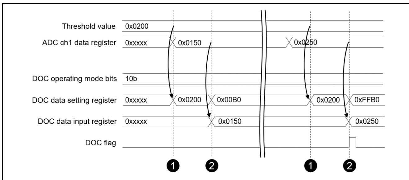
Figure 2.6. Level judgment using DOC subtraction mode
