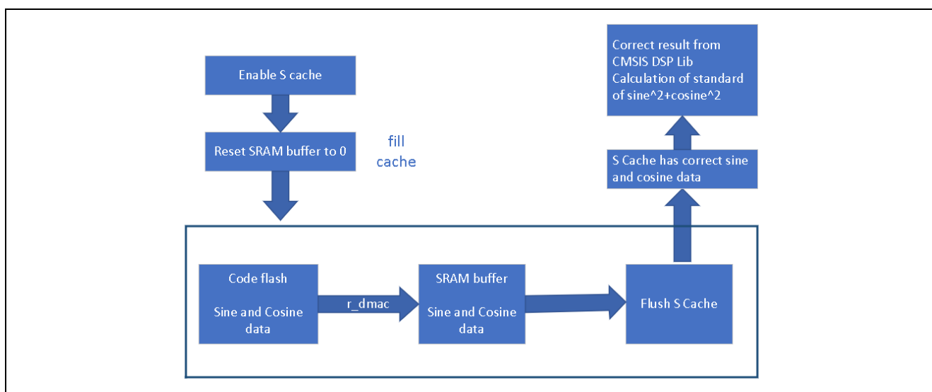
Figure 11. S Cache Coherency is Restored – Flush S Cache in Application Code
