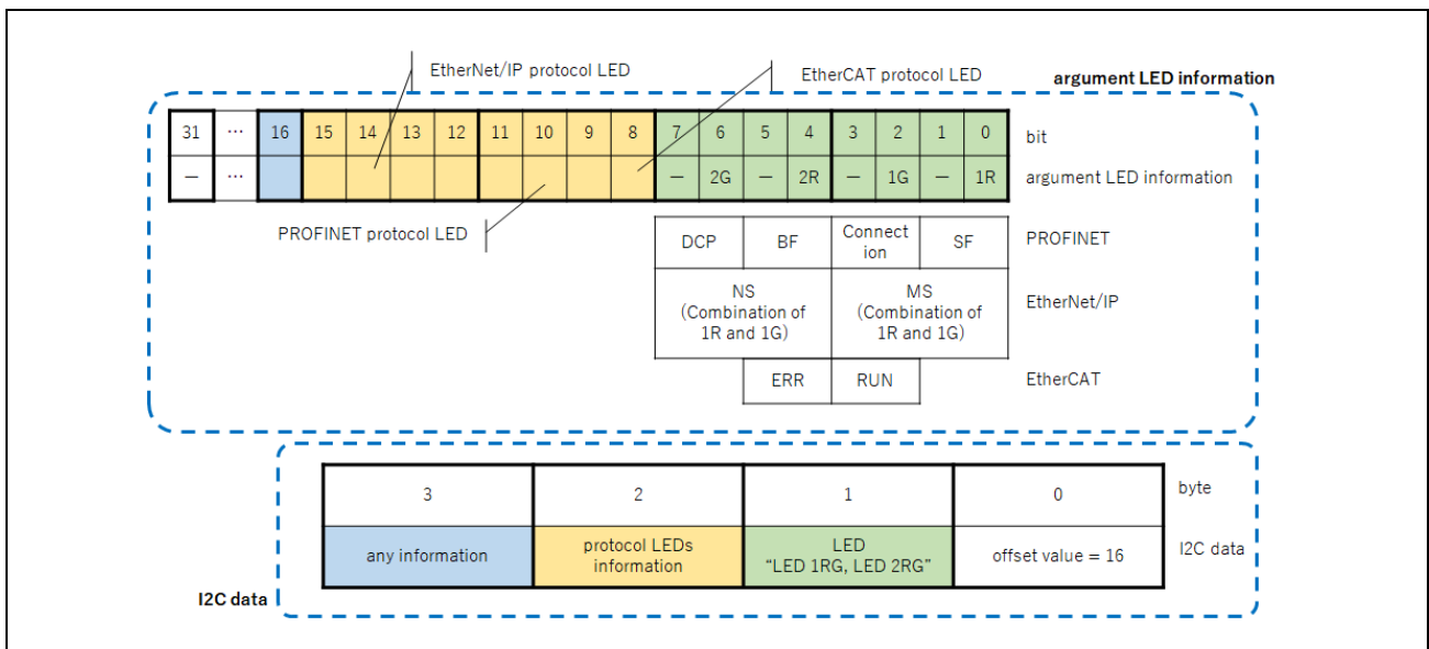
Figure 3-10 Relationship between argument information and I2C data
