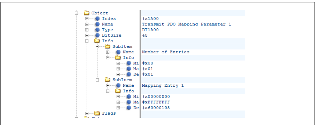
Figure 6-11 TxPDO Entry
