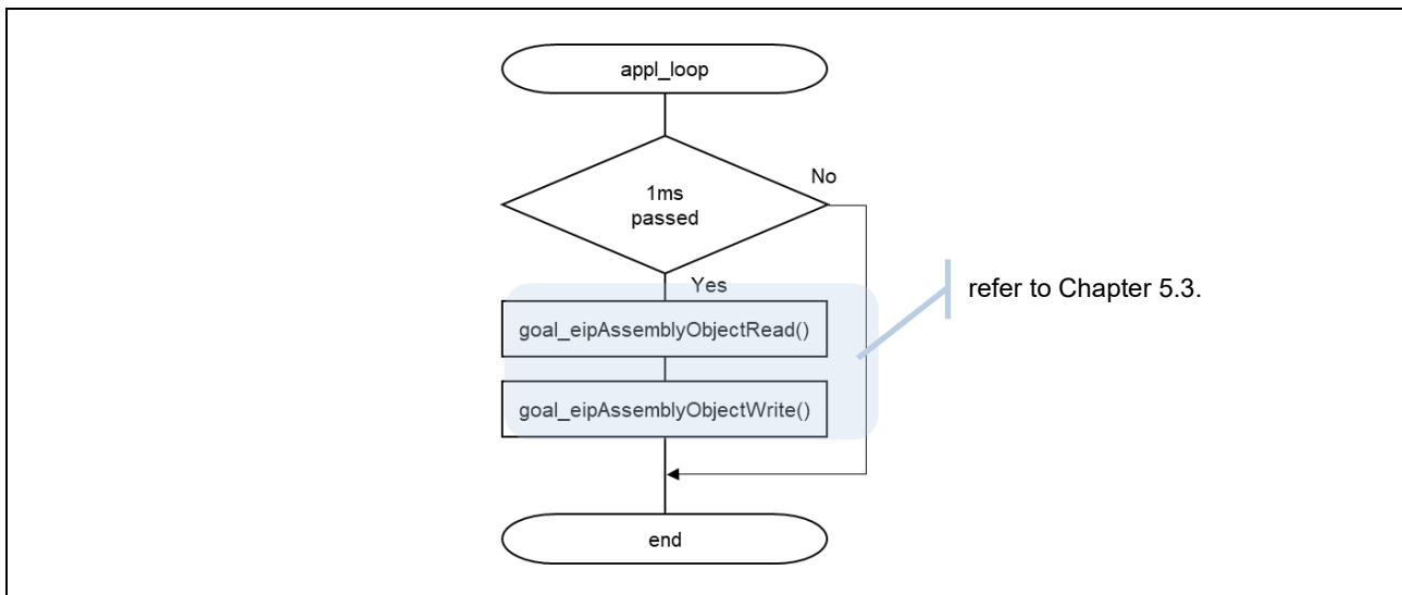
Figure 2-11 EtherNet/IP appl_loop() flow
