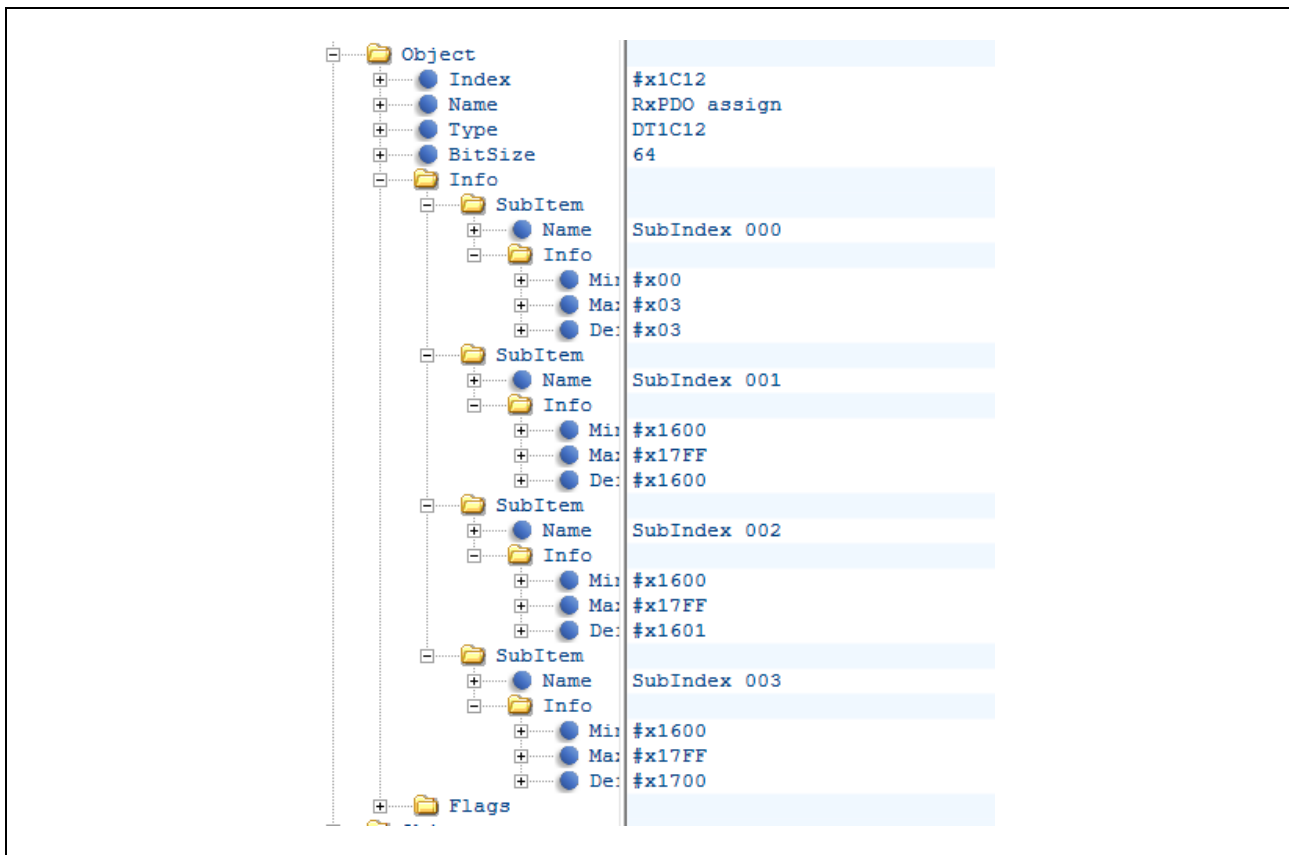
Figure 6-8 Set Object [0x1C12]
