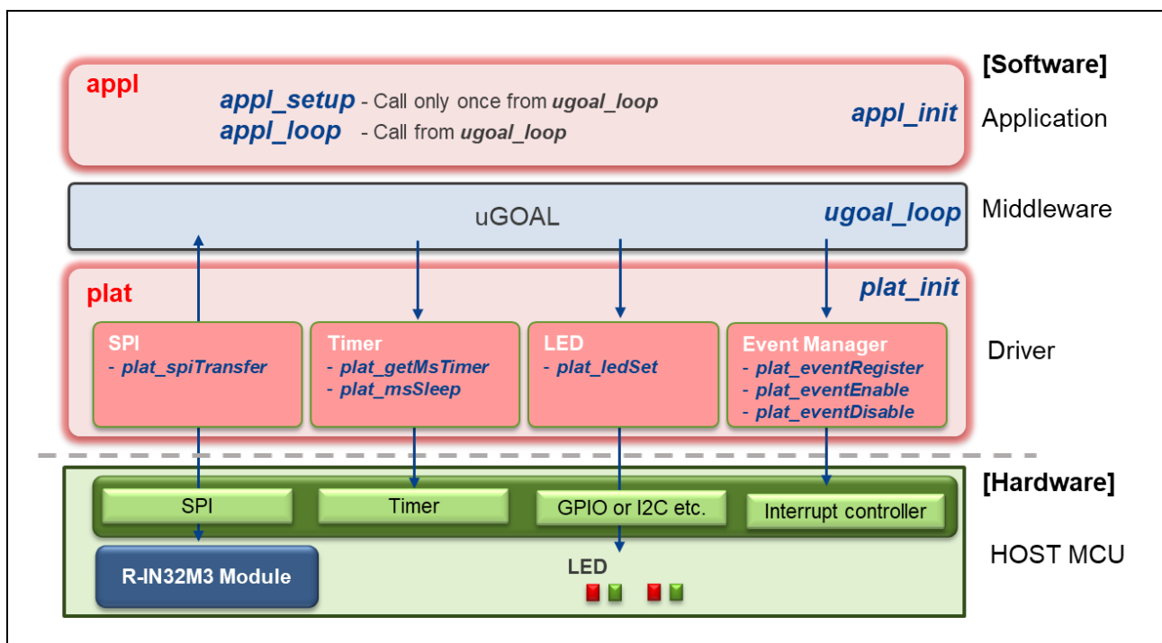
Figure 2-2 software structure
