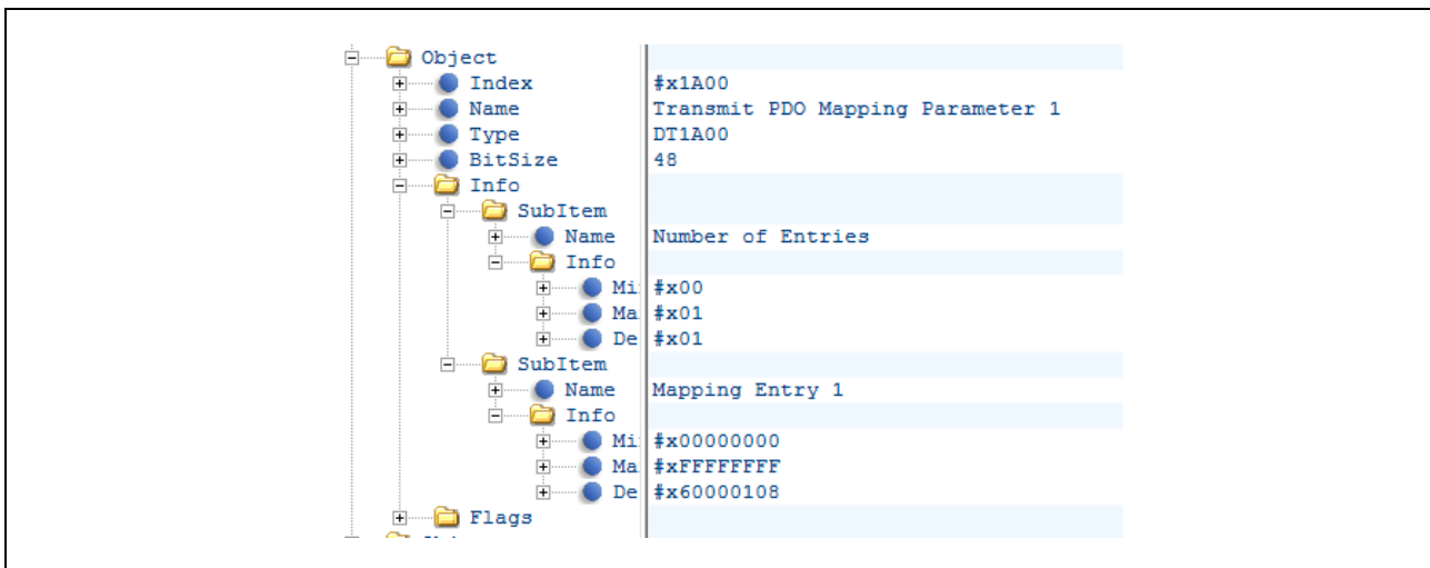
Figure 6-11 TxPDO Entry
