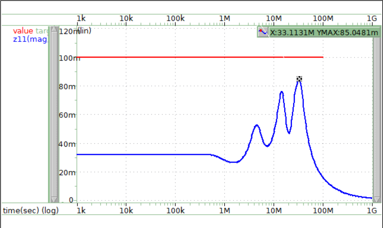
Figure 4.2 Target impedance of core power supply and impedance data of 13mm RZ/G2LC
