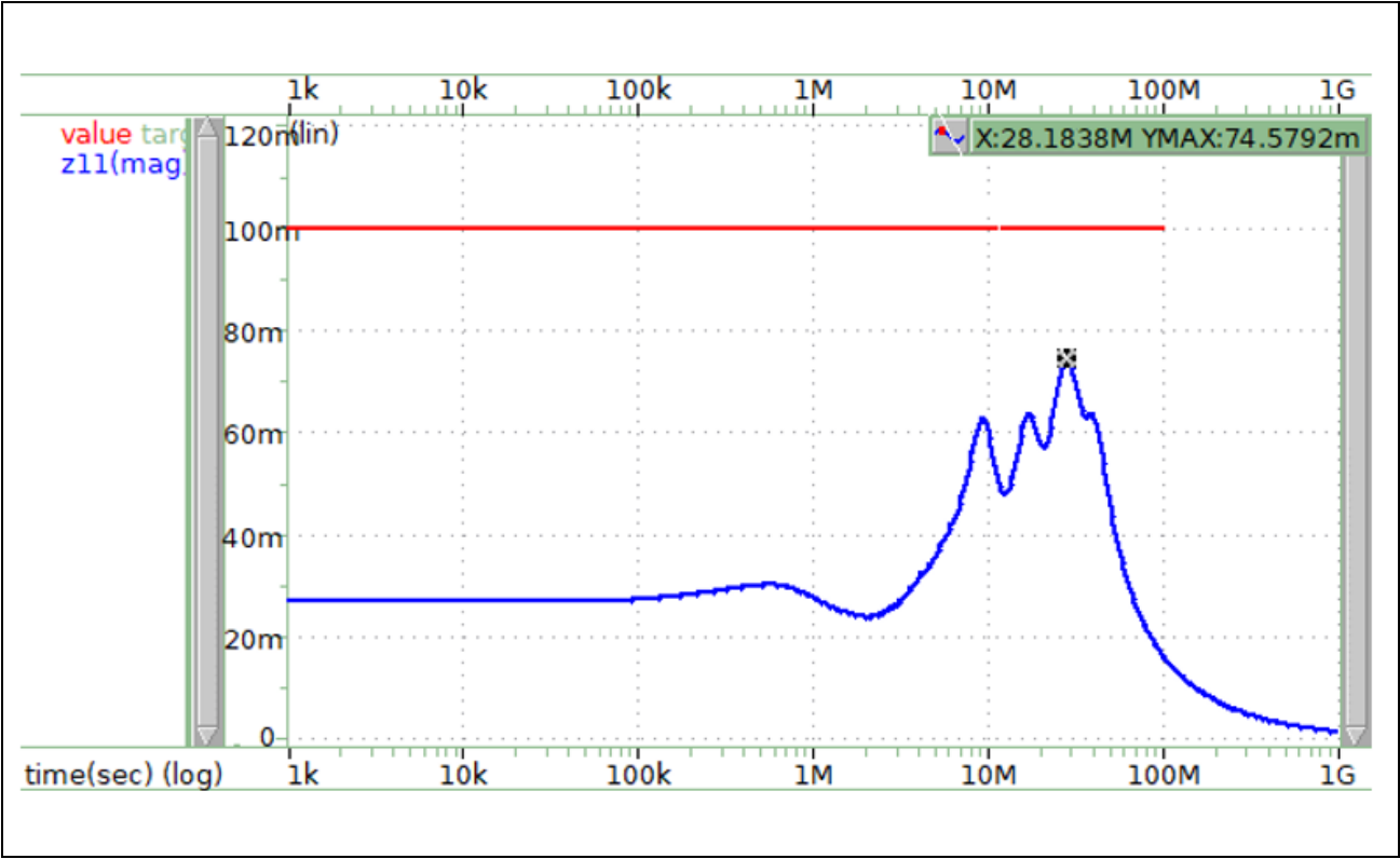
Figure 4.3 Target impedance of core power supply and impedance data of 15mm RZ/G2L
