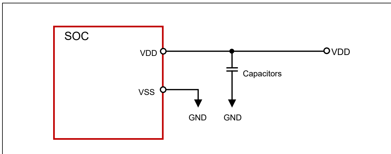
Figure 3.1 Circuit diagram of Core power supply (VDD) and external parts
