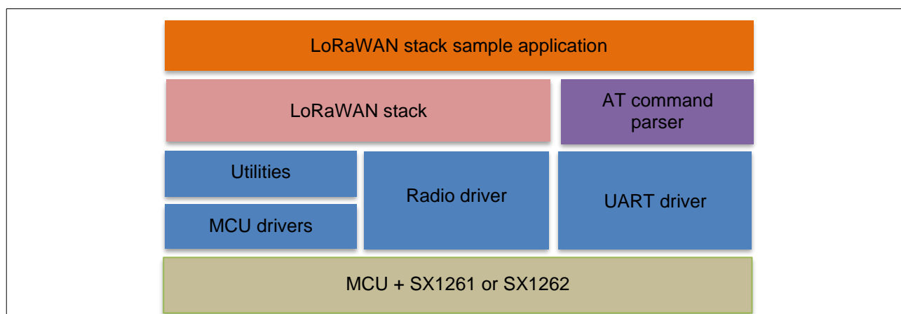
Figure 2. Sample Application Block Diagram
