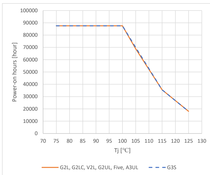
Figure 1.1 Lifetime Estimation vs T_j
