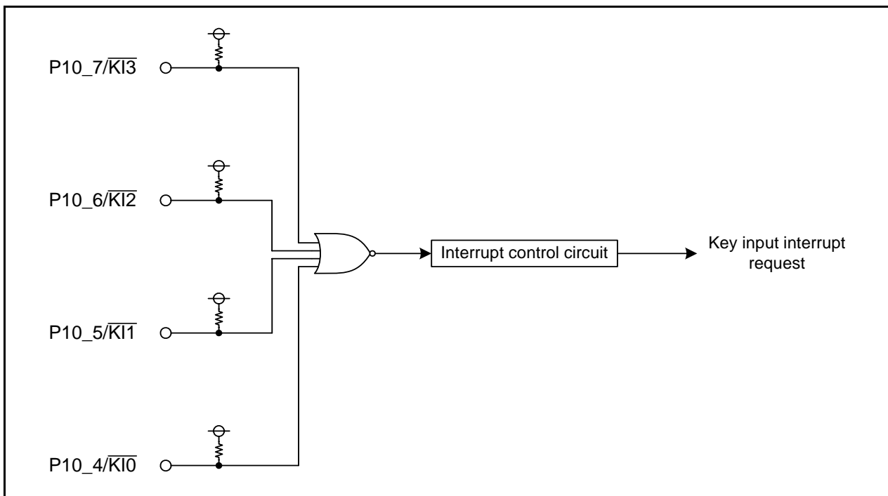
Figure 4.1 Key Input Interrupt Block Diagram
