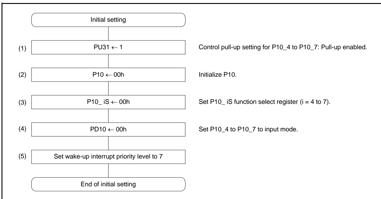
Figure 4.3 Initial Setting Flowchart
