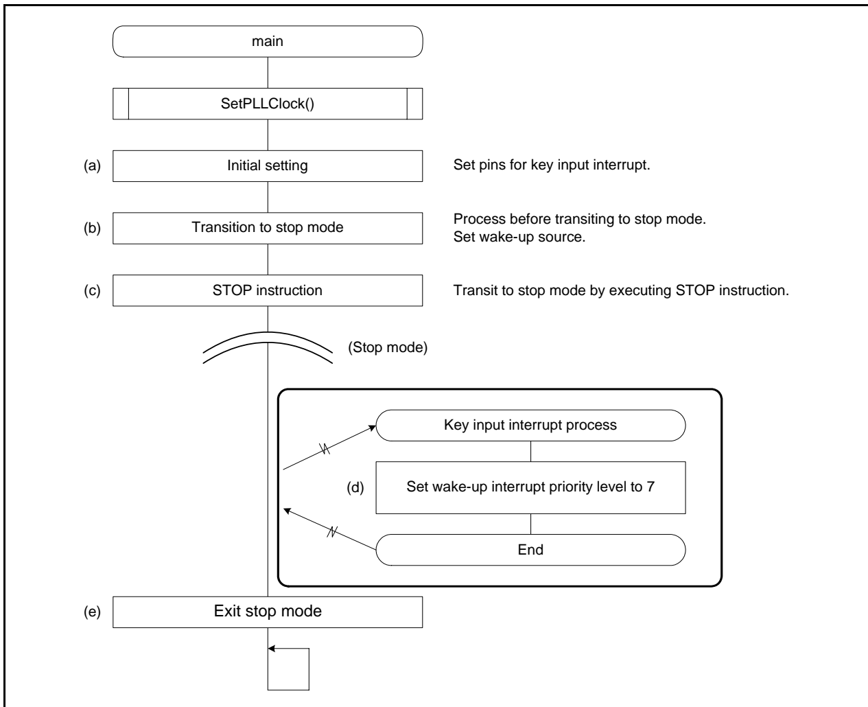
Figure 4.2 Main Function Flowchart
