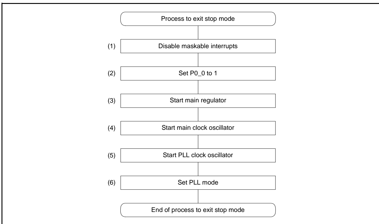
Figure 4.5 Exit Stop Mode Flowchart
