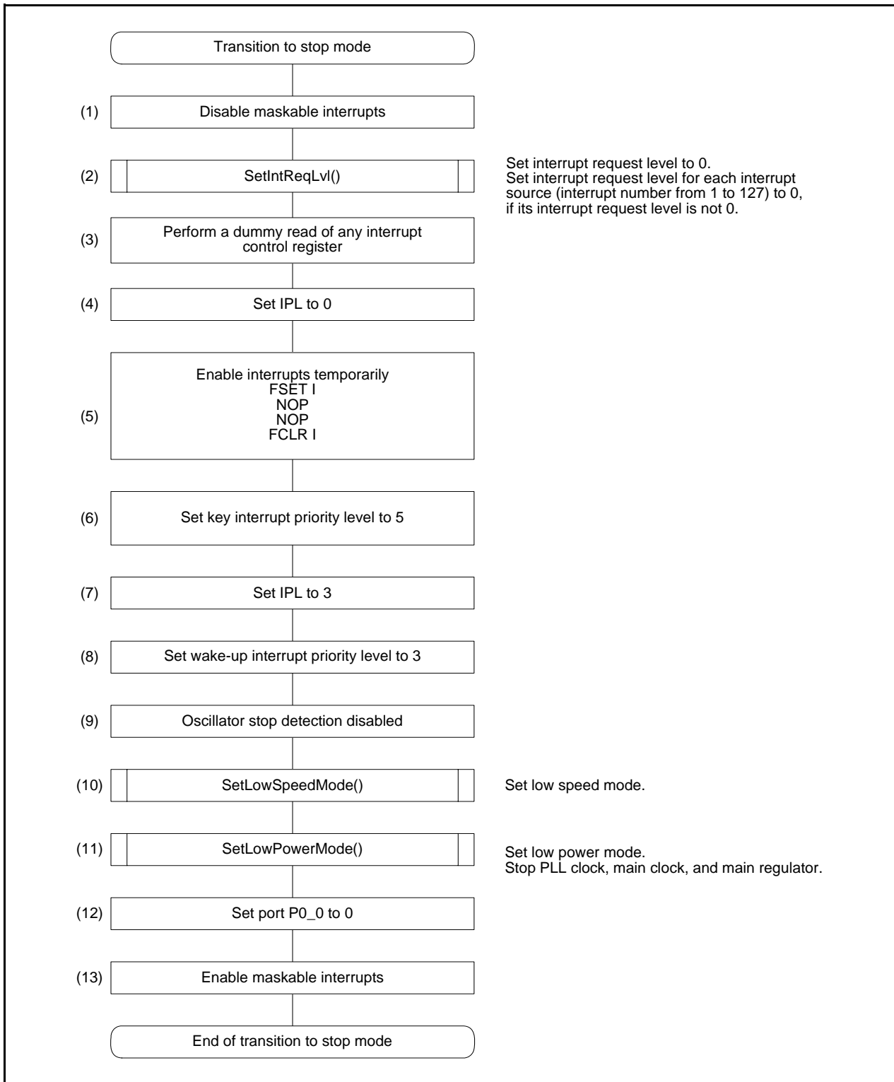
Figure 4.4 Transition to Stop Mode Flowchart
