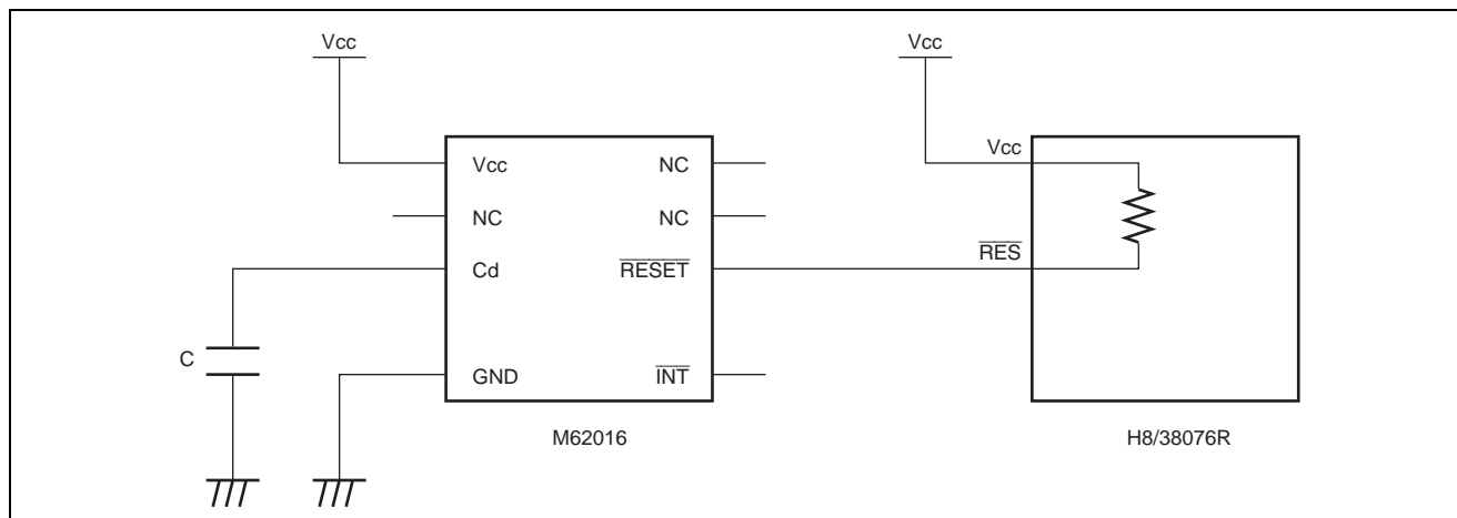
Figure 1 Power-On Reset Operation Using Reset IC
