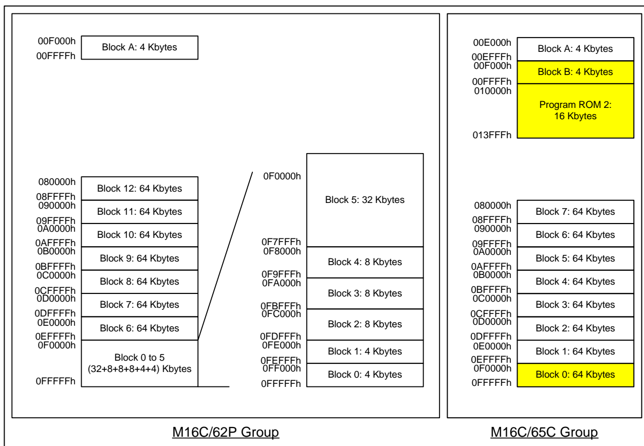
Figure 2.1 Differences in Flash Memory Block Configuration
