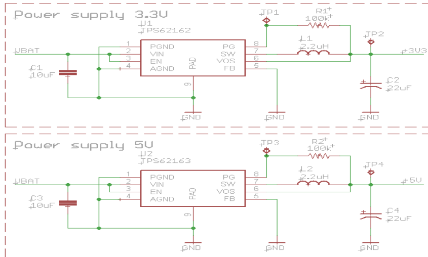
Figure 21: Supply Schematic
