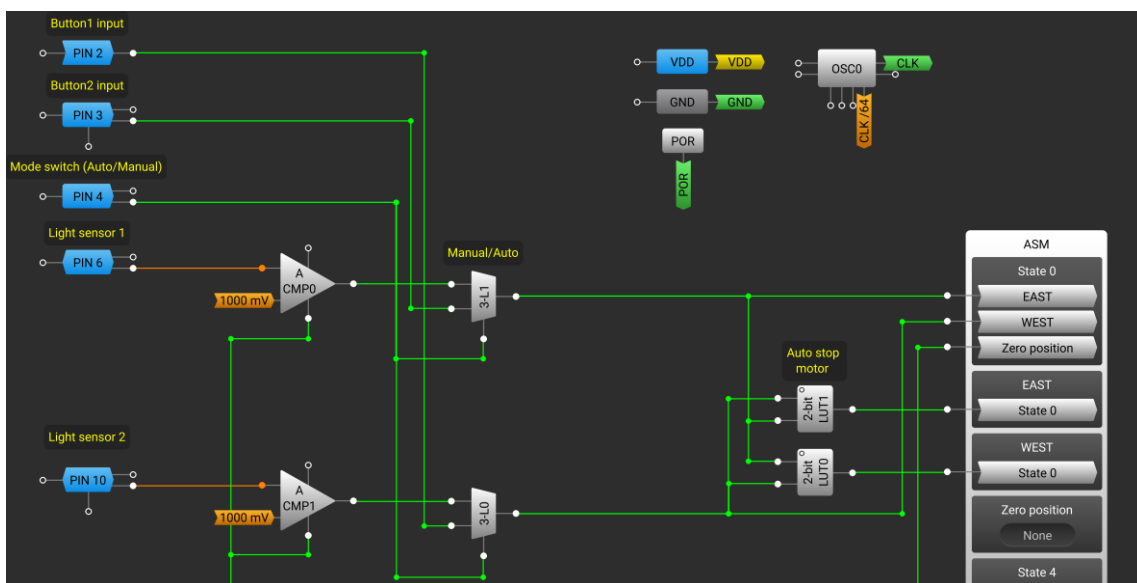
Figure 4. Mode and LDR Inputs to ASM
