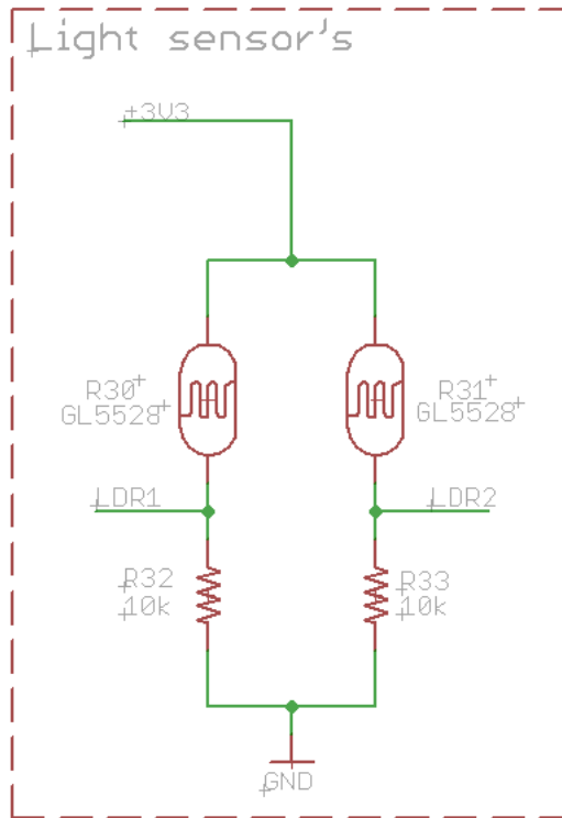
Figure 3. LDR Sensor
