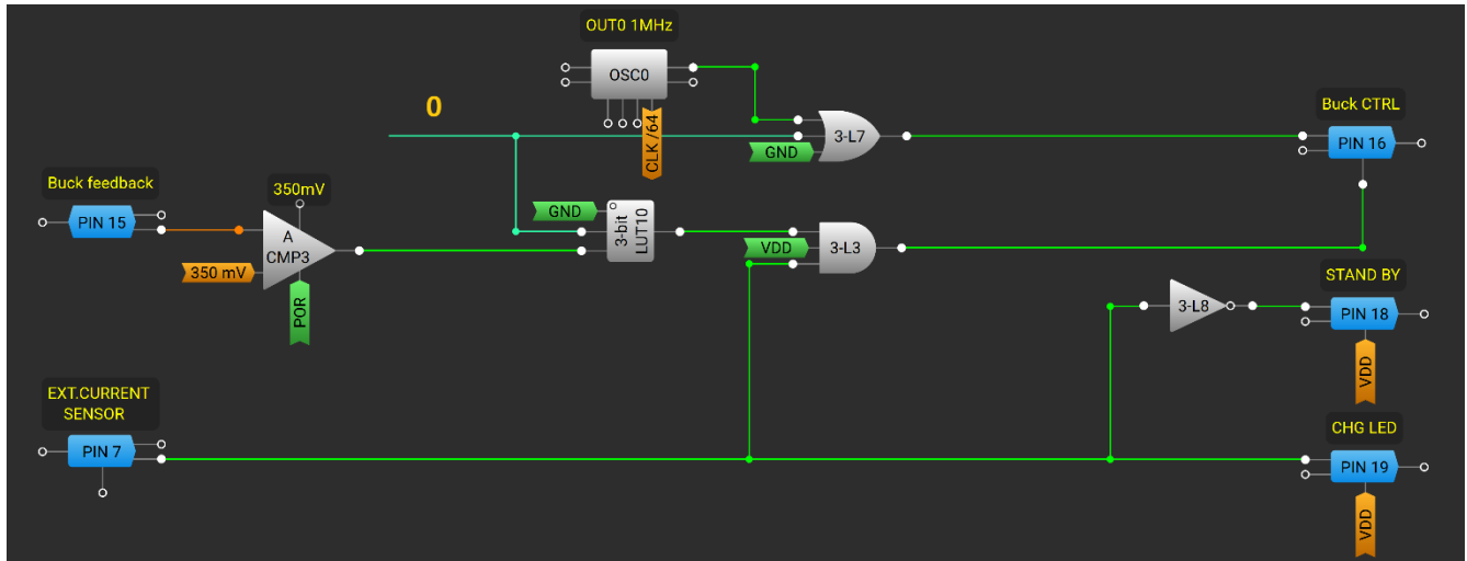
Figure 17. Buck Regulator Charging Logic
