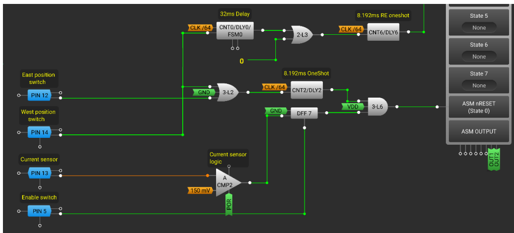
Figure 8. Motor Limit and Overload Protection
