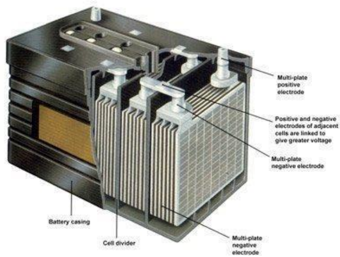
Figure 22. Lead Acid Battery
