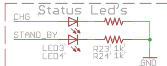
Figure 20. Battery Charge Status LEDs are Connected on PIN18 and PIN19
