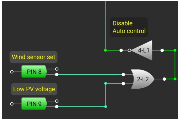
Figure 13. Wind Fault Control
