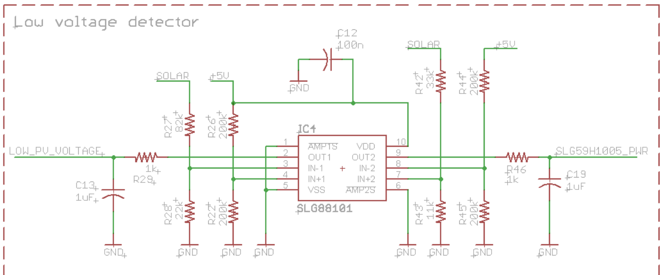
Figure 12. Low Voltage Detector Circuit
