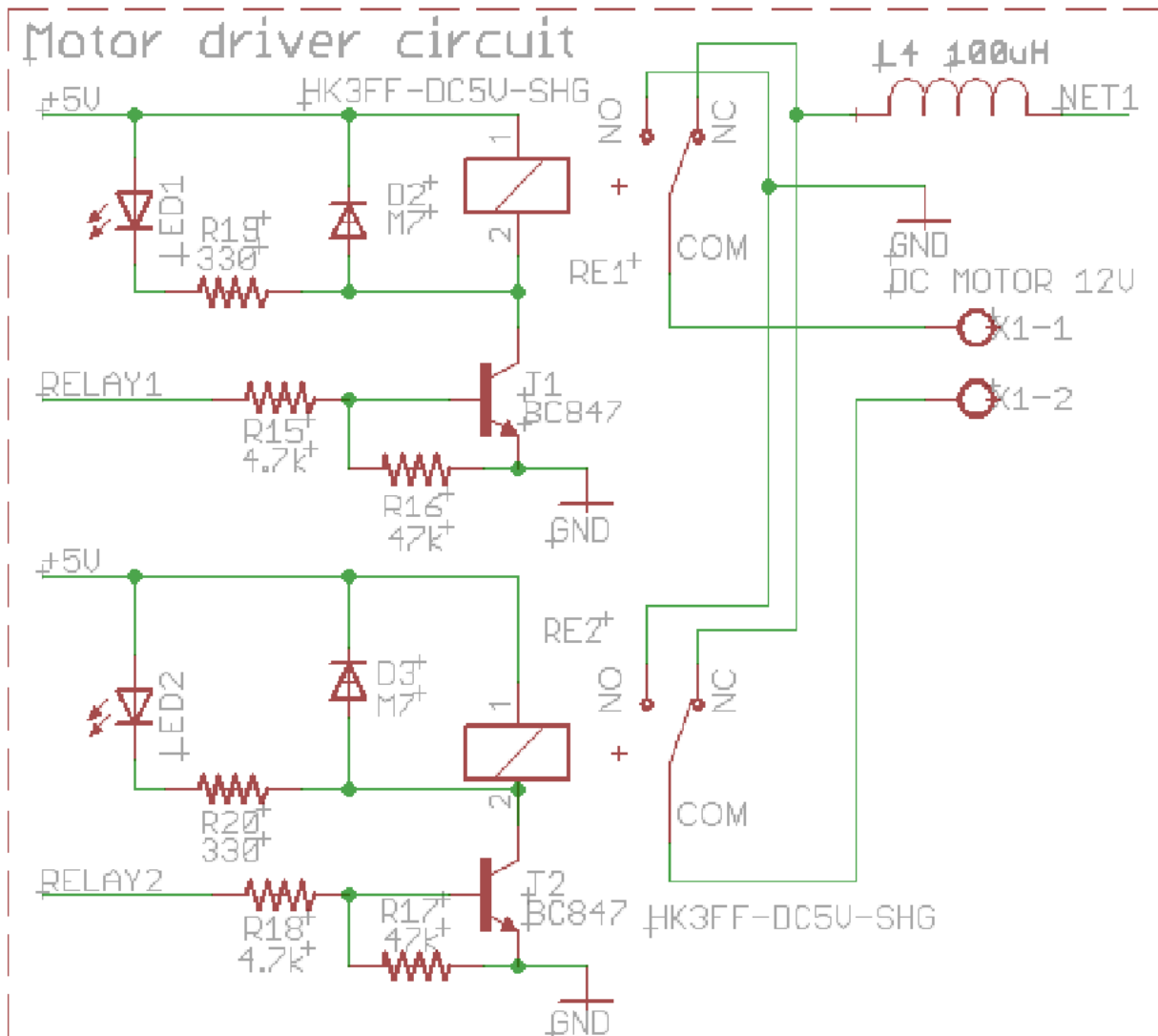
Figure 9. Motor Driver Circuit
