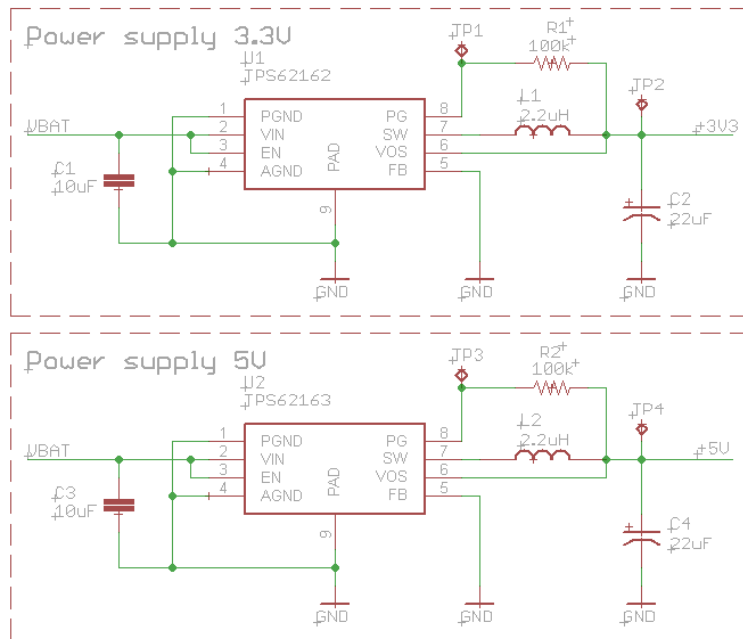
Figure 21. Supply Schematic
