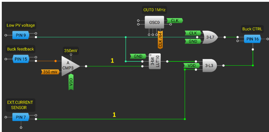
Figure 14. Low Voltage Control
