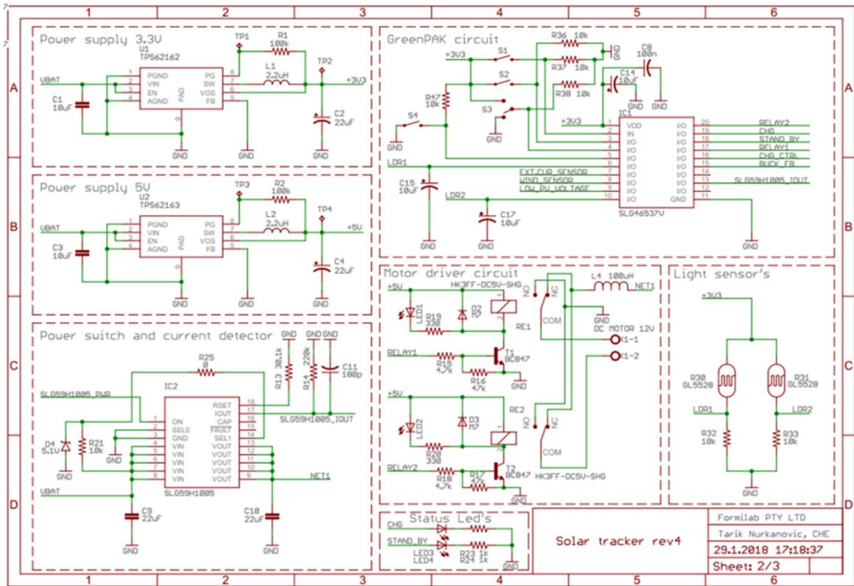
Figure 23. Electrical Schematic Part 1
