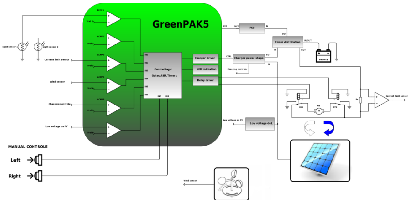
Figure 1. Top Level Schematic
