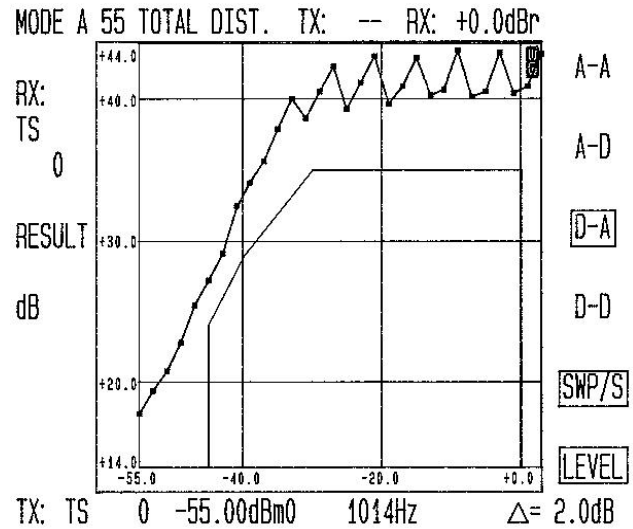
FIGURE 14. (D/A) TOTAL DISTORTION
