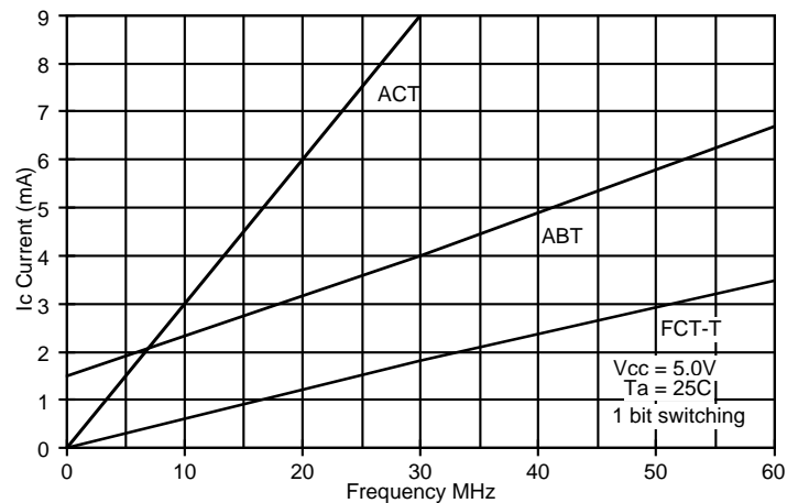
Figure 34, I_c vs. Frequency
