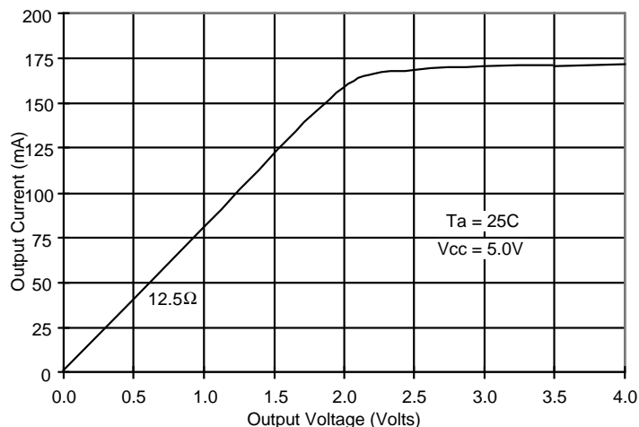
Figure 9, Vol Characteristics of Balanced Drive
