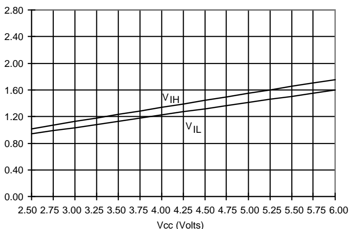
Figure 2, Input Threshold Voltage ( V_{IH}/V_{IL} )
