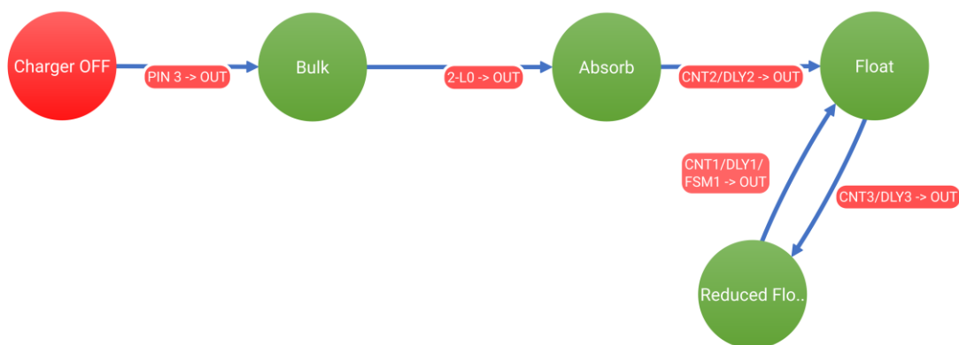
Figure 1. The Battery State Machine
