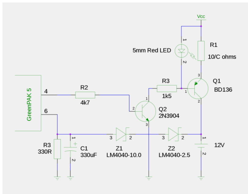
Figure 3. External Components Used
