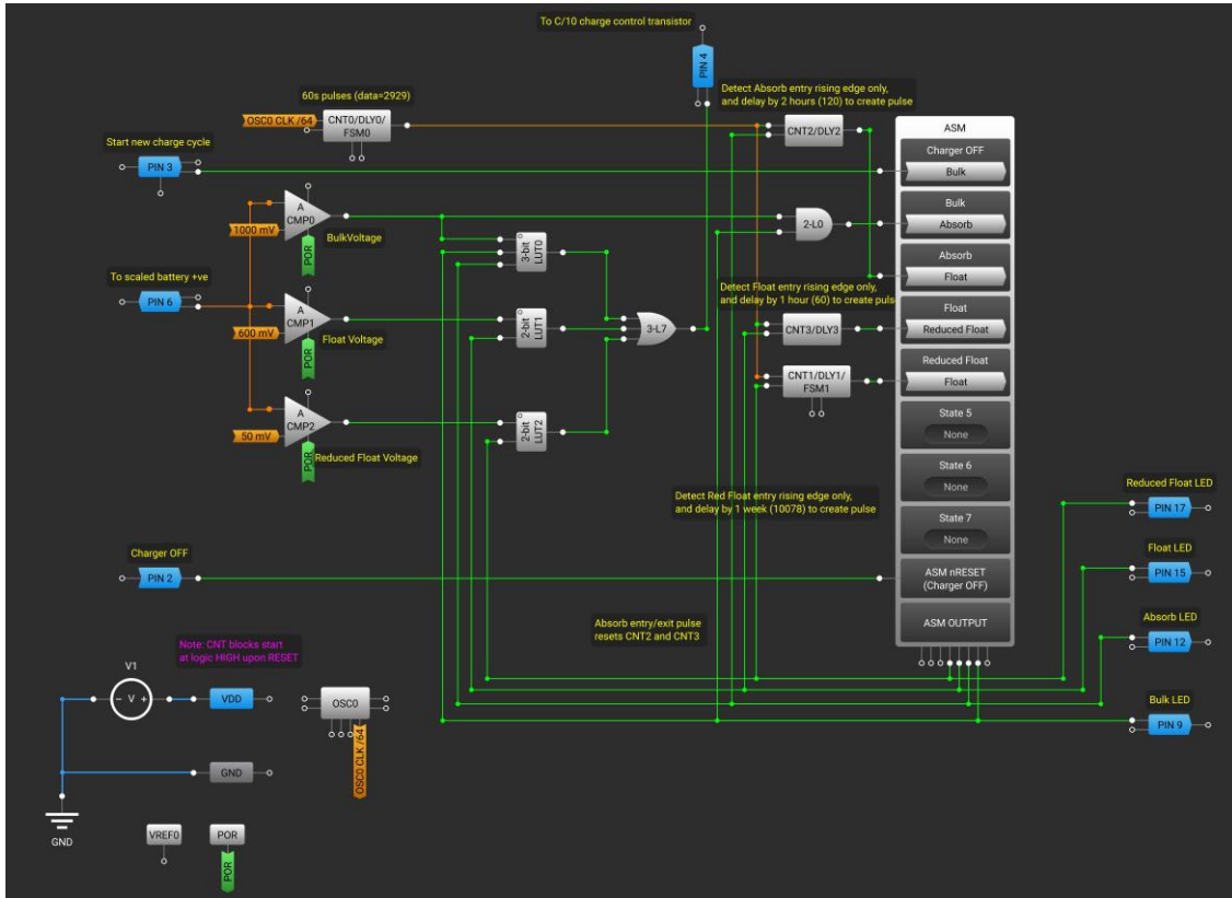
Figure 2. The GreenPAK Design
