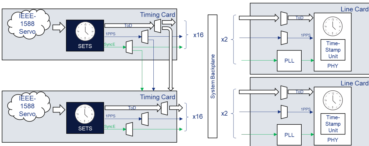
Figure 2. System ToD Infrastructure Diagram for Class C or D Compliance
